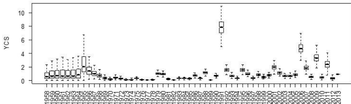
Figure 7: Distribution of YCS posteriors for the Equilibrium Age Prop0.70 model (run 4.1). Bold lines and boxes are the median and lower/upper quantiles; whiskers extend to the most extreme data point that is not more than 1.5 times the interquartile range from the box.
