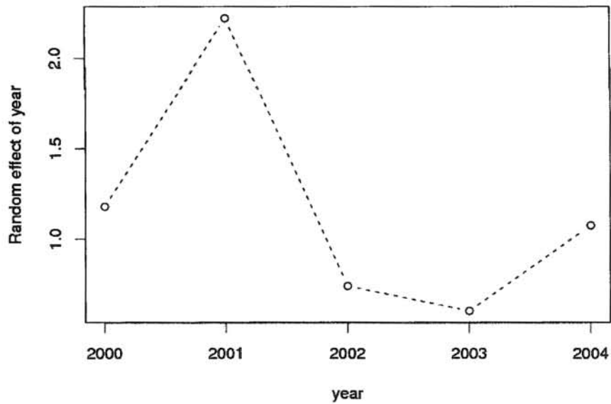
Figure 14: The year random effects. Catch rates are predicted to have been higher in 2001 than can be explained by the fixed effects alone.
