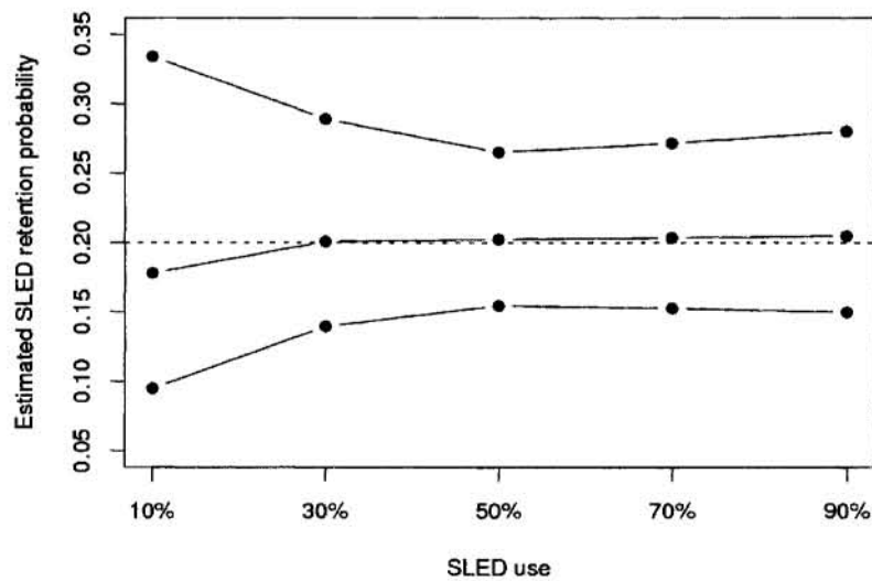
Figure 16: The model estimated SLED retention probability (mean and 95% c.i.), as a function of the assumed level of SLED coverage.
