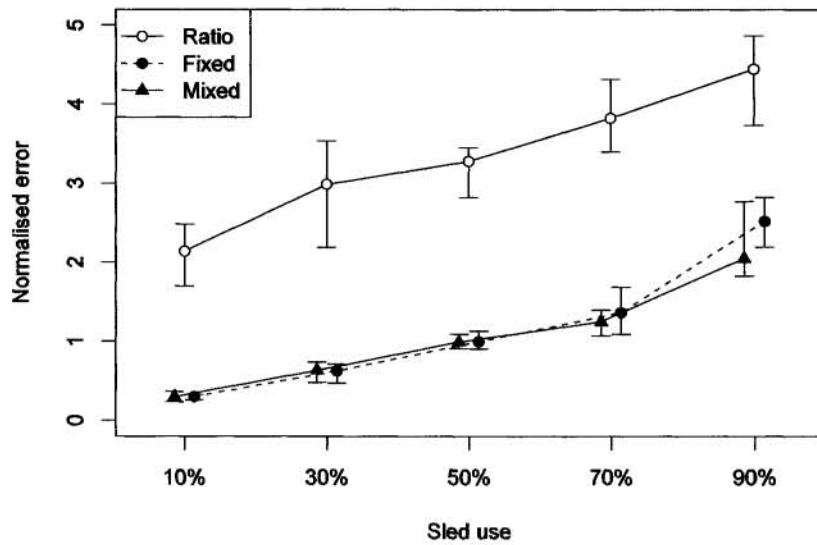
Figure 15: Comparing the models' ability to recover the test data. The test data are a simulation of the 2000 to 2004 data, with varying levels of SLED use. The y-axis shows the mean and range of the normalised error (predicted total – actual total)/sqrt(actual total), where the data are grouped by SLED coverage and by year. The three lines are for the ratio estimate, and the models with fixed and with mixed effects.
