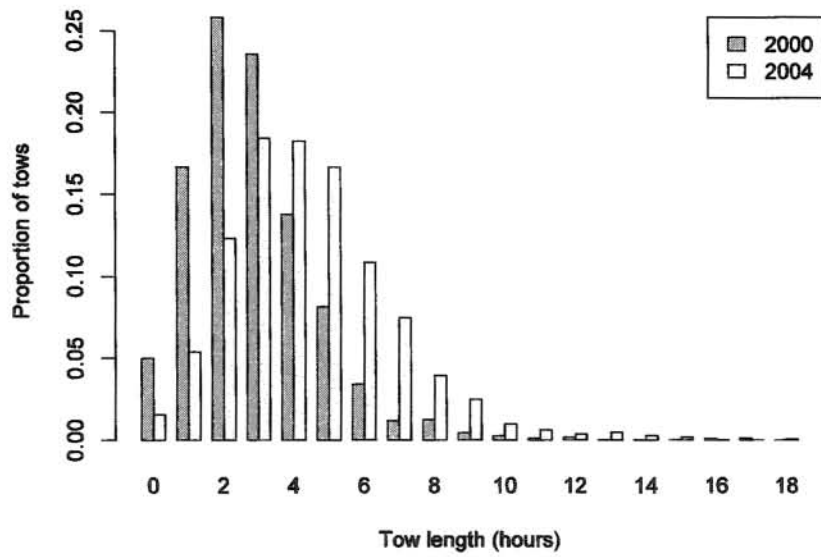
Figure 13: Change in distribution of tow length between 2000 and 2004, from the catch effort data.
