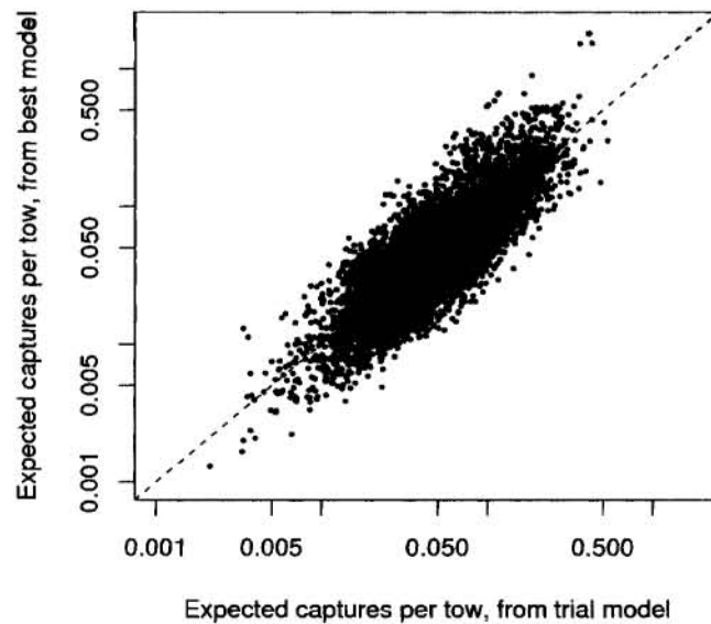
Figure 8: Comparison between the best and the trial models. The predictions of the best and the trial models, from the catch-effort data, are shown against one another.
