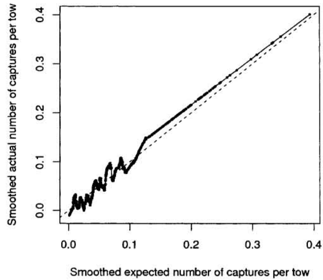
Figure 7: Smoothed model predictions. The actual captures are compared with the predictions from the best model, with the data being jointly smoothed. The 1:1 relationship is shown by the dashed line.
