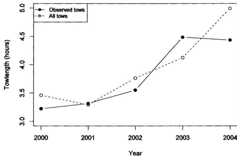
Figure 12: Changes in the tow length over the five years. The two lines show the mean tow length from the observer tows only (as recorded in the observer data) and the mean tow length from all tows (as recorded in the catch effort data). Both datasets show an increase in the mean tow length over the five year period.
