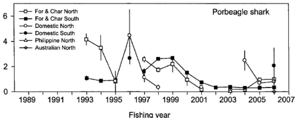
Figure 1: Unstandardised CPUE indices (number of sharks per 1000 hooks) for the tuna longline fishery based on observer reports. Years are fishing years (1993 = October 1992 to September 1993). Confidence intervals are from bootstrapped data. Source: Griggs et al. (2008).
