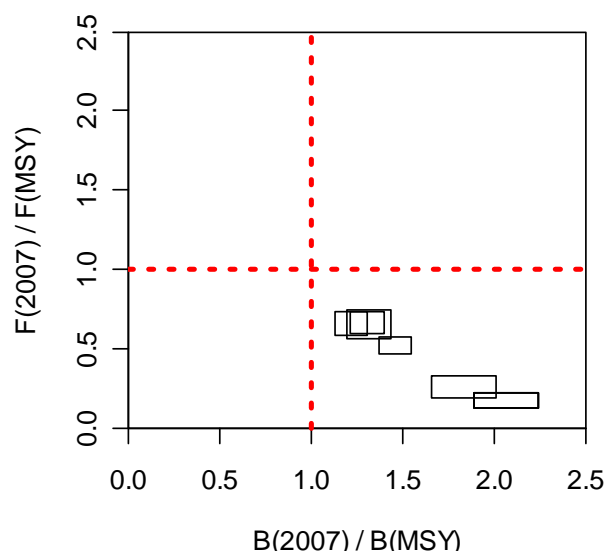
Figure 1: Summary plot comparing South-West Pacific fishing mortality, F(2007)/F(MSY) , and total stock biomass, TSB(2007)/TSB(MSY) , for Southwest Pacific swordfish from a subset of plausible MULTIFAN-CL models. Boxes indicate the upper and lower 95% confidence limits (but not the covariance) for each individual model.
