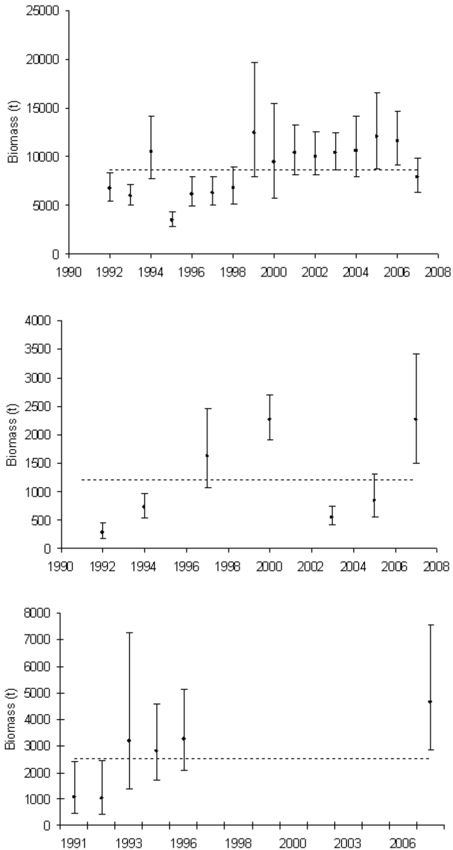
Figure 2: Biomass trends \pm 95\% CI (estimated from survey CV's assuming a lognormal distribution) and the time series mean (dotted line) from the Chatham rise (top), West (middle) and East (bottom) Coast South Island trawl surveys.
