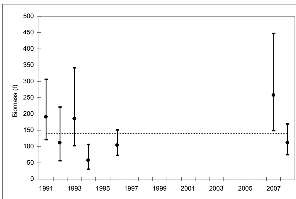
Figure 2: Biomass estimates \pm 95\% CI (estimated from survey CV's assuming a lognormal distribution) and the time series mean (dotted line) from the East Coast South Island trawl survey.
