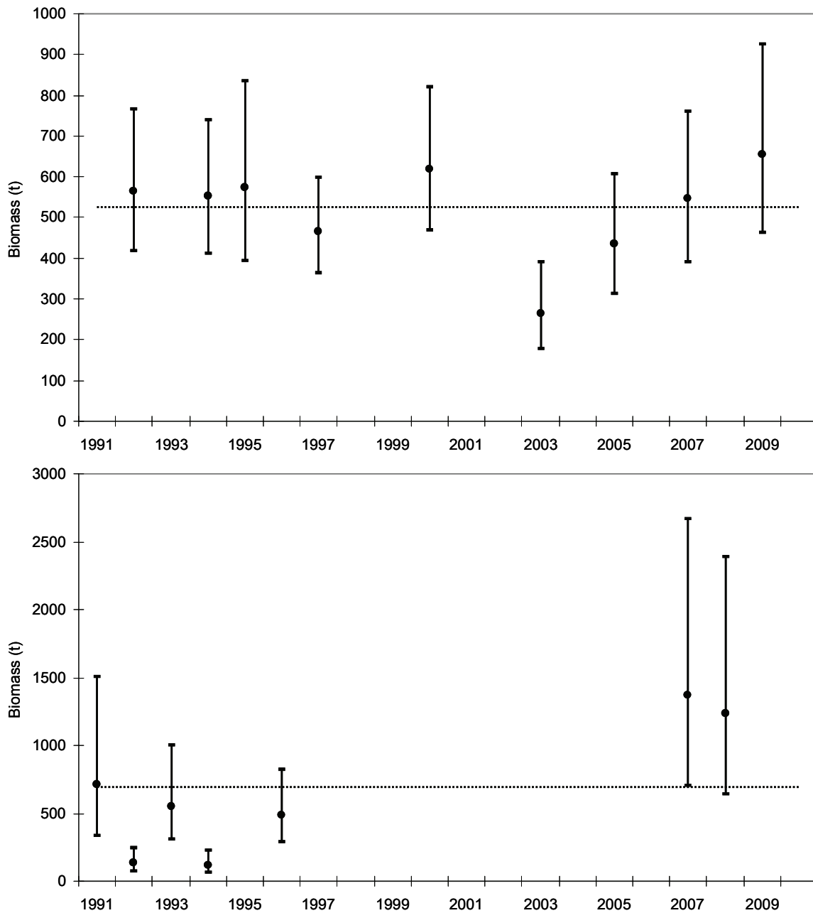
Figure 5: Biomass trends \pm 95% CI (estimated from survey CV's assuming a lognormal distribution) and the time series mean (dotted line) from the West (top) and East (bottom) Coast South Island trawl surveys.
