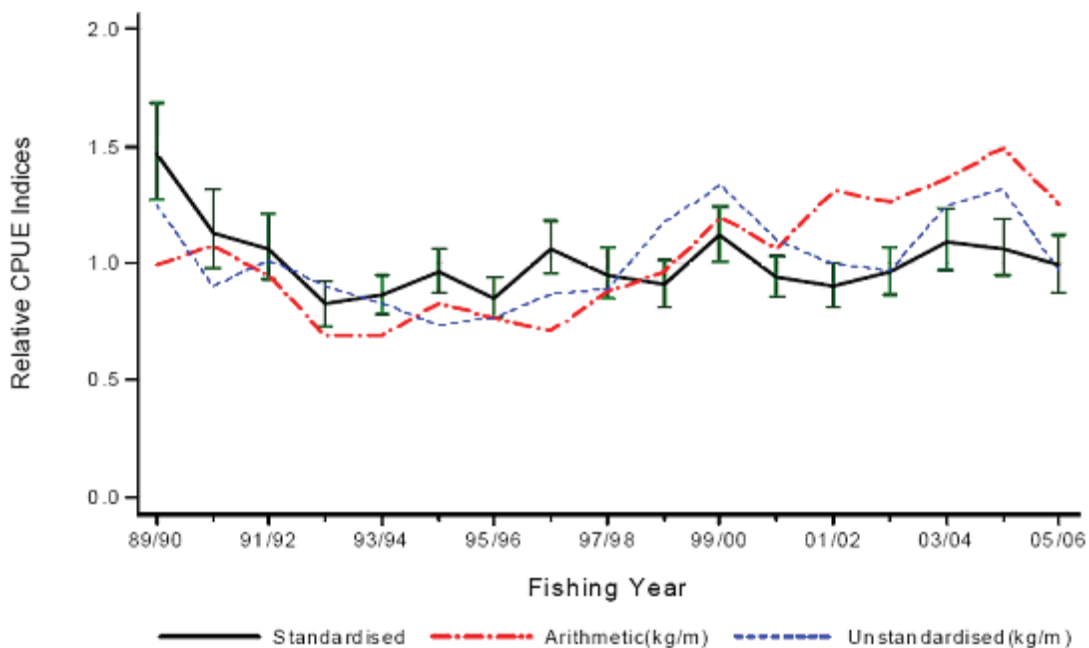
Figure 3: Relative CPUE indices for SCH 3 using the lognormal non-zero model based on the shark setnet fishery. Error bars are \pm 2*SE . Also shown are two unstandardised series from the same data. [Continued on next page]...
