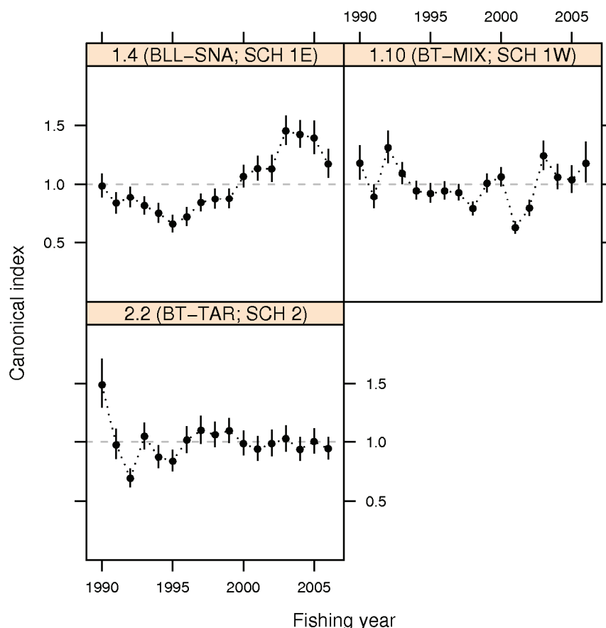
Figure 2: Canonical CPUE indices with 95% confidence intervals for the two SCH 1 CPUE series (top) and one SCH 2 CPUE series (bottom).
