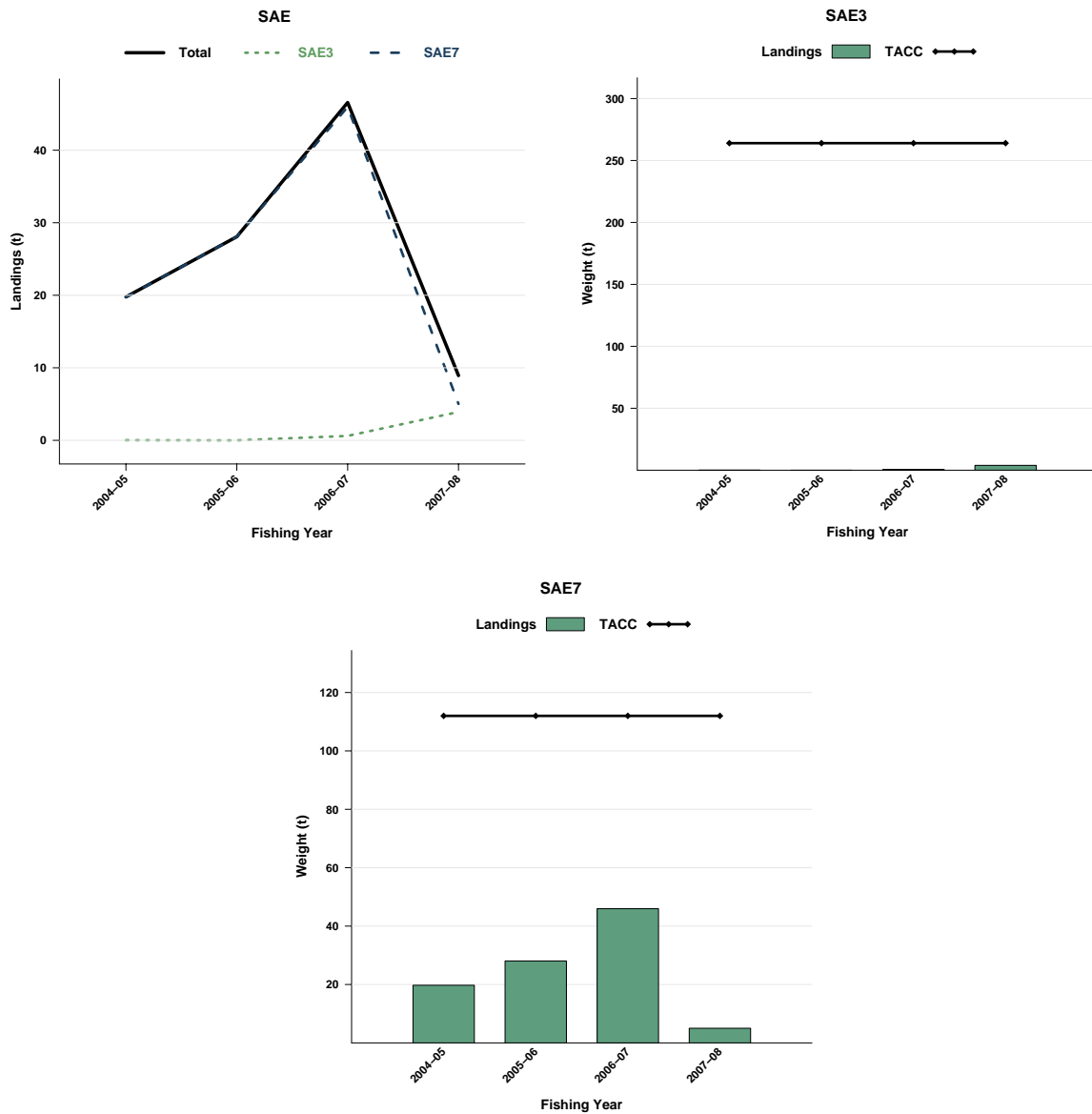
Figure 1: Top Left: Landings and the sum total (solid line) of the two main SAE stocks throughout time. From Top Right: Historical landings and TACC for SAE3 (South East Coast), and SAE7 (Challenger). Note that these figures do not show data prior to entry into the QMS.
