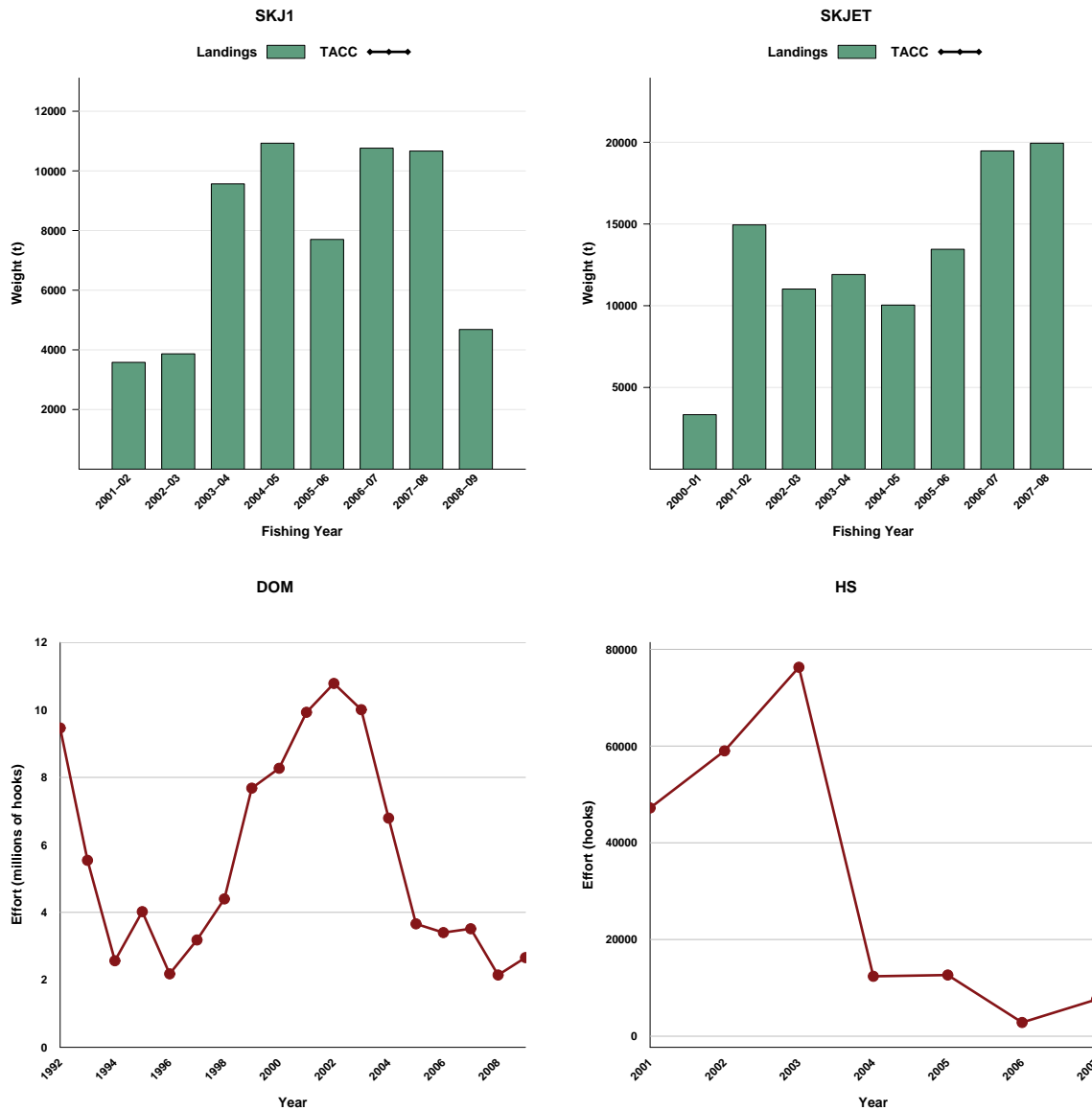
Figure 1: [Top] Skipjack catch from 2001-02 to 2008-09 within NZ waters (SKJ1), and 2000-01 to 2007-08 on the high seas (SKJET). [Bottom] Fishing effort (number of hooks set) for all domestic and high seas surface longline vessels, from 1992 to 2009 and 2001 to 2007, respectively.
