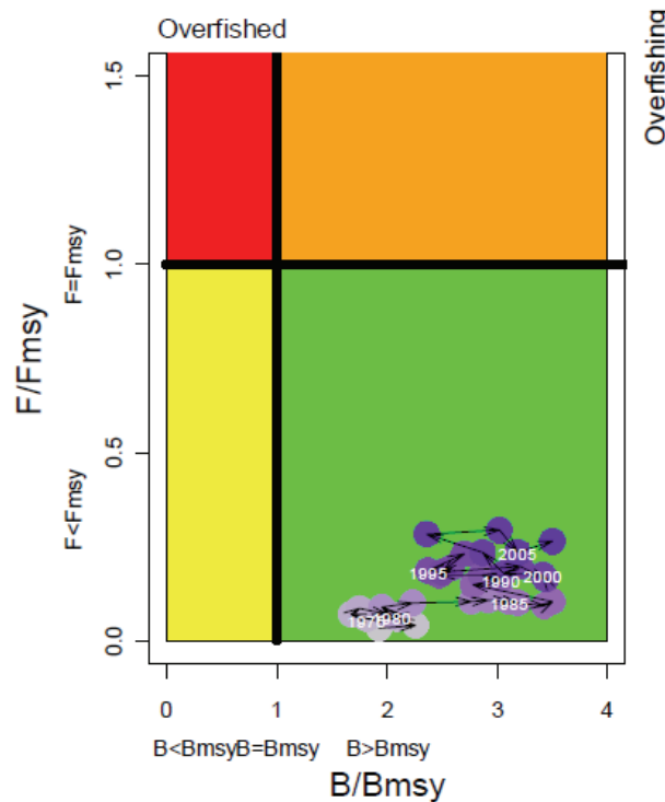
Temporal trend in annual stock status for skipjack tuna, relative to B_{MSY} (x-axis) and F_{MSY} (y-axis) reference points, for the model period (1972–2006) from the equatorial model. The colour of the points is graduated from mauve (1972) to dark purple (2006) and the points are labelled at five-year intervals.
