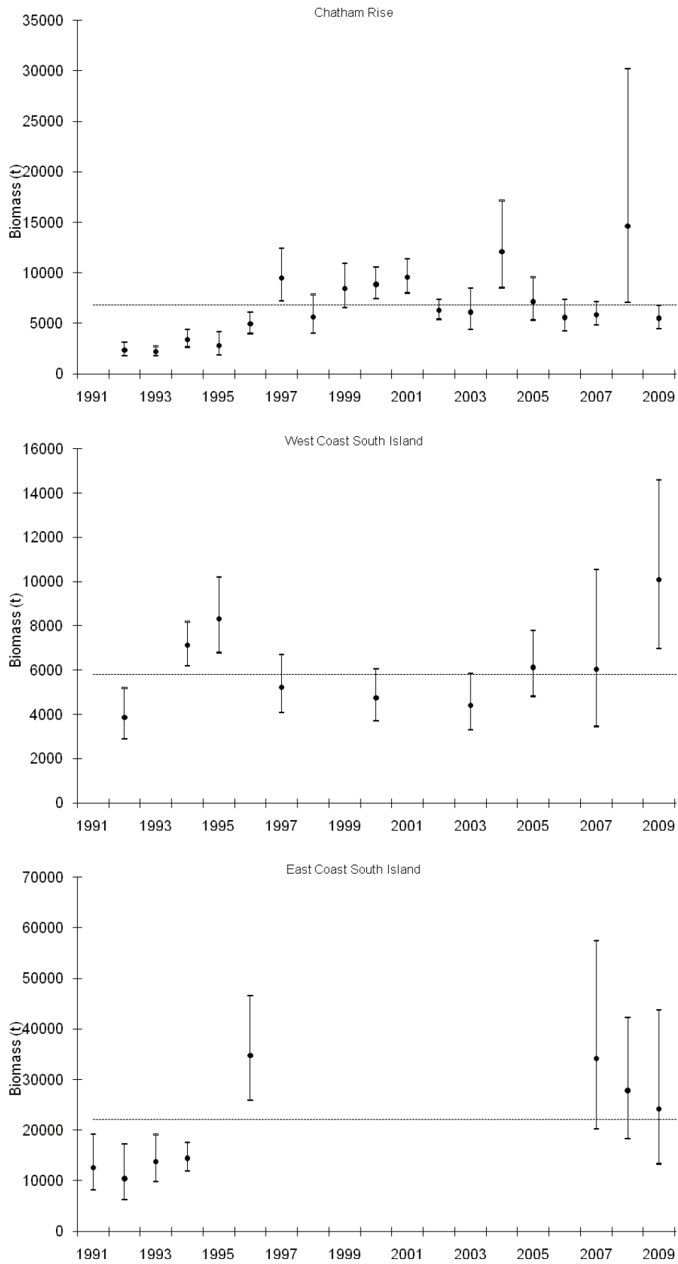
Figure 2: Spiny dogfish biomass \pm 95\% CI (estimated from survey CV's assuming a lognormal distribution) and the time series mean (dotted line) estimated from the Chatham Rise (Top), West (Middle) and East (bottom) Coast South Island trawl survey.
