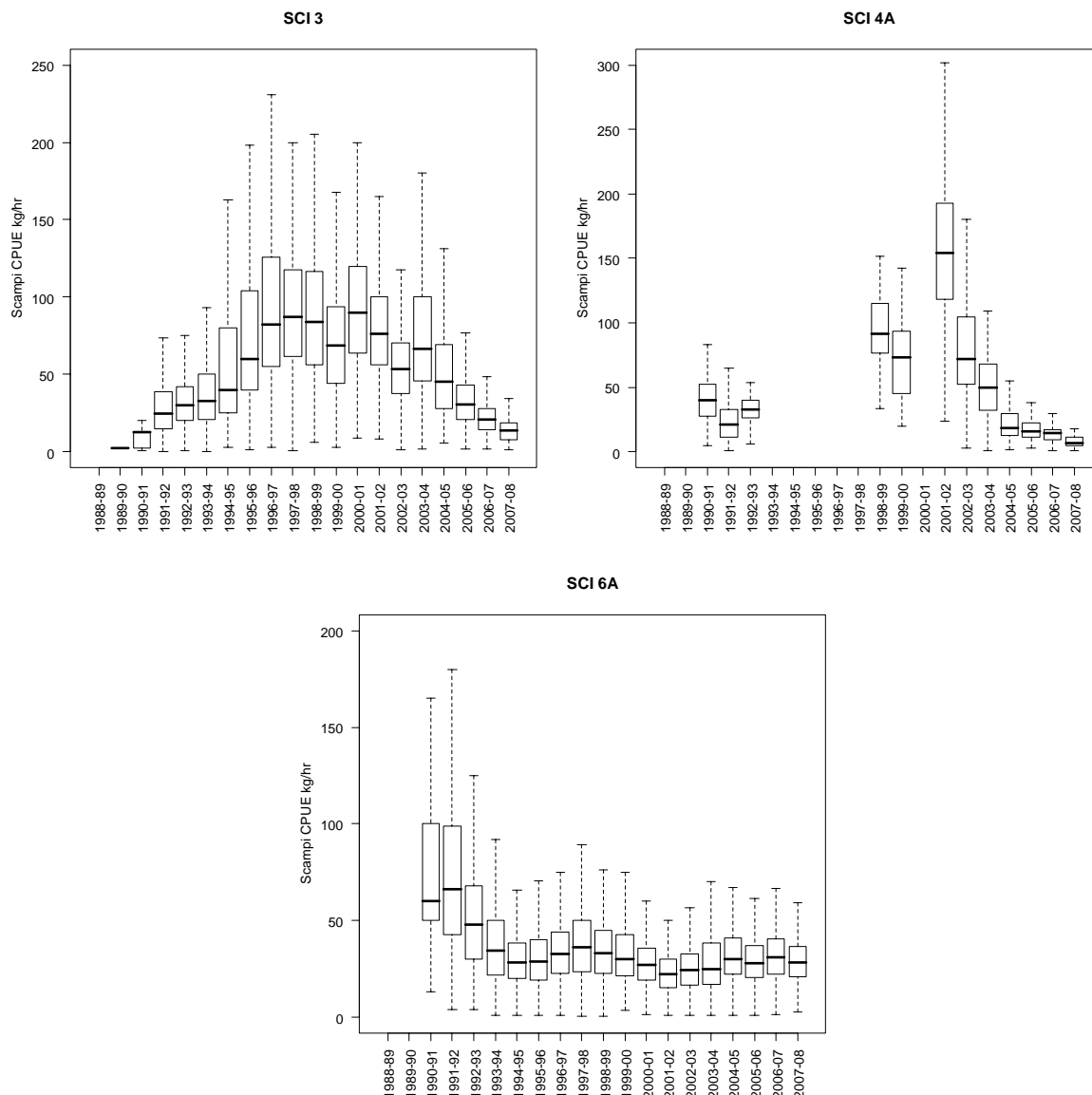
Figure 2 [Continued]: Box plots (with outliers removed) of individual observations of unstandardised catch rate for scampi (tow catch (kg) divided by tow effort (hours)) with tows of zero scampi catch excluded, by fishing year for main stocks. Note different scales between plots. Horizontal bars within boxes represent distribution median. Upper and lower limits of boxes represent upper and lower quartiles. Whisker extends to largest (or smallest) observation which is less than or equal (greater than or equal) to the upper quartile plus 1.5 times the interquartile range (lower quartile less 1.5 times the interquartile range). Outliers (removed from this plot) are values outside the whiskers.
