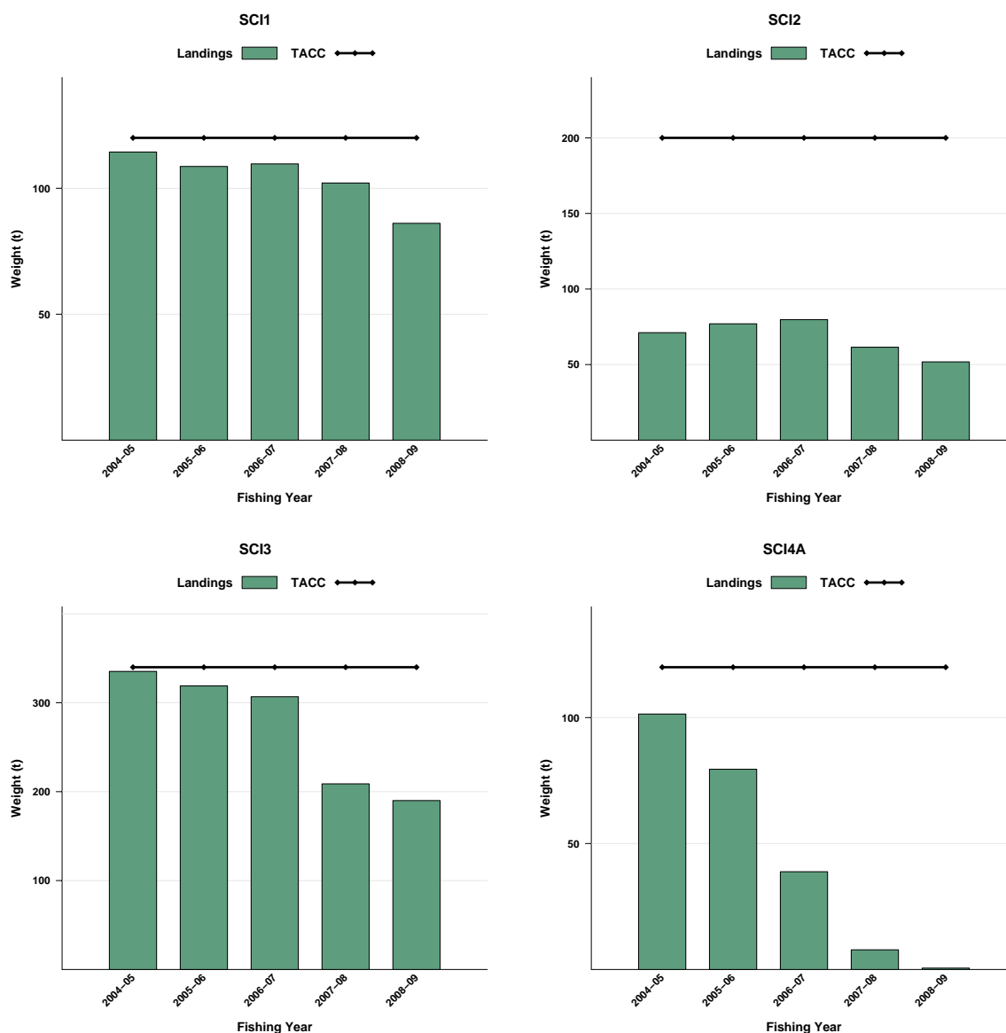
Figure 1: Historical landings and TACC for the five main SCI stocks. From top left: SCI1 (Auckland East), SCI2 (Central East), SCI3 (South East Coast), SCI 4A (Chatham Islands East). [Continued on next page]...
