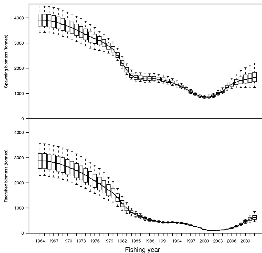
Figure 6: The posterior biomass trajectories for spawning (upper) and recruited (lower) biomass for the base case for PAU 7. For each year, the figure shows the median of the posterior (horizontal bar), the 25th and 75th percentiles (box) and 5th and 95th percentiles of the posterior.
