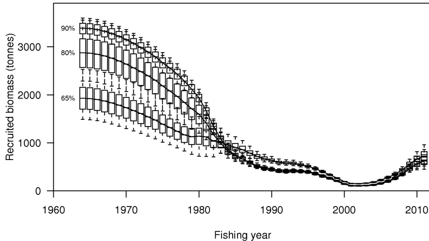
Figure 7: Recruited biomass trajectories from the MCMC sensitivity trials in which maximum allowed exploitation rate was varied from 80% in the base case to 65% and 90%. The 65% trial is the line that is lowest on the left and highest in the early 2000s.
