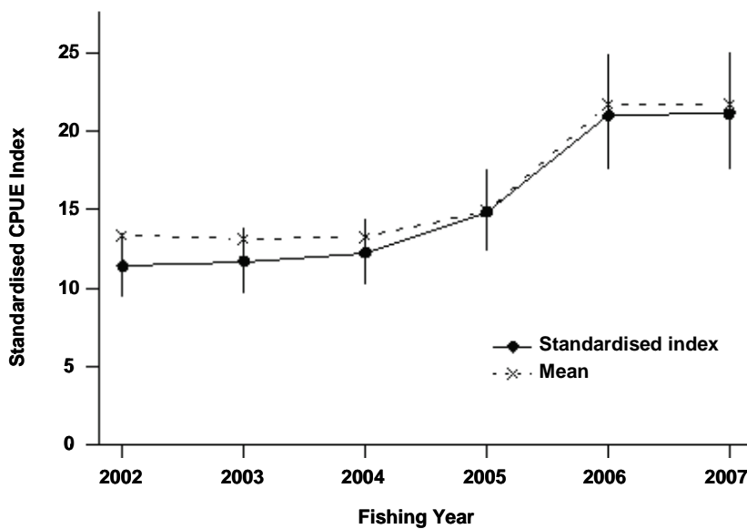
Figure 4: Standardised (with 95% confidence intervals) and unstandardised mean PCPUE (kg per diver hour) from PCELR forms, from statistical areas 17 and 18 combined.
