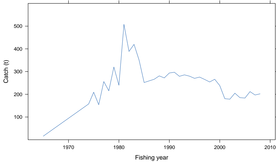
Figure 2: Assumed catch series used in the assessment. Only catches from Statistical Areas 17 and 38 were used.
