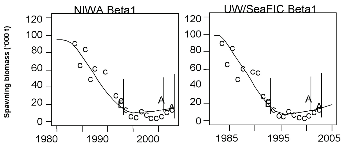
Figure 3: Estimated biomass trajectories (lines) and fitted data (points) from all model runs. Data are identified by plotting symbol ('c' = CPUE, 'A' = acoustic, 'E' = egg survey). CPUE data are scaled up to the biomass. Vertical bars for absolute indices show 95% confidence intervals. Plots are from the modes of the posterior distribution. The UW/SeaFIC assessment estimates biomass up to 2004–05 NIWA up to 2003–04).
