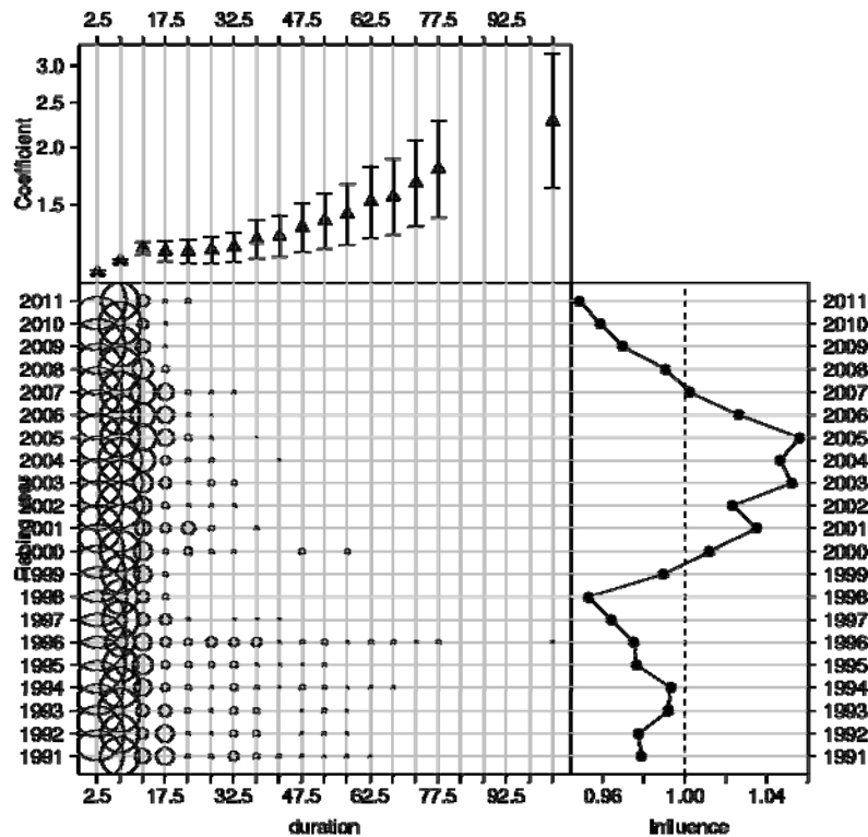
Figure D19: Effect and influence of \log \text{duration} in the YBF_HG gamma model. See caption (D1) for details.
