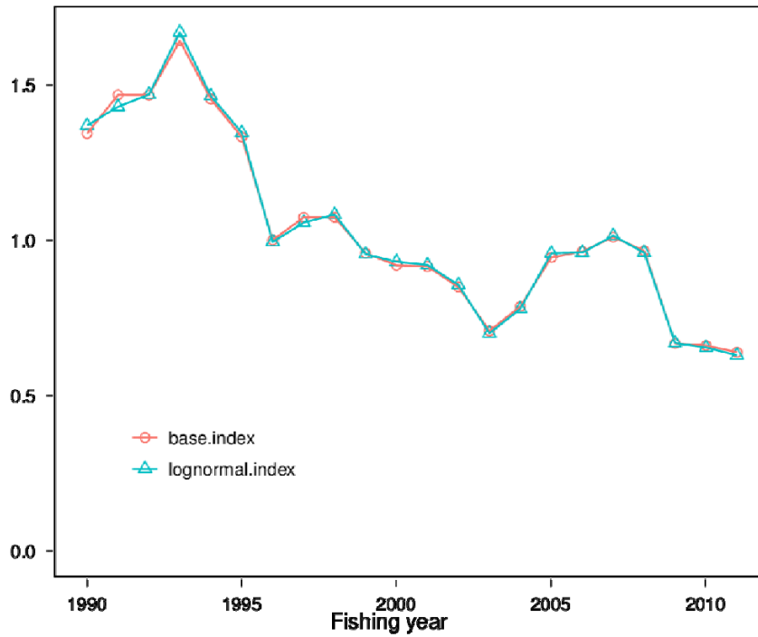
Figure G3: Comparison between the final log logistic index for (YBF) MH and an index from a similar model fit assuming lognormal errors.
