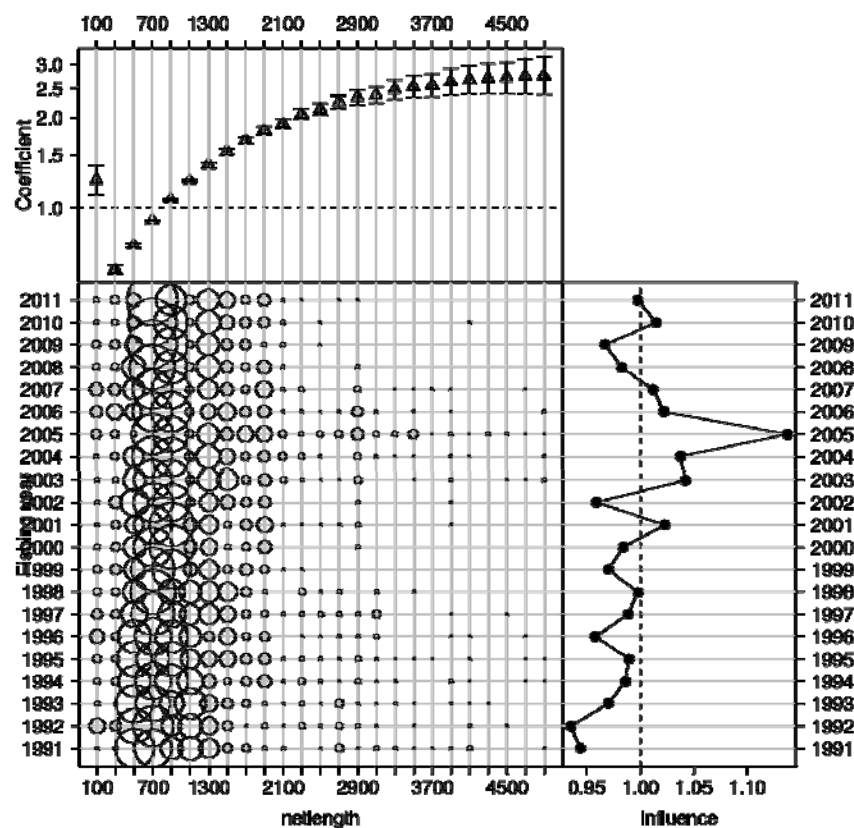
Figure D20: Effect and influence of \log \text{netlength} in the YBF_HG gamma model. See caption (D1) for details.
