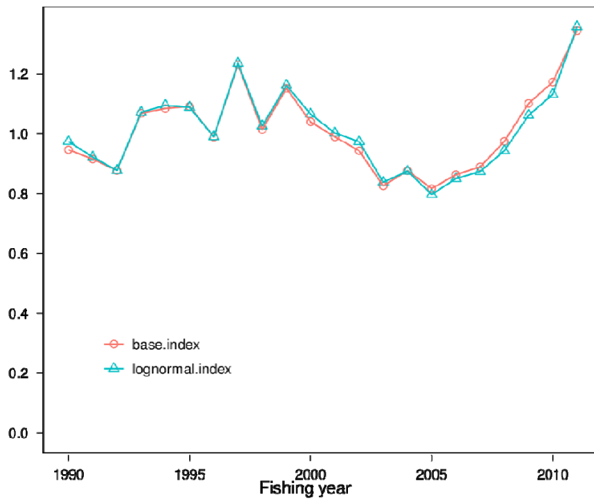
Figure G4: Comparison between the final log logistic index for (YBF) LW and an index from a similar model fit assuming lognormal errors.
