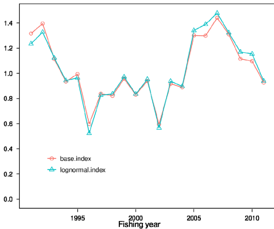
Figure G6: Comparison between the final gamma index for YBF_HG and an index from a similar model fit assuming lognormal errors.
