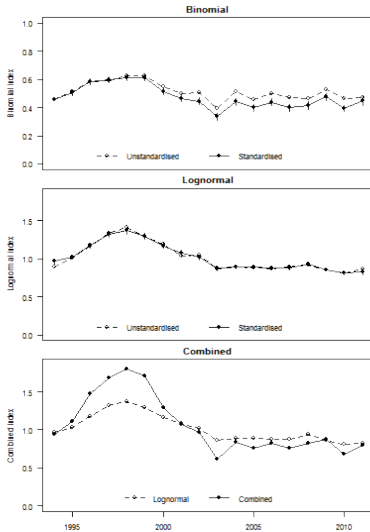
Figure D.4. Standardised annual CPUE indices for the model based on CRA 2 rllb potlift data using year , month , vessel , statistical area , depth and soak time as explanatory variables. [top panel] binomial index representing probability of capture; [centre panel] lognormal index representing magnitude of positive catch records; [bottom panel] combined index using delta method representing expected catch
