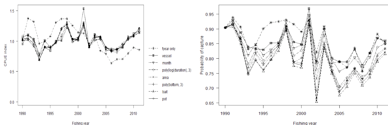
Figure K.2. Year index coefficients for the standardised CPUE analysis based on CRA 7 rlcs potlift data using year, month, vessel, statistical area, pot type, bait type, depth and soak time as explanatory variables: effect of adding successive variables to the trajectory of Y_{y_i} indices; [left panel] lognormal model using positive catch records [right panel] binomial logit model of the probability of a successful lift
