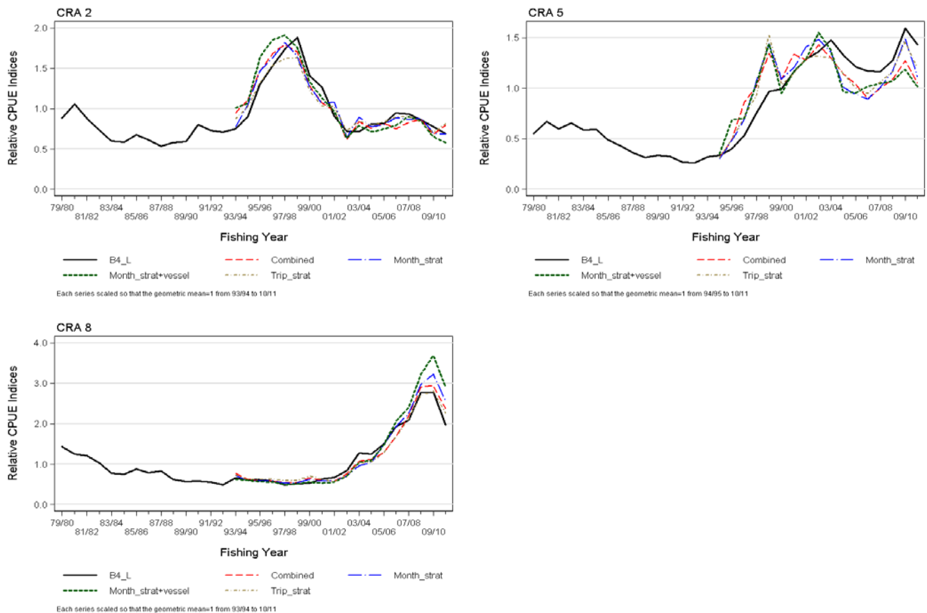
Figure 6: RLLB: comparison for CRA 2, CRA 5 and CRA 8 of (a) the annual “B4_L” CPUE analyses (based on MFish CELR data) with (b) the “Combined” series: Eq. 4 and Figure 5, (c) “Month_strat”: prepared and analysed in the same manner as the CELR data, (d) Month_strat+vessel”: same as (c) with added vessel explanatory variable and (e) “Trip_strat”, a daily series based on the [trip] field using [year], [month], and [statistical area] as explanatory variables.
