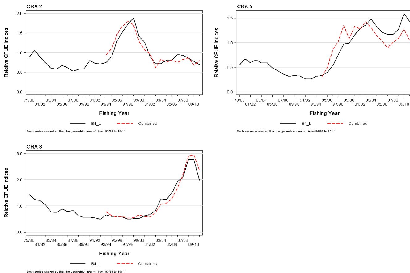
Figure 3. RLLB: comparison of the annual “B4_L” CPUE analyses (based on MFish CELR data) for CRA 2, CRA 5 and CRA 8 with the combined standardised CPUE analyses (Eq. 4) for the same three QMAs (CRA 2:Appendix A; CRA 5: Appendix E; CRA 8:Appendix F), based on potlift data using all available explanatory variables.
