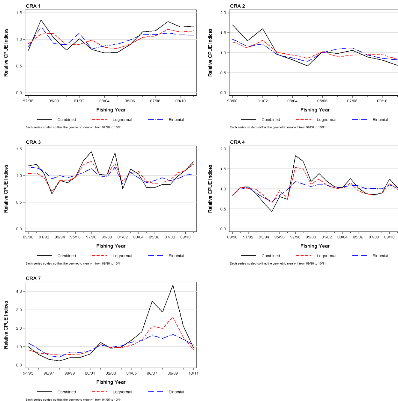
Figure 4. RLCS: three standardised potlift-based CPUE analyses (lognormal [Eq. 3], binomial [Eq. 3, modified as described in Section 3.1C], and combined [Eq. 4], plotted for CRA 1, CRA 2, CRA 3, CRA 4 and CRA 7, using all available explanatory variables listed in Table G.2 (CRA 1), Table H.2 (CRA 2), Table I.2 (CRA 3), Table J.2 (CRA 4) and Table K.2 (CRA 7).
