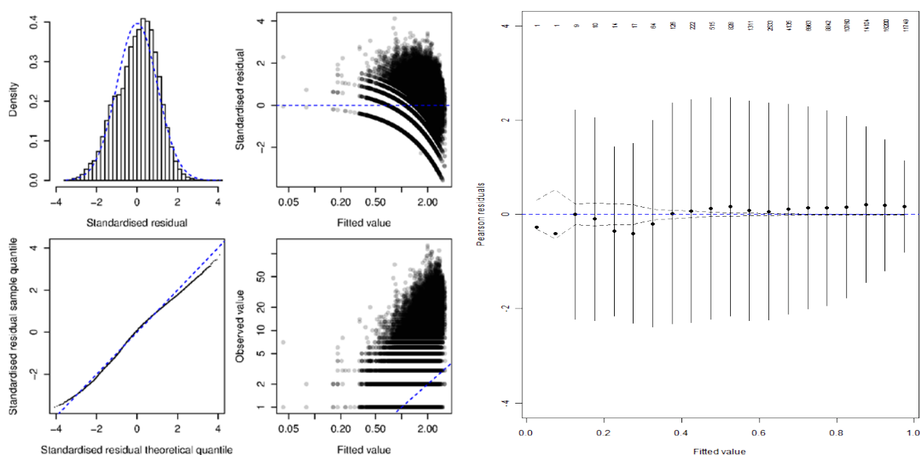
Figure J.1. Residual plots for CRA 4 CPUE regression analyses using year, month, vessel, statistical area, pot type, bait type, depth and soak time as explanatory variables on potlift data from the rlcs database. [left panel] residuals from the lognormal model using positive catch records [right panel] residuals from the binomial logit model of the probability of a successful lift.
