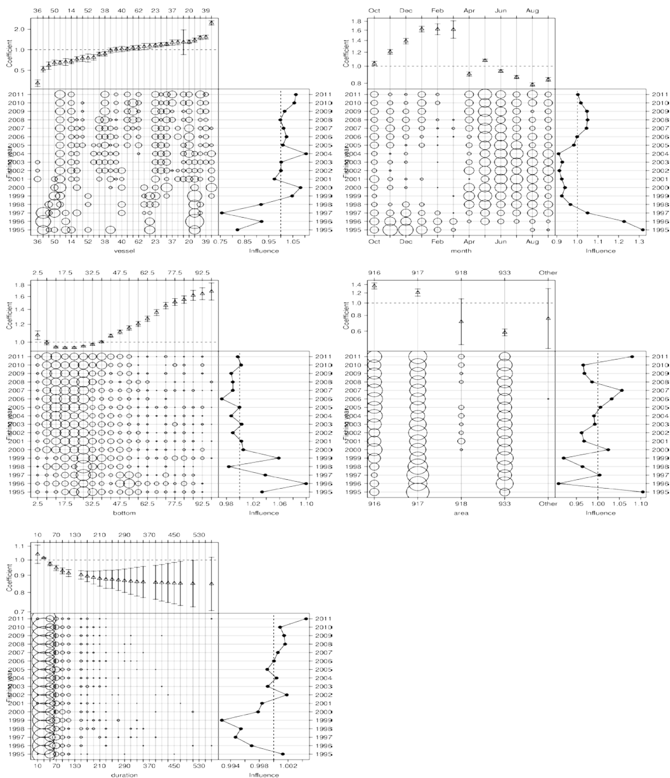
Figure E.3. “Influence” plots (Bentley et al. 2011) showing the relative effect of each explanatory variable on the standardised CPUE analysis based on CRA 5 rllb potlift data using year, month, vessel, statistical area, depth and soak time as explanatory variables: [upper left panel] vessel categorical variable; [upper right panel] month categorical variable; [centre left panel] depth continuous variable; [centre right panel] statistical area categorical variable; [lower left panel] soak_time continuous variable;
