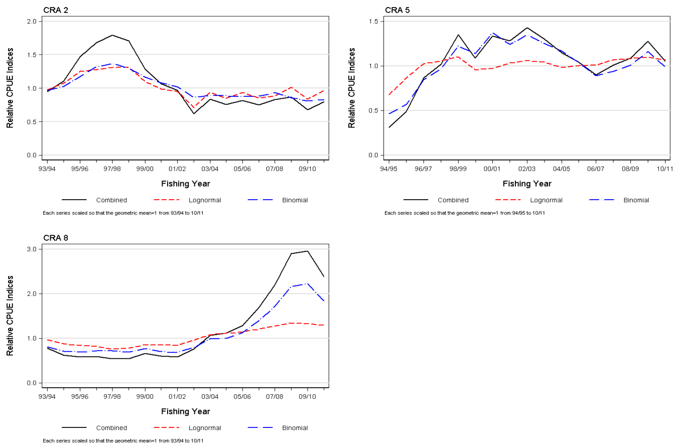
Figure 2. RLLB: three standardised potlift-based CPUE analyses (lognormal [Eq. 3], binomial [Eq. 3, modified as described in Section 3.1C], and combined [Eq. 4], plotted for CRA 2, CRA 5 and CRA 8, using all available explanatory variables listed in Table D.2 (CRA 2), Table E.2 (CRA 5), and Table F.2 (CRA 8).
