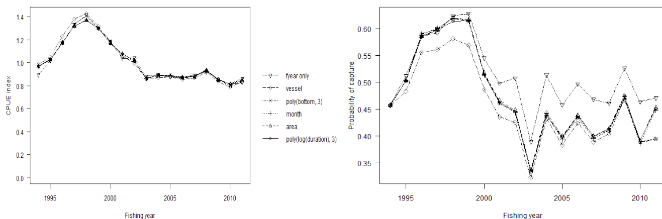
Figure D.2. Year index coefficients for the standardised CPUE analysis based on CRA 2 rllb potlift data using year, month, vessel, statistical area, depth and soak time as explanatory variables: effect of adding successive variables to the trajectory of Y_{y_i} indices; [left panel] lognormal model using positive catch records [right panel] binomial logit model of the probability of a successful lift
