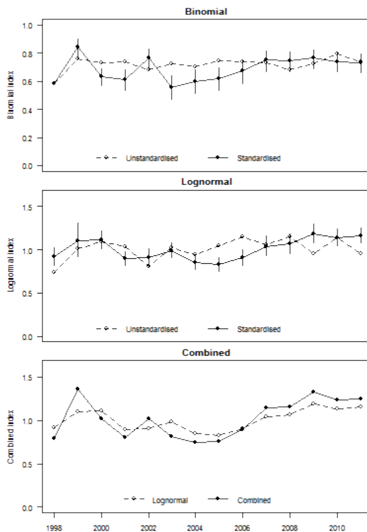
Figure G.4. Standardised annual CPUE indices for the model based on CRA 1 rlcs potlift data using year , month , vessel , statistical area , pot type , bait type , depth and soak time as explanatory variables. [top panel] binomial index representing probability of capture; [centre panel] lognormal index
