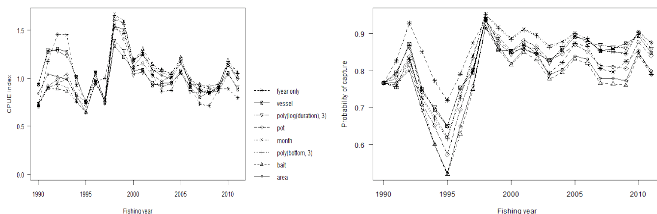
Figure J.2. Year index coefficients for the standardised CPUE analysis based on CRA 4 rlcs potlift data using year, month, vessel, statistical area, pot type, bait type, depth and soak time as explanatory variables: effect of adding successive variables to the trajectory of Y_{y_i} indices; [left panel] lognormal model using positive catch records [right panel] binomial logit model of the probability of a successful lift
