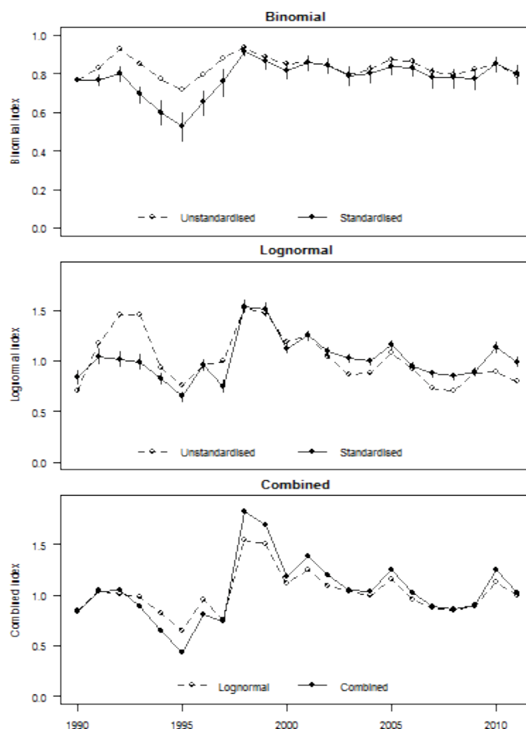
Figure J.4. Standardised annual CPUE indices for the model based on CRA 4 rlc's potlift data using year , month , vessel , statistical area , pot type , bait type , depth and soak time as explanatory variables. [top panel] binomial index representing probability of capture; [centre panel] lognormal index representing magnitude of positive catch records; [bottom panel] combined index using delta method representing expected catch
