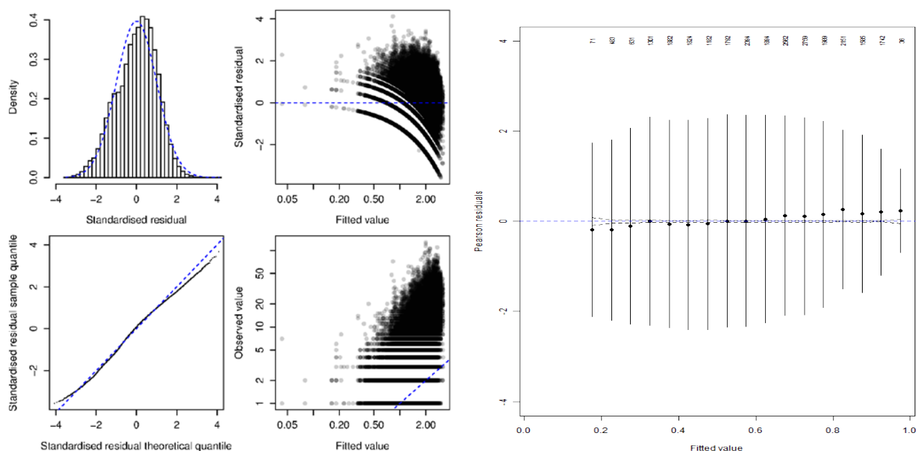
Figure K.1. Residual plots for CRA 7 CPUE regression analyses using year, month, vessel, statistical area, pot type, bait type, depth and soak time as explanatory variables on potlift data from the rlcs database. [left panel] residuals from the lognormal model using positive catch records [right panel] residuals from the binomial logit model of the probability of a successful lift.
