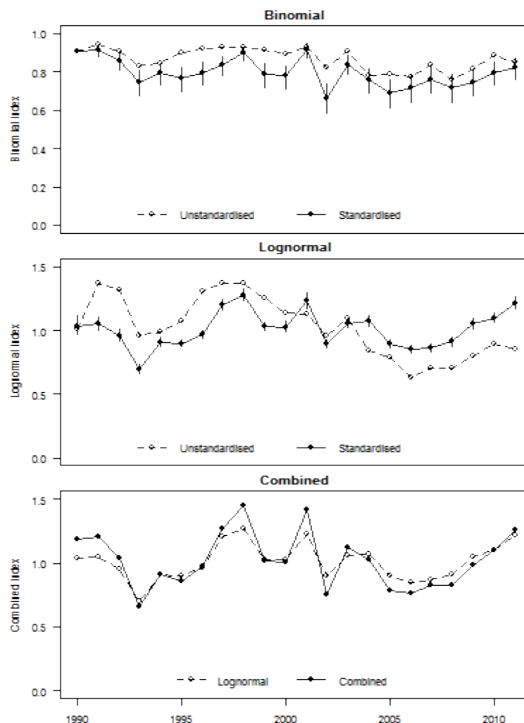
Figure I.4. Standardised annual CPUE indices for the model based on CRA 3 rlcs potlift data using year , month , vessel , statistical area , pot type , bait type , depth and soak time as explanatory variables. [top panel] binomial index representing probability of capture; [centre panel] lognormal index representing magnitude of positive catch records; [bottom panel] combined index using delta method representing expected catch
