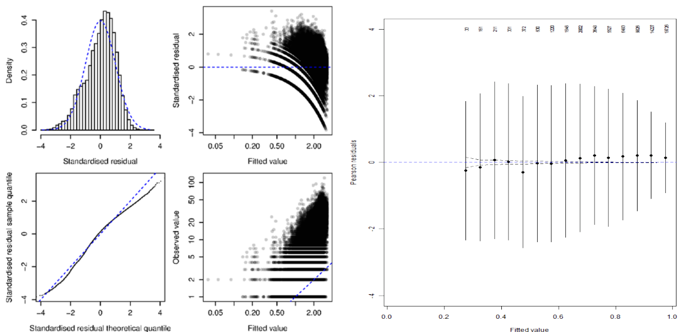
Figure I.1. Residual plots for CRA 3 CPUE regression analyses using year, month, vessel, statistical area, pot type, bait type, depth and soak time as explanatory variables on potlift data from the rlcs database. [left panel] residuals from the lognormal model using positive catch records [right panel] residuals from the binomial logit model of the probability of a successful lift.
