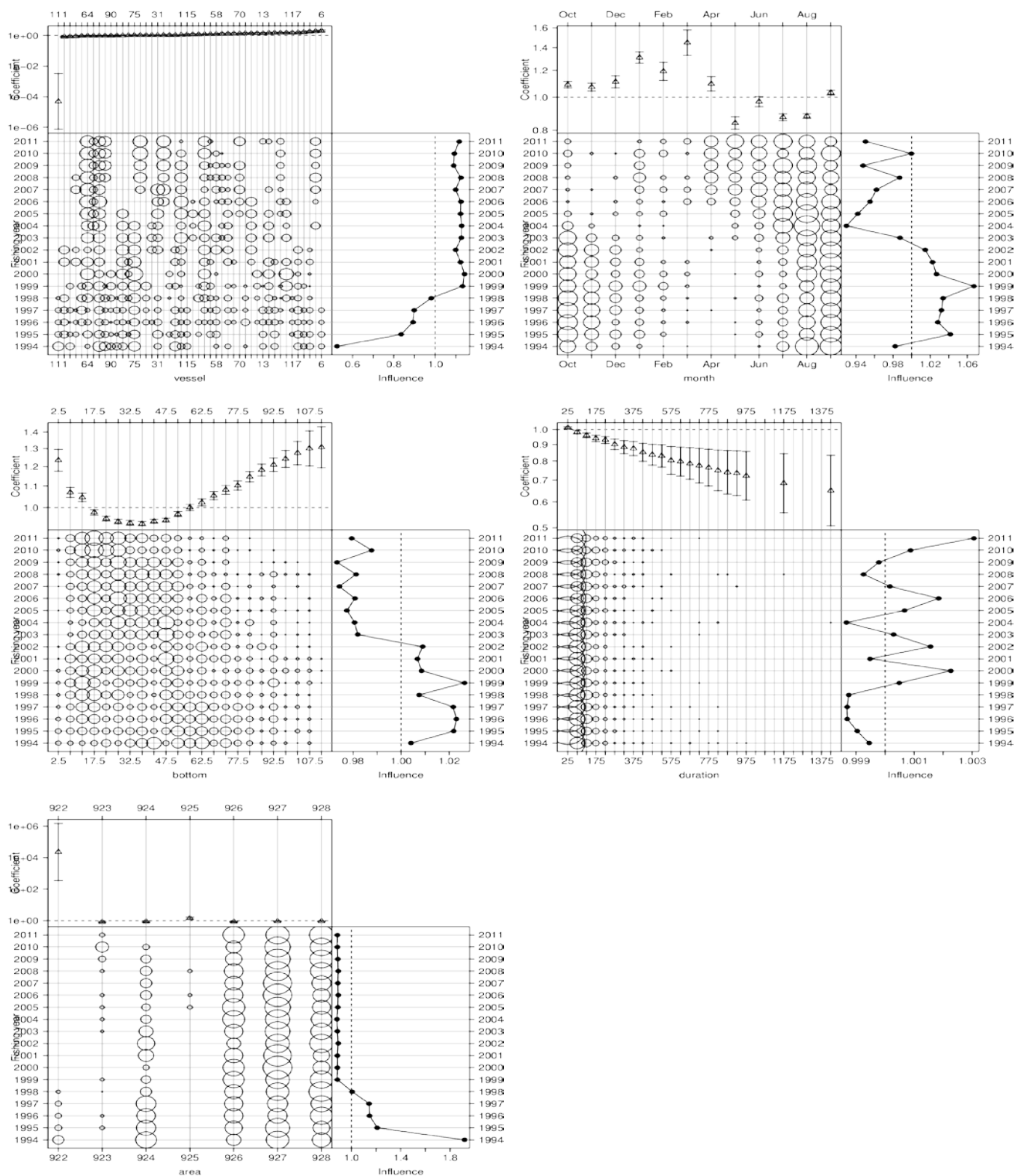
Figure F.3. “Influence” plots (Bentley et al. 2011) showing the relative effect of each explanatory variable on the standardised CPUE analysis based on CRA 8 r/lb potlift data using year, month, vessel, statistical area, depth and soak time as explanatory variables: [upper left panel] vessel categorical variable; [upper right panel] month categorical variable; [centre left panel] depth continuous variable; [centre right panel] soak_time continuous variable; [lower left panel] statistical area categorical variable
