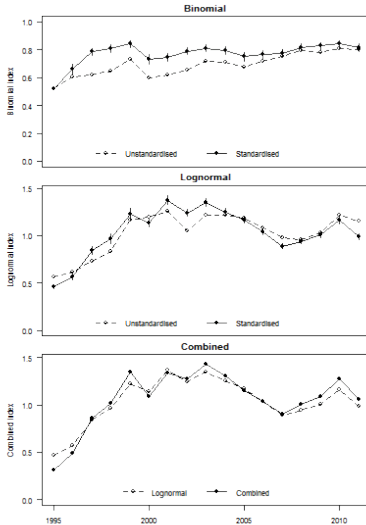
Figure H.4. Standardised annual CPUE indices for the model based on CRA 2 rlcs potlift data using year , month , vessel , statistical area , pot type , bait type , depth and soak time as explanatory variables. [top panel] binomial index representing probability of capture; [centre panel] lognormal index representing magnitude of positive catch records; [bottom panel] combined index using delta method representing expected catch
