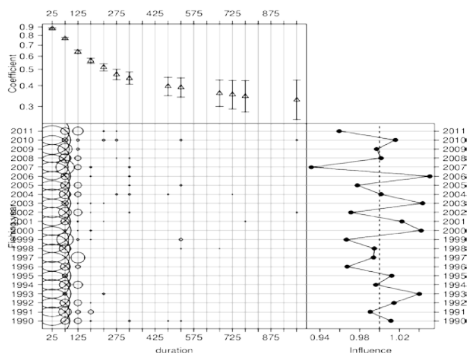
Figure K.3. (cont.): soak_time continuous variable
