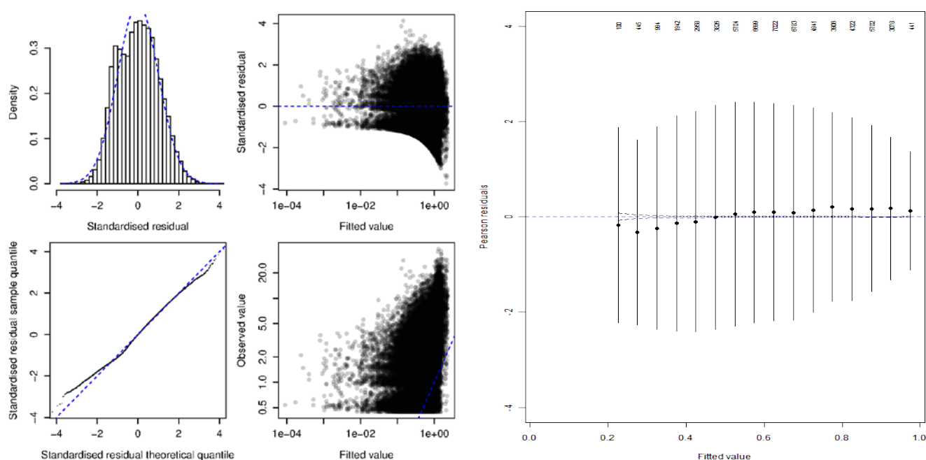
Figure F.1. Residual plots for CRA 8 CPUE regression analyses using year , month , vessel , statistical area , depth and soak time as explanatory variables on potlift data from the rllb database. [left panel] residuals from the lognormal model using positive catch records [right panel] residuals from the binomial logit model of the probability of a successful lift.
