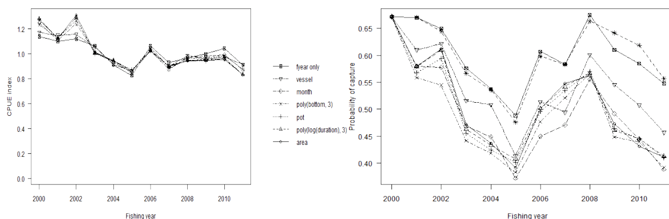
Figure H.2. Year index coefficients for the standardised CPUE analysis based on CRA 2 rlcs potlift data using year, month, vessel, statistical area, pot type, bait type, depth and soak time as explanatory variables: effect of adding successive variables to the trajectory of Y_{y_i} indices; [left panel] lognormal model using positive catch records [right panel] binomial logit model of the probability of a successful lift
