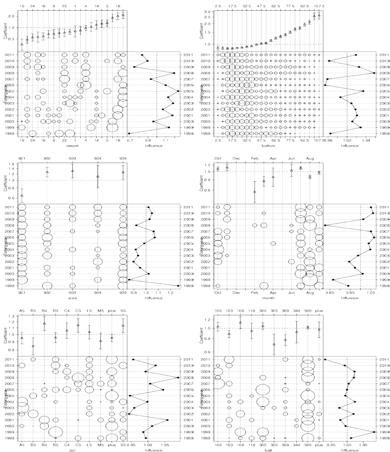
Figure G.3. "Influence" plots (Bentley et al. 2011) showing the relative effect of each explanatory variable on the standardised CPUE analysis based on CRA 1 r/lcs potlift data using year, month, vessel, statistical area, pot type, bait type, depth and soak time as explanatory variables: [upper left panel] vessel categorical variable; [upper right panel] depth continuous variable; [centre left panel] statistical area categorical variable; [centre right panel] month categorical variable; [lower left panel] pot type categorical variable; [lower right panel] bait type categorical variable;
