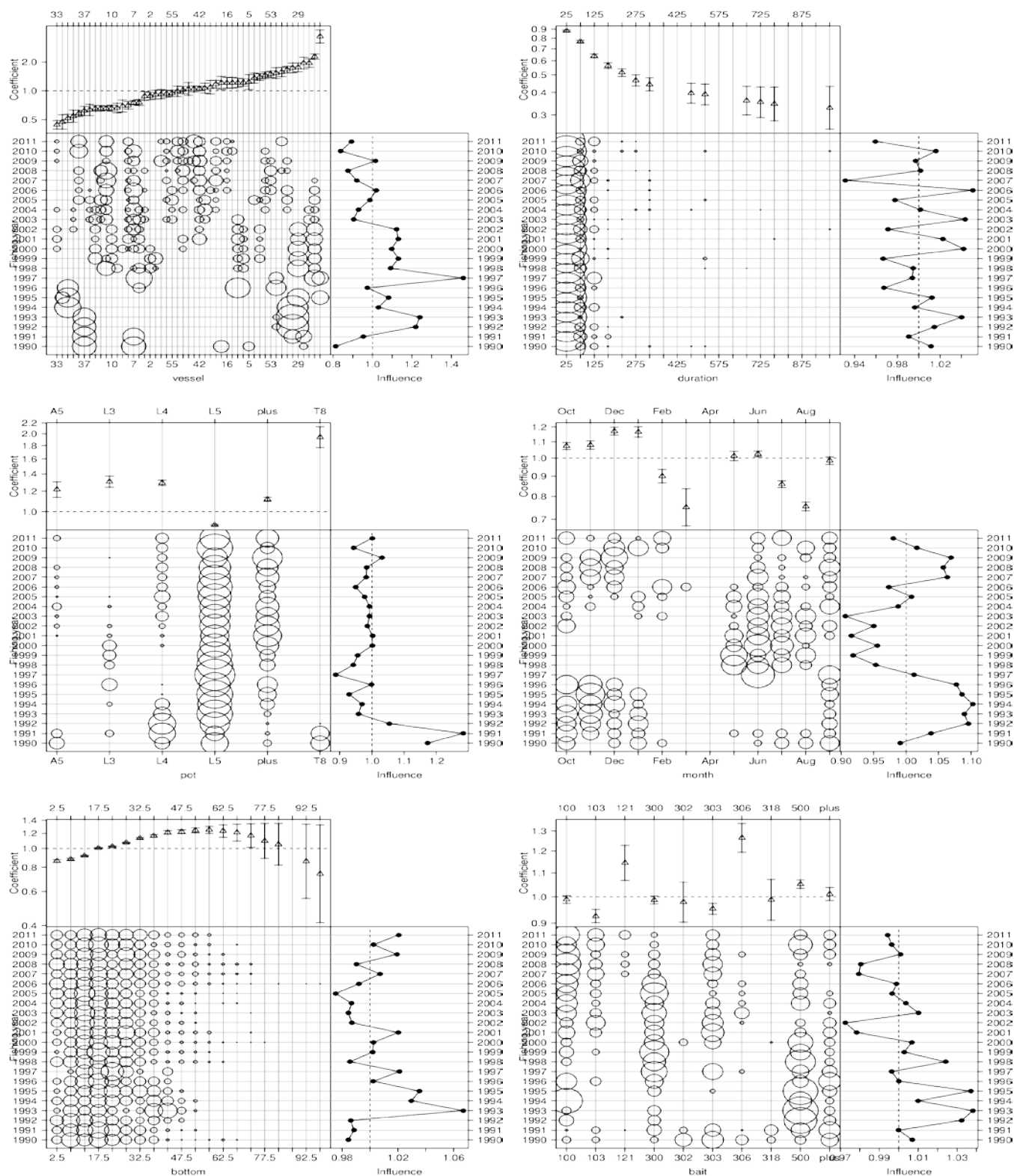
Figure J.3. “Influence” plots (Bentley et al. 2011) showing the relative effect of each explanatory variable on the standardised CPUE analysis based on CRA 4 r/lcs potlift data using year, month, vessel, statistical area, pot type, bait type, depth and soak time as explanatory variables: [upper left panel] vessel categorical variable; [upper right panel] soak_time continuous variable; [centre left panel] pot type categorical variable; [centre right panel] month categorical variable; [lower left panel] depth continuous variable; [lower right panel] bait type categorical variable;
