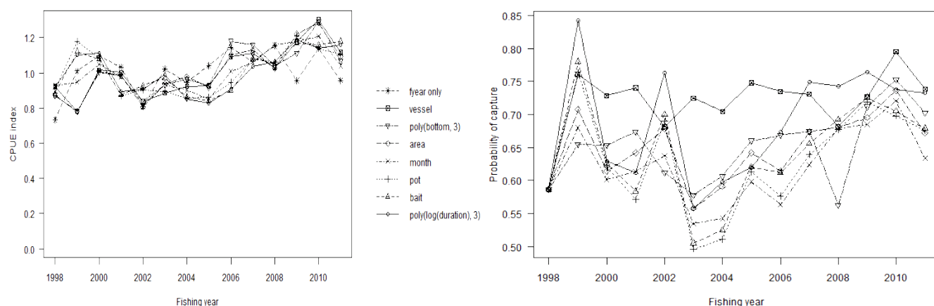
Figure G.2. Year index coefficients for the standardised CPUE analysis based on CRA 1 rlcs potlift data using year, month, vessel, statistical area, pot type, bait type, depth and soak time as explanatory variables: effect of adding successive variables to the trajectory of Y_{y_i} indices; [left panel] lognormal model using positive catch records [right panel] binomial logit model of the probability of a successful lift
