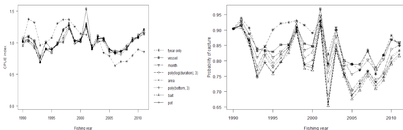
Figure I.2. Year index coefficients for the standardised CPUE analysis based on CRA 3 rlcs potlift data using year, month, vessel, statistical area, pot type, bait type, depth and soak time as explanatory variables: effect of adding successive variables to the trajectory of Y_{y_i} indices; [left panel] lognormal model using positive catch records [right panel] binomial logit model of the probability of a successful lift
