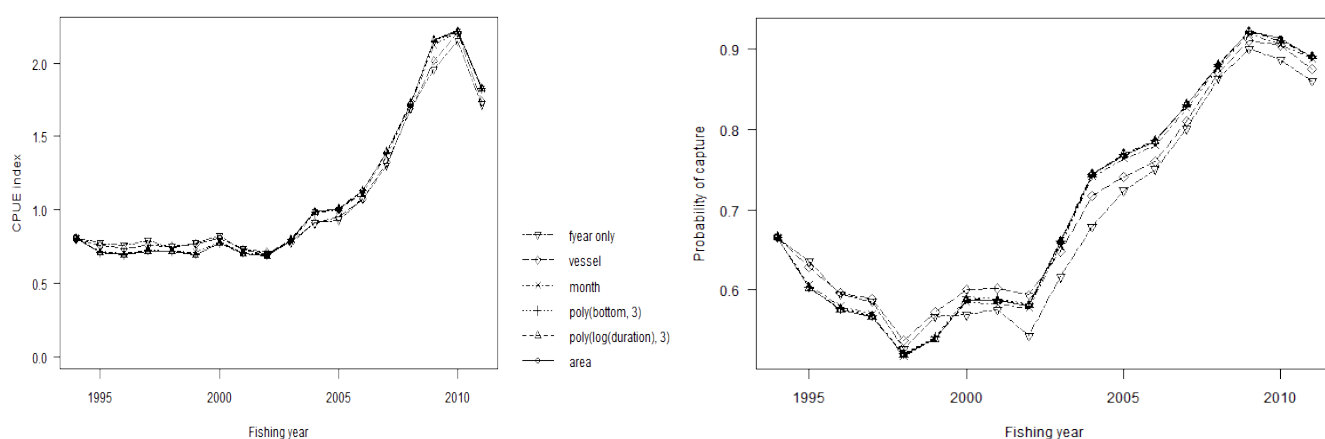
Figure F.2. Year index coefficients for the standardised CPUE analysis based on CRA 8 rllb potlift data using year , month , vessel , statistical area , depth and soak time as explanatory variables: effect of adding successive variables to the trajectory of Y_{y_i} indices; [left panel] lognormal model using positive catch records [right panel] binomial logit model of the probability of a successful lift
