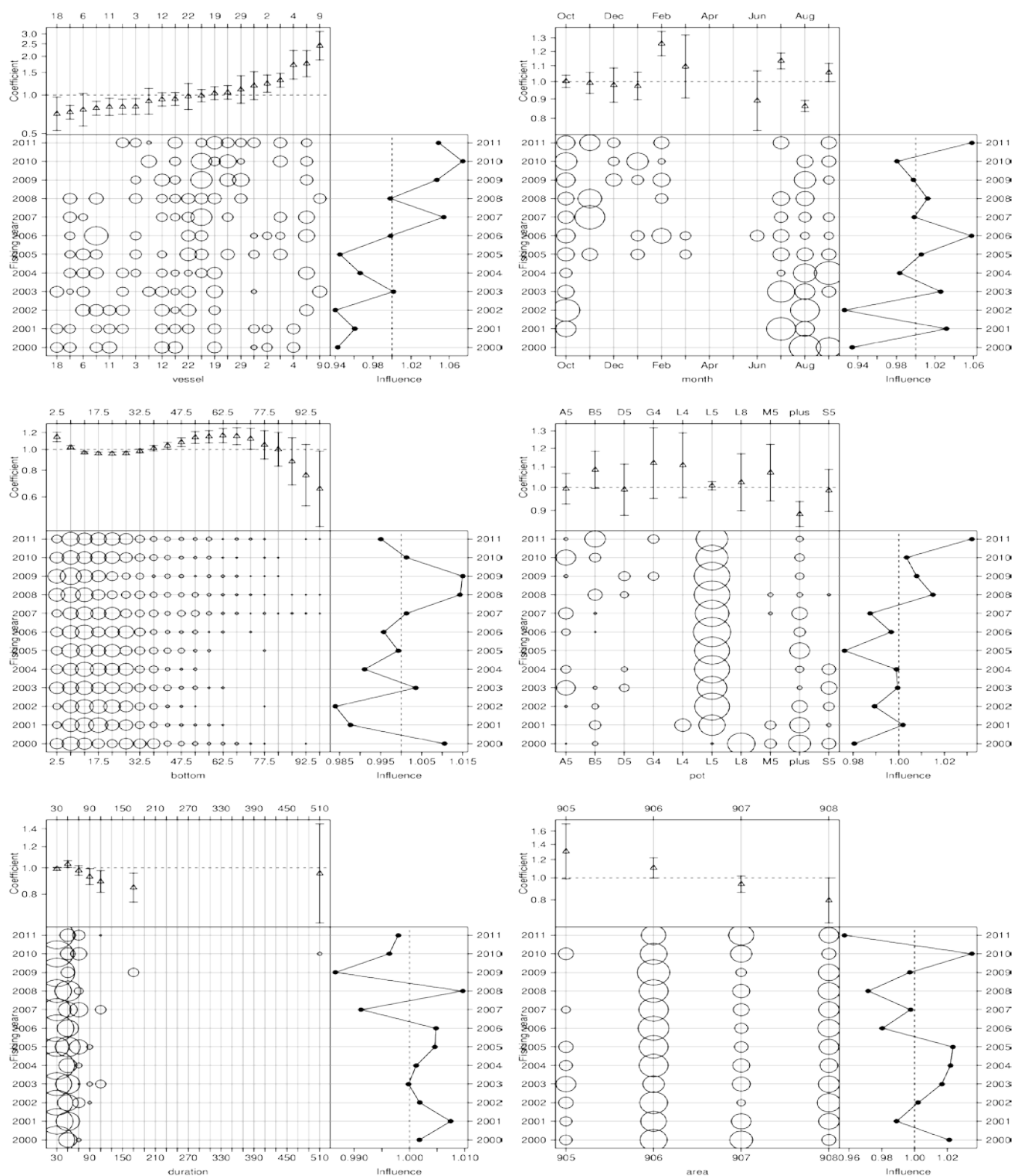
Figure H.3. “Influence” plots (Bentley et al. 2011) showing the relative effect of each explanatory variable on the standardised CPUE analysis based on CRA 2 r/lcs potlift data using year, month, vessel, statistical area, pot type, bait type, depth and soak time as explanatory variables: [upper left panel] vessel categorical variable; [upper right panel] month categorical variable; [centre left panel] depth continuous variable; [centre right panel] pot type categorical variable; [lower left panel] soak_time continuous variable; [lower right panel] statistical area categorical variable;
