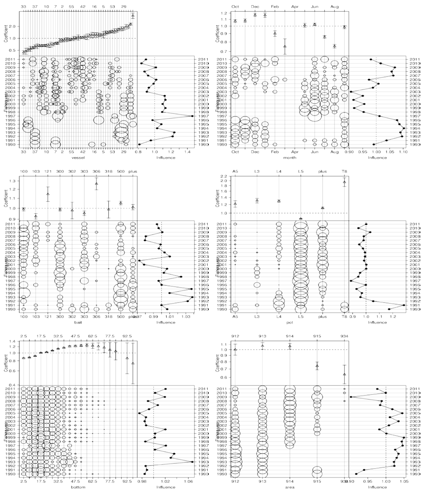
Figure K.3. “Influence” plots (Bentley et al. 2011) showing the relative effect of each explanatory variable on the standardised CPUE analysis based on CRA 7 r/lcs potlift data using year, month, vessel, statistical area, pot type, bait type, depth and soak time as explanatory variables: [upper left panel] vessel categorical variable; [upper right panel] month categorical variable; [centre left panel] bait type categorical variable; [centre right panel] pot type categorical variable; [lower left panel] depth continuous variable; [lower right panel] statistical area categorical variable;
