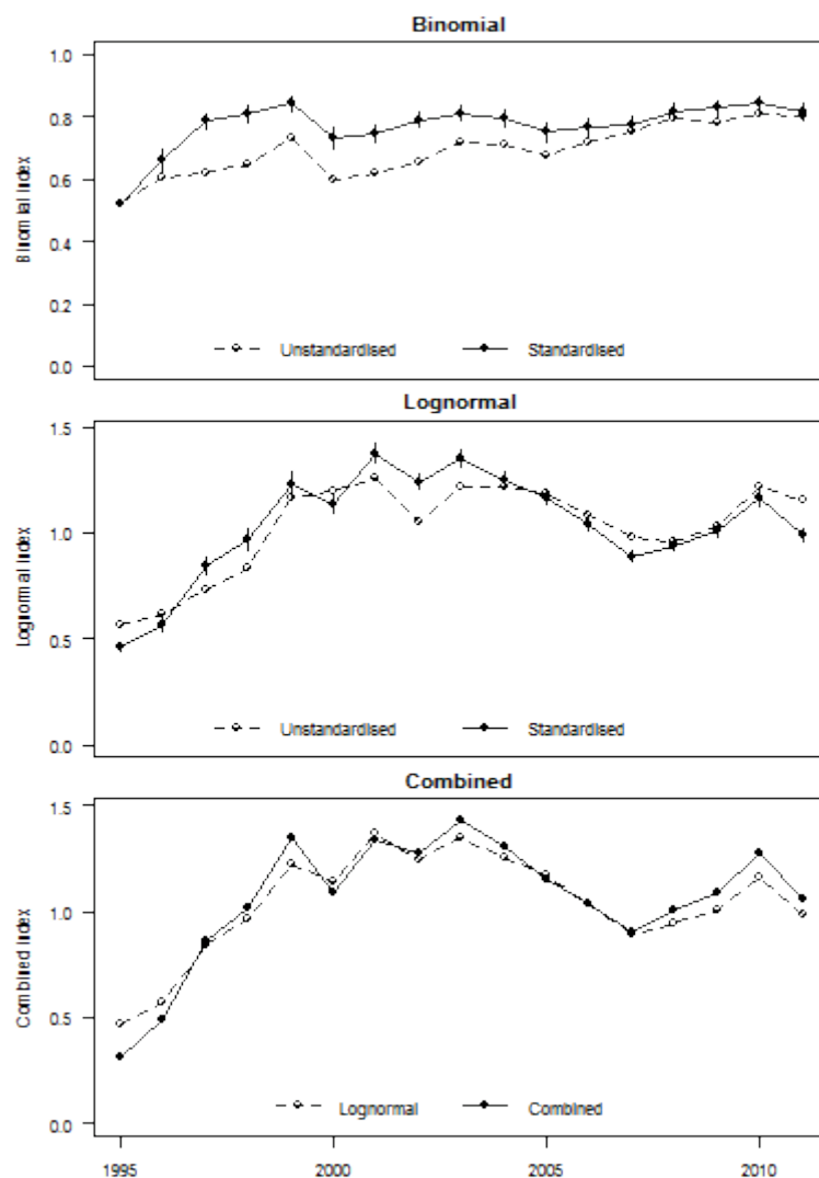
Figure E.4. Standardised annual CPUE indices for the model based on CRA 5 rllb potlift data using year , month , vessel , statistical area , depth and soak time as explanatory variables. [top panel] binomial index representing probability of capture; [centre panel] lognormal index representing magnitude of positive catch records; [bottom panel] combined index using delta method representing expected catch
