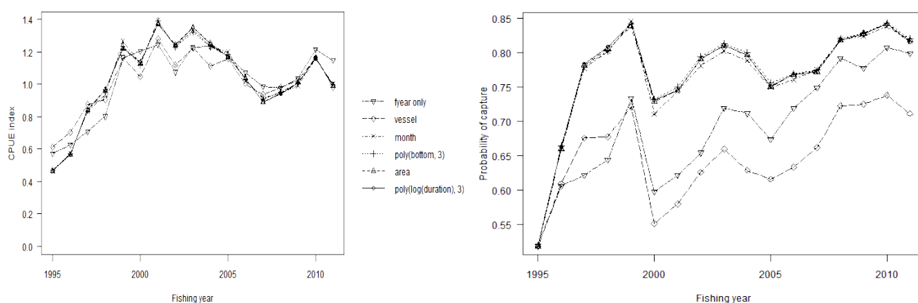
Figure E.2. Year index coefficients for the standardised CPUE analysis based on CRA 5 rllb potlift data using year , month , vessel , statistical area , depth and soak time as explanatory variables: effect of adding successive variables to the trajectory of Y_{y_i} indices; [left panel] lognormal model using positive catch records [right panel] binomial logit model of the probability of a successful lift
