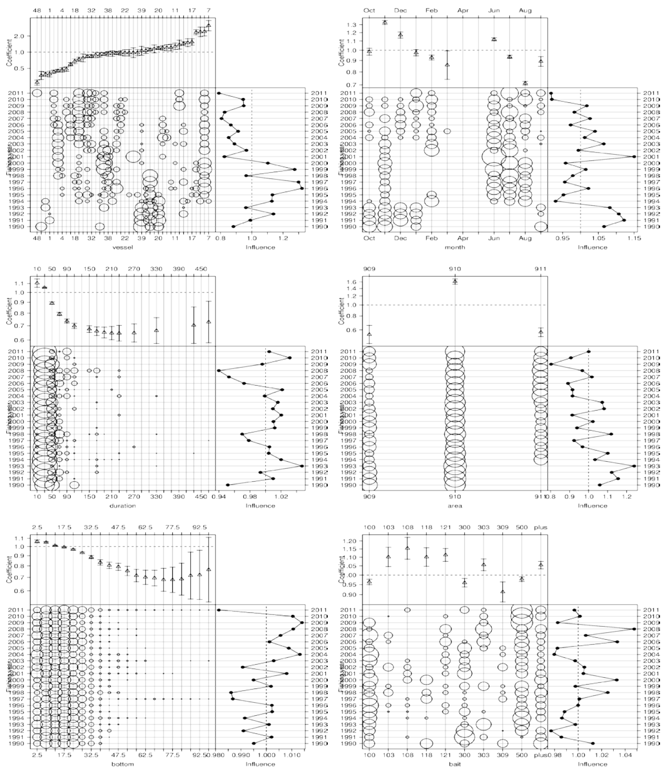
Figure I.3. “Influence” plots (Bentley et al. 2011) showing the relative effect of each explanatory variable on the standardised CPUE analysis based on CRA 3 r/lcs potlift data using year, month, vessel, statistical area, pot type, bait type, depth and soak time as explanatory variables: [upper left panel] vessel categorical variable; [upper right panel] month categorical variable; [centre left panel] soak_time continuous variable; [centre right panel] statistical area categorical variable; [lower left panel] depth continuous variable; [lower right panel] bait type categorical variable;
