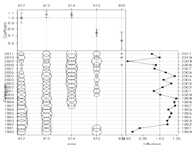
Figure J.3. (cont.): statistical area categorical variable
