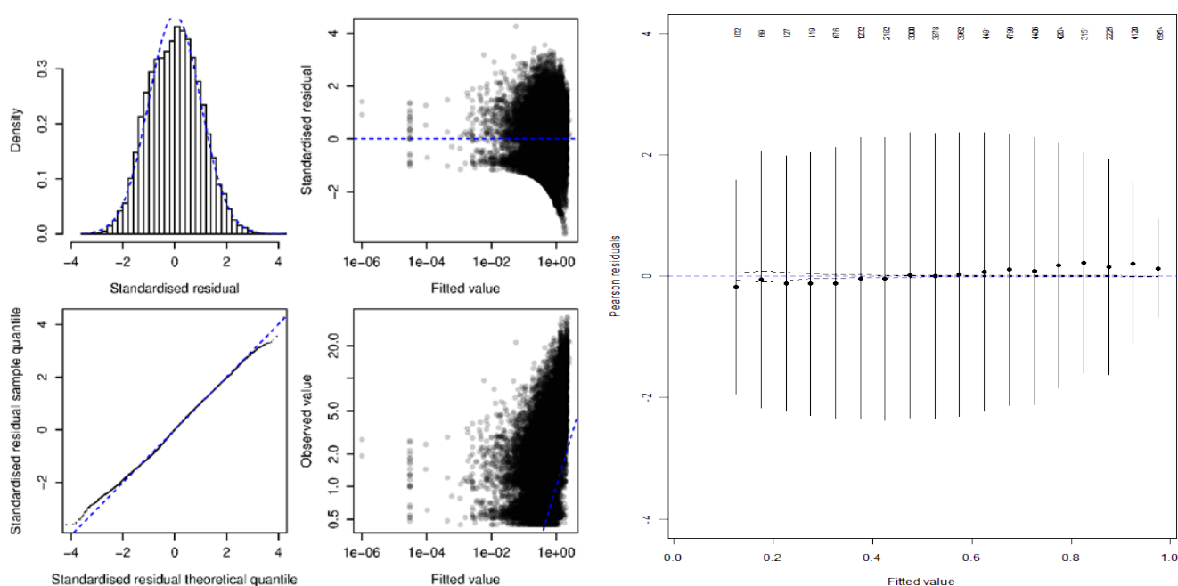
Figure E.1. Residual plots for CRA 5 CPUE regression analyses using year , month , vessel , statistical area , depth and soak time as explanatory variables on potlift data from the rllb database. [left panel] residuals from the lognormal model using positive catch records [right panel] residuals from the binomial logit model of the probability of a successful lift.
