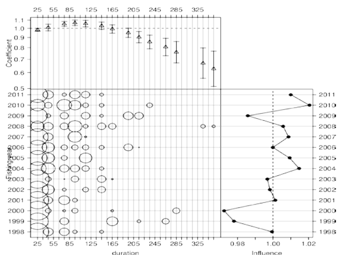
Figure G.3. (cont.): soak_time continuous variable
