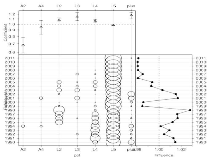
Figure I.3. (cont.): pot type categorical variable
