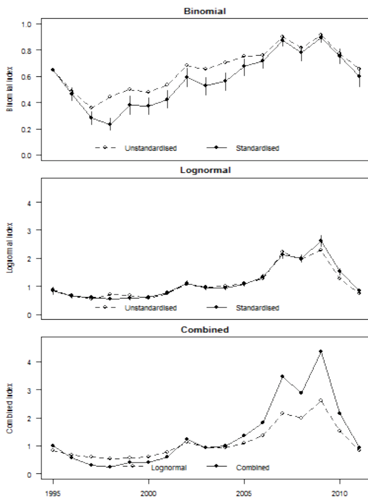
Figure K.4. Standardised annual CPUE indices for the model based on CRA 7 rlcs potlift data using year , month , vessel , statistical area , pot type , bait type , depth and soak time as explanatory variables. [top panel] binomial index representing probability of capture; [centre panel] lognormal index representing magnitude of positive catch records; [bottom panel] combined index using delta method representing expected catch
