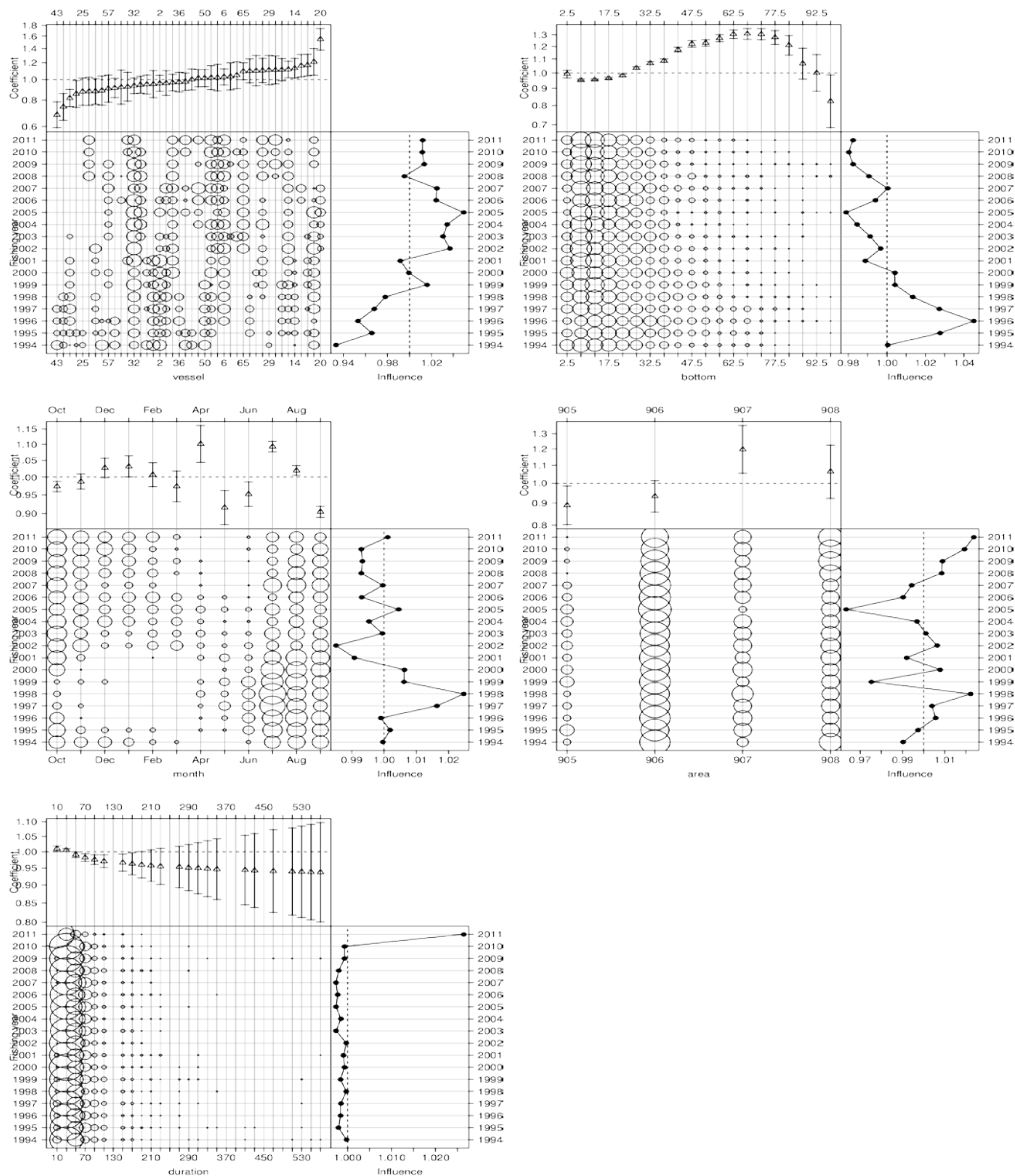
Figure D.3. “Influence” plots (Bentley et al. 2011) showing the relative effect of each explanatory variable on the standardised CPUE analysis based on CRA 2 rlb potlift data using year, month, vessel, statistical area, depth and soak time as explanatory variables: [upper left panel] vessel categorical variable; [upper right panel] depth continuous variable; [centre left panel] month categorical variable; [centre right panel] statistical area categorical variable; [lower left panel] soak_time continuous variable;
