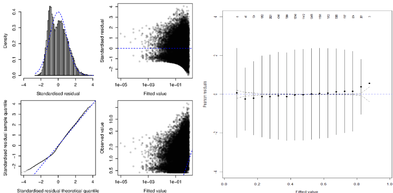
Figure D.1. Residual plots for CRA 2 CPUE regression analyses using year, month, vessel, statistical area, depth and soak time as explanatory variables on potlift data from the rllb database. [left panel] residuals from the lognormal model using positive catch records [right panel] residuals from the binomial logit model of the probability of a successful lift.
