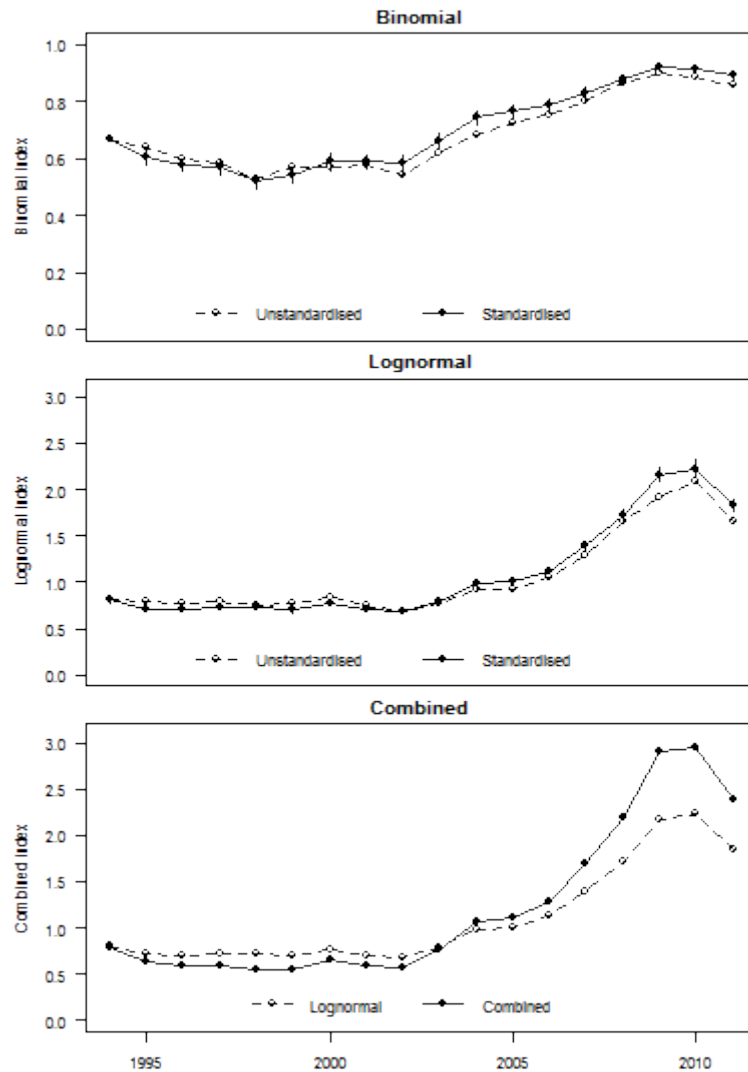
Figure F.4. Standardised annual CPUE indices for the model based on CRA 8 rllb potlift data using year , month , vessel , statistical area , depth and soak time as explanatory variables. [top panel] binomial index representing probability of capture; [centre panel] lognormal index representing magnitude of positive catch records; [bottom panel] combined index using delta method representing expected catch
