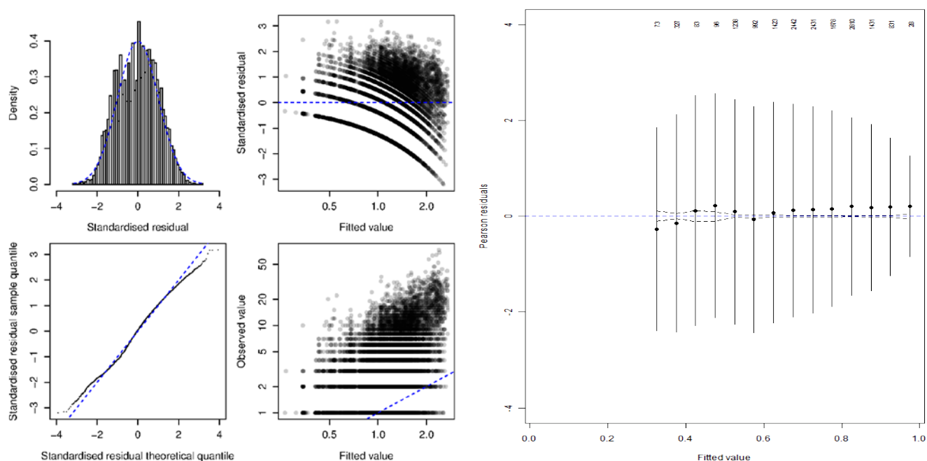
Figure G.1. Residual plots for CRA 1 CPUE regression analyses using year, month, vessel, statistical area, pot type, bait type, depth and soak time as explanatory variables on potlift data from the rlcs database. [left panel] residuals from the lognormal model using positive catch records [right panel] residuals from the binomial logit model of the probability of a successful lift.
