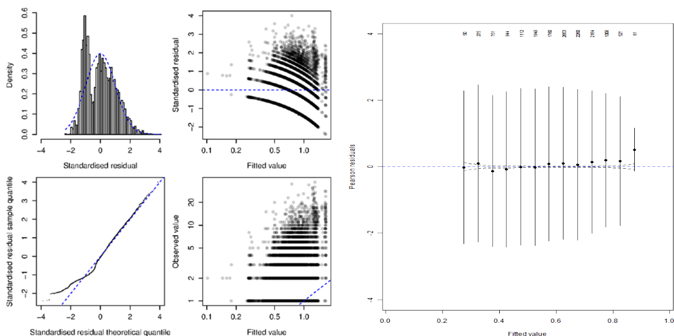
Figure H.1. Residual plots for CRA 2 CPUE regression analyses using year, month, vessel, statistical area, pot type, bait type, depth and soak time as explanatory variables on potlift data from the rlcs database. [left panel] residuals from the lognormal model using positive catch records [right panel] residuals from the binomial logit model of the probability of a successful lift.
