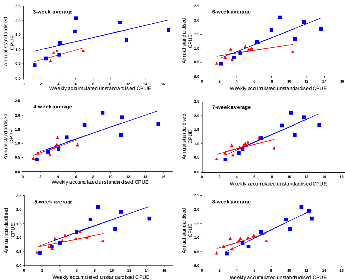
Figure E3 Correlations of weekly accumulated unstandardised CPUE (weeks 3–8) and annual standardised CPUE indices for two separate periods (1990–99 and 2000–08), for the Snare target bottom trawl fishery, 1989–90 – 2007–08.
