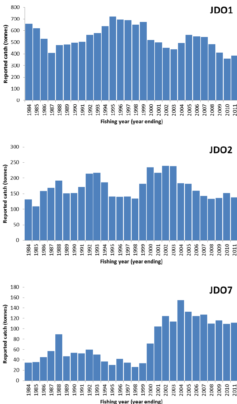
Figure 13: Reported landings of John dory by QMA (Ministry for Primary Industries 2012).
