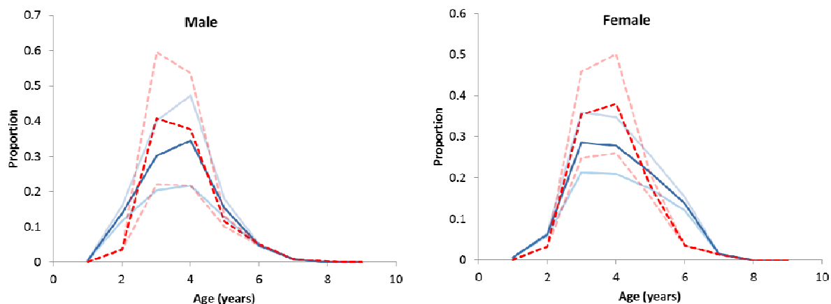
Figure 6: Estimated proportion at age (dark shaded lines) with 95% credible intervals (light shaded lines) for male and female John dory from the east coast of JDO1 (solid lines) and west coast JDO1 (broken lines). Estimates from Horn et al. (2006).
