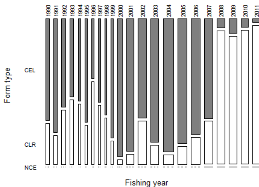
Figure A1.14: The proportion of reported landings of John dory by form type for JDO 7. Calculated from estimated greenweight. CEL, Catch Effort Landing Return; CLR, Catch Landing Return (for TCP and TCEPR forms); NCE, Netting Catch, Effort and Landing Return (for set nets, inshore drift nets, or pair set nets).
