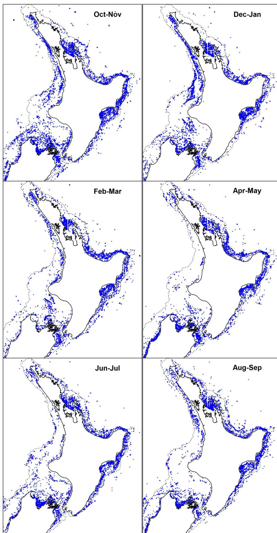
Figure 24: Location of bottom trawls from tow-by-tow data (points) in 2010–11, by bi-monthly groups.
