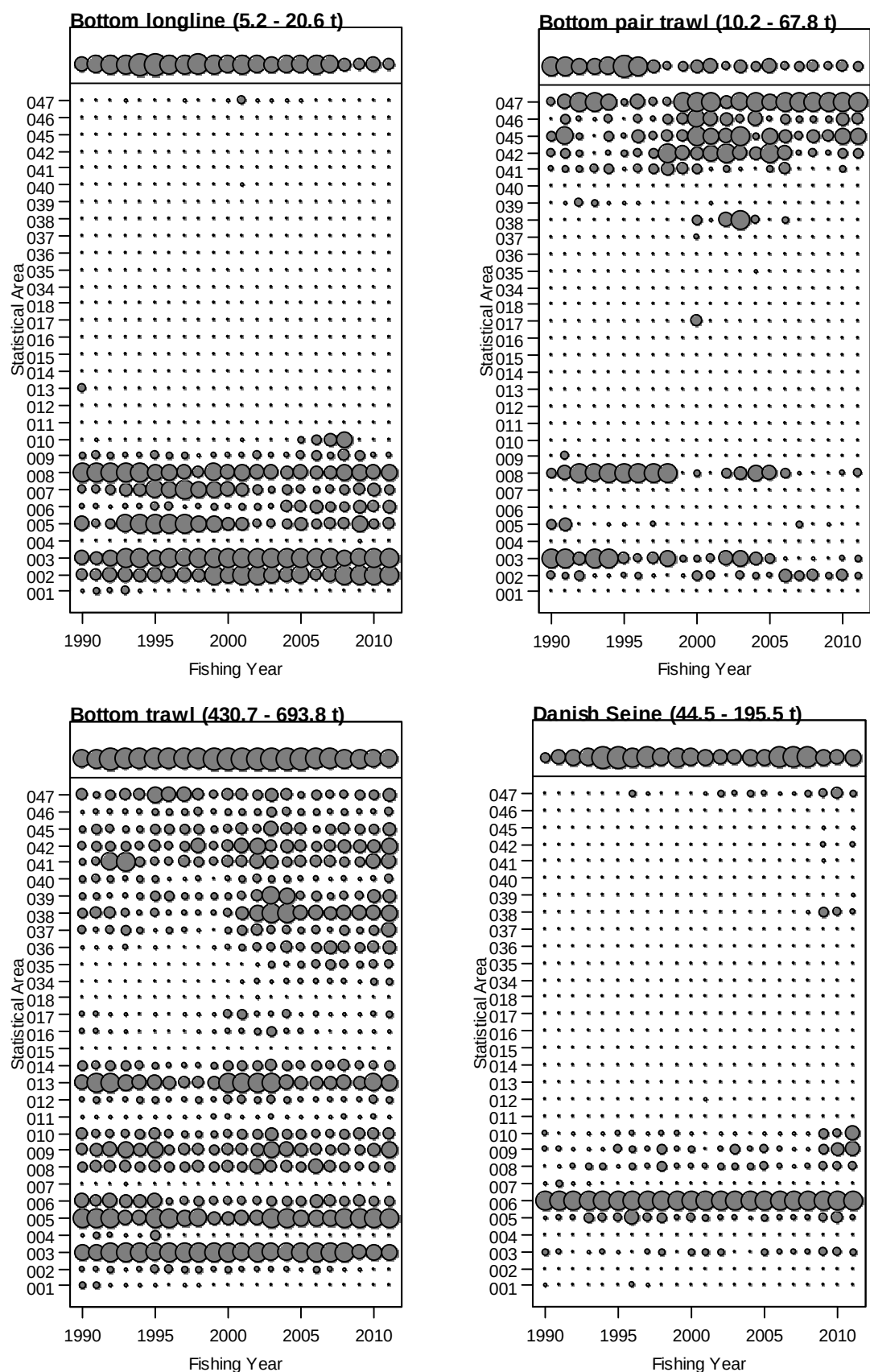
Figure 27: Bubble plots of John dory catch by method, statistical area, and fishing year. Bubble area is proportional to catch size. Catches by area are normalised within each year. The top panel shows the catch by year, with bubble sizes varying between the catch sizes shown in the title. Fishing year is labelled as the year ending.
