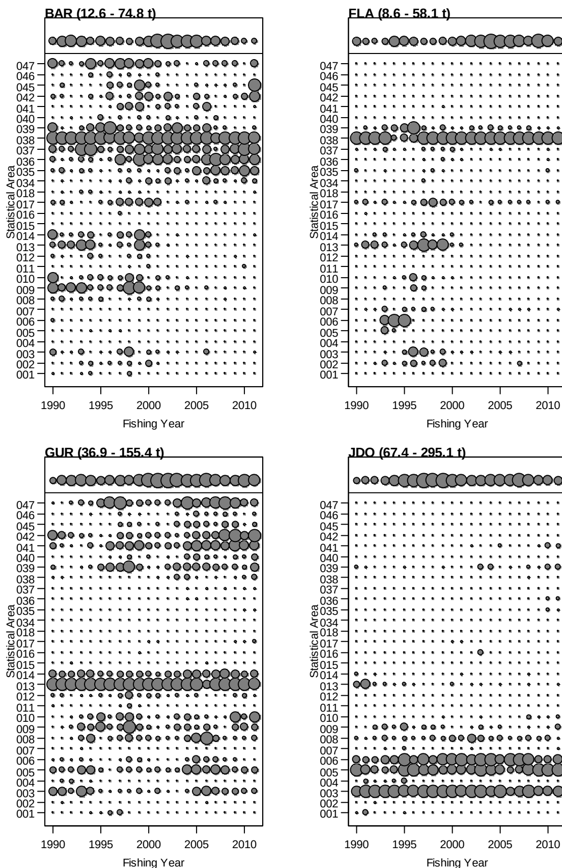
Figure 28: Bubble plots of John dory catch by target species, statistical area, and fishing year. Bubble area is proportional to catch size. Catches by area are normalised within each year. The top panel shows the catch by year, with bubble sizes varying between the catch sizes shown in the title. Fishing year is labelled as the year ending.
