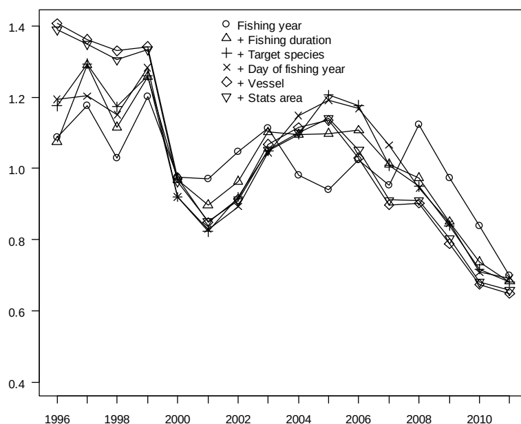
Figure A2.1: Annual CPUE indices for the Hauraki Gulf and east Northland stock normal model at each step in the variable selection process.
