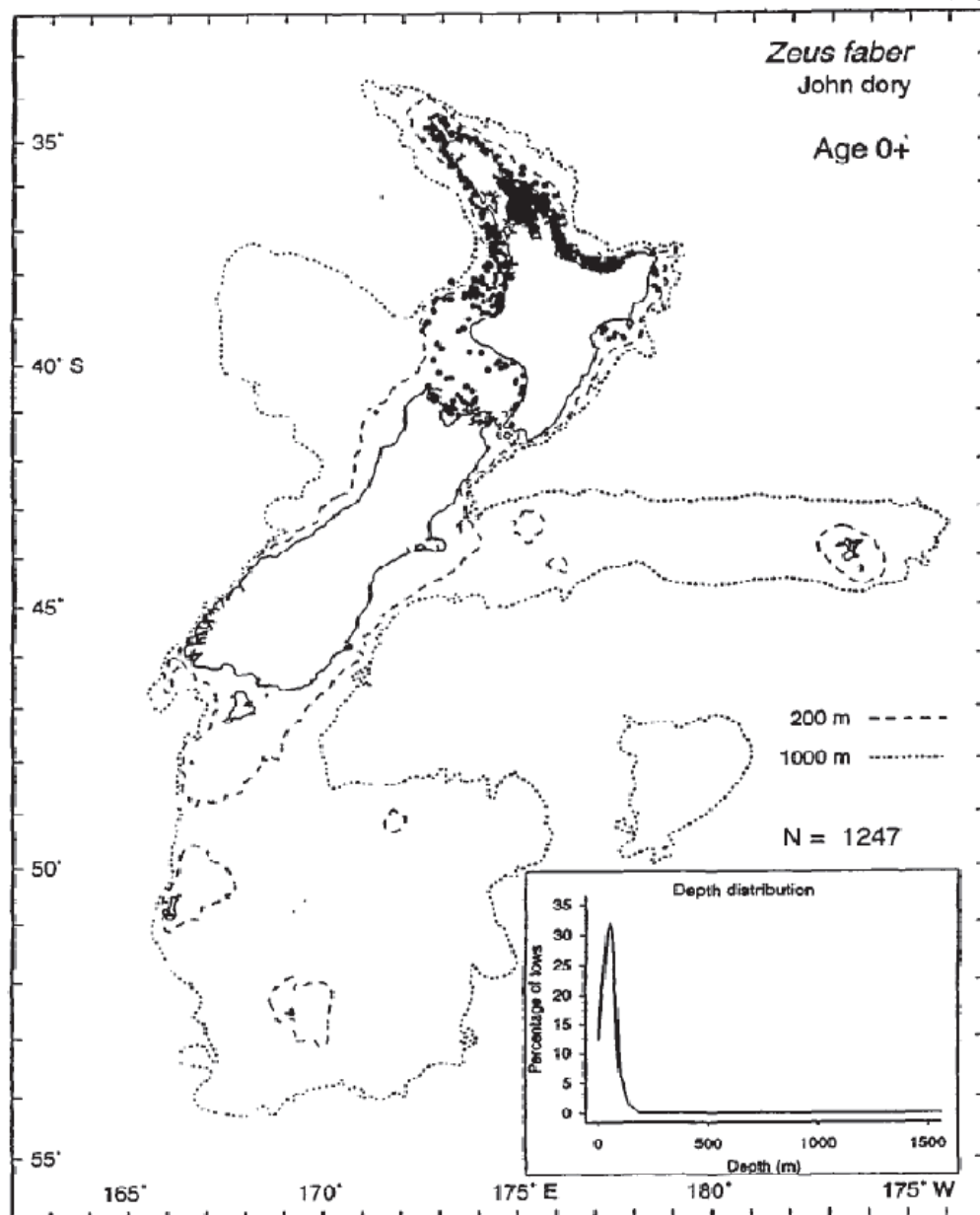
Figure 3: Observations of age 0 (0+ group) John dory (black dots). Reproduced from Hurst et al. (2000).
