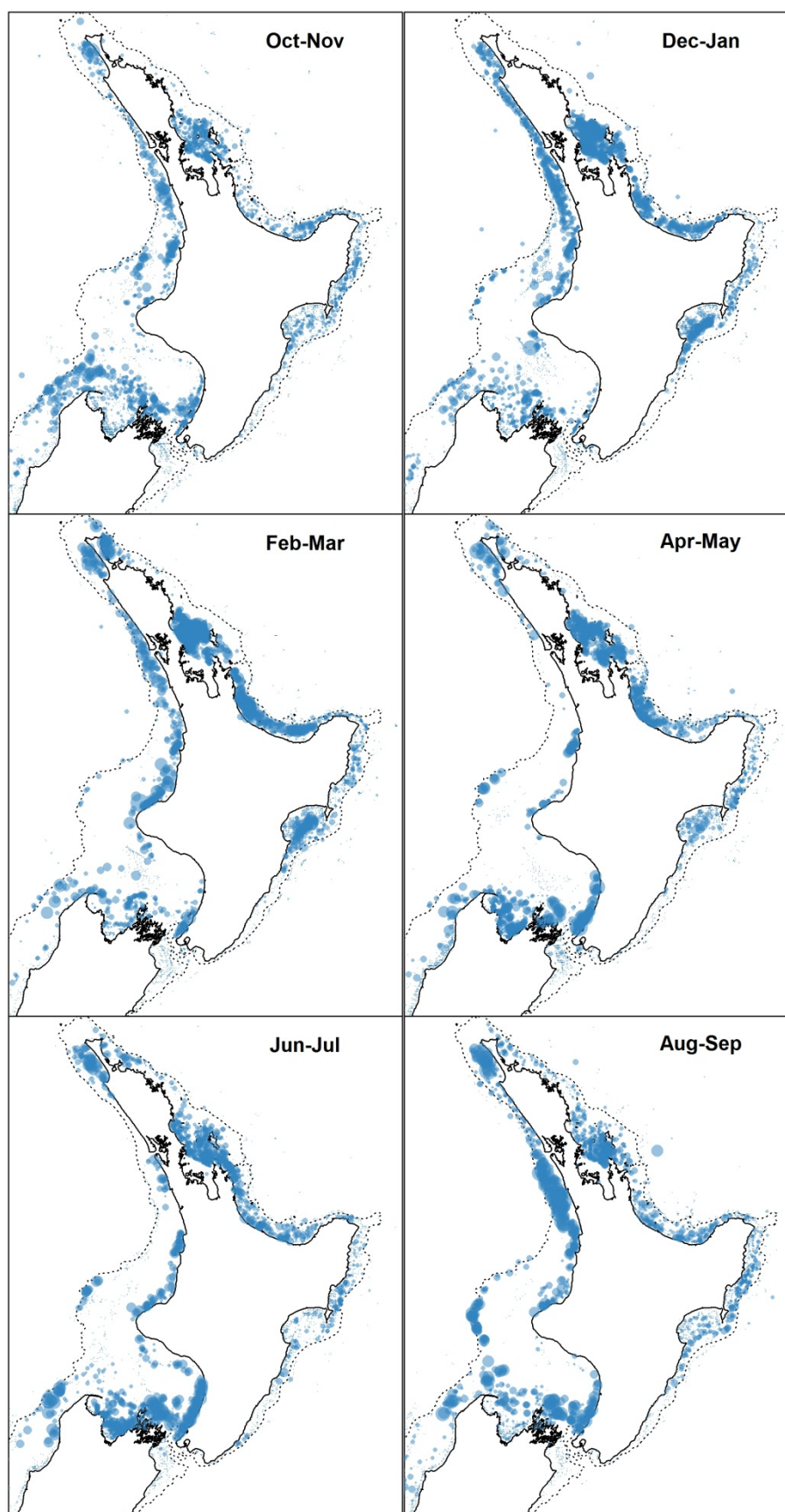
Figure 25: Catch of John dory per hour fished by bottom trawlers in 2010–11, by bi-monthly groups. Circle size is proportional to catch rate; the largest circle in each plot represents the largest catch rate in that two-month period. Dotted line, 200 m isobath.
