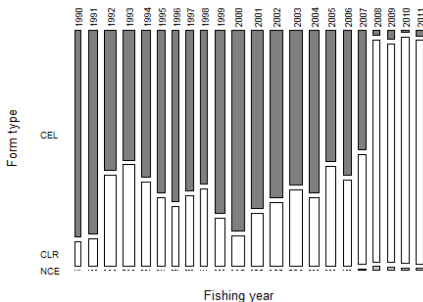
Figure A1.6: The proportion of reported landings of John dory by form type for JDO 2. Calculated from estimated greenweight. CEL, Catch Effort Landing Return; CLR, Catch Landing Return (for TCP and TCEPR forms); NCE, Netting Catch, Effort and Landing Return (for set nets, inshore drift nets, or pair set nets).
