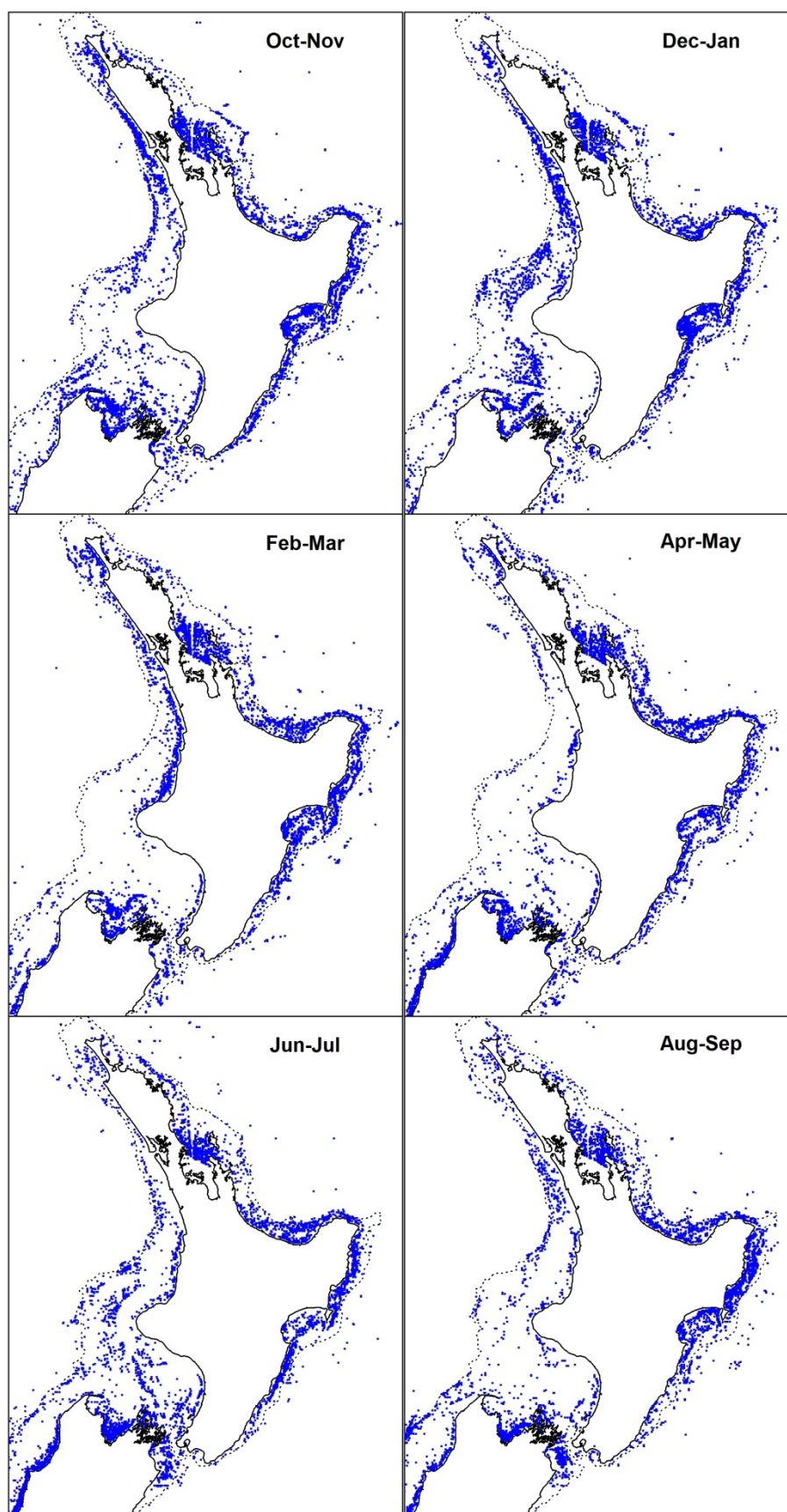
Figure 20: Location of bottom trawls from tow-by-tow data (points) in 2008–09, by bi-monthly groups.
