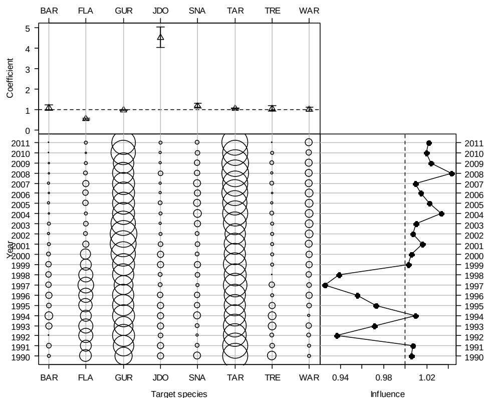
Figure A2.19: Effect and influence of target species in the Southeast North Island CPUE normal model. Top: relative effect by level of variable; Bottom-left, relative distribution of variables by fishing year; Bottom-right, influence of variable on unstandardized CPUE by fishing year.
