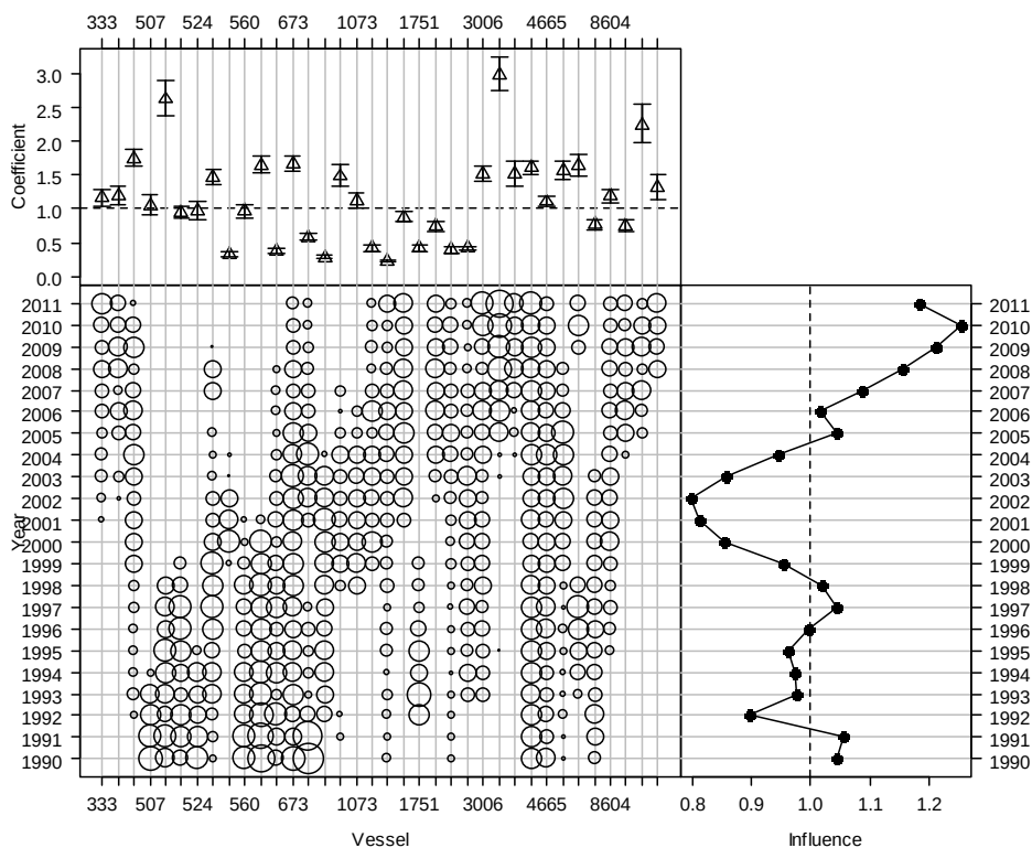
Figure A2.20: Effect and influence of vessel in the Southeast North Island CPUE normal model. Top: relative effect by level of variable; Bottom-left, relative distribution of variables by fishing year; Bottom-right, influence of variable on unstandardized CPUE by fishing year.
