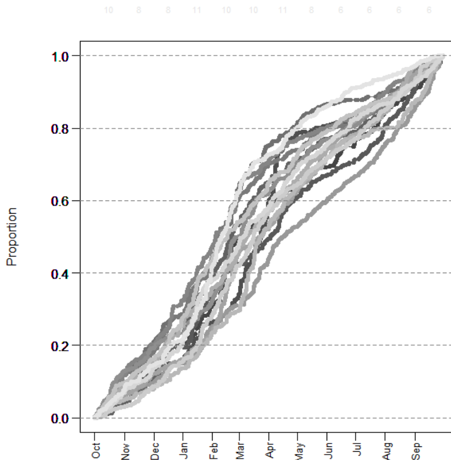
Figure 34: Cumulative catches of John dory in Bay of Plenty, by fishing year, by day of fishing year, after applying the target species and vessel selection criteria. Catches are summed in chronological order through the fishing year. Fishing years are shown by the degree of shading, with the earliest year in black (1995–96), through to the most recent year in light grey (2010–11).
