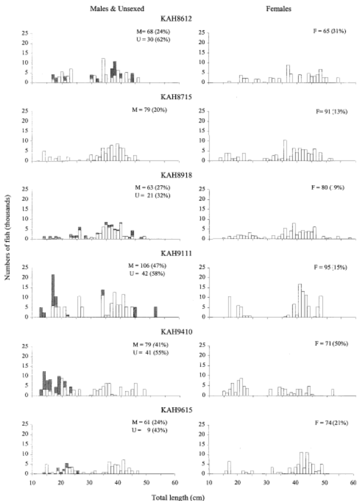
Figure 10: Scaled length frequency distributions for John dory sampled in the west coast North Island trawl survey (October–December), by year and sex. Reproduced from Morrison et al. (2001a).
