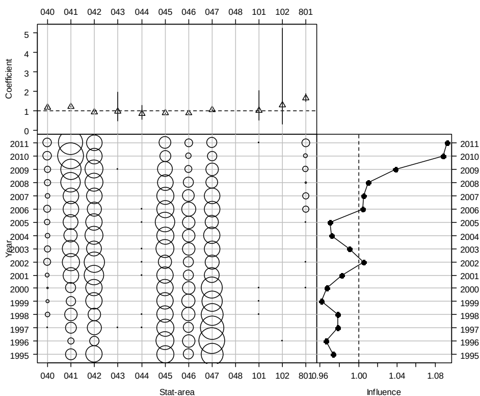
Figure A2.16: Effect and influence of statistical area in the West coast North Island CPUE normal model. Top: relative effect by level of variable; Bottom-left, relative distribution of variables by fishing year; Bottom-right, influence of variable on unstandardized CPUE by fishing year.
