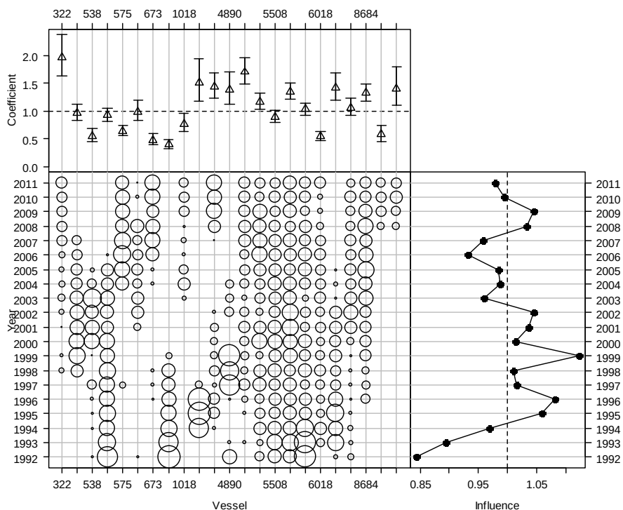
Figure A2.26: Effect and influence of vessel in the northern South Island CPUE normal model. Top: relative effect by level of variable; Bottom-left, relative distribution of variables by fishing year; Bottom-right, influence of variable on unstandardized CPUE by fishing year.
