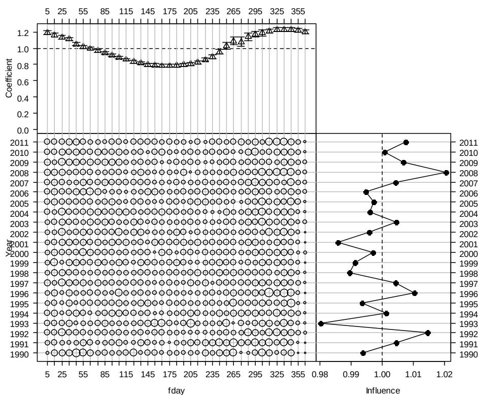
Figure A2.22: Effect and influence of day of the fishing year in the Southeast North Island CPUE normal model. Top: relative effect by level of variable; Bottom-left, relative distribution of variables by fishing year; Bottom-right, influence of variable on unstandardized CPUE by fishing year.
