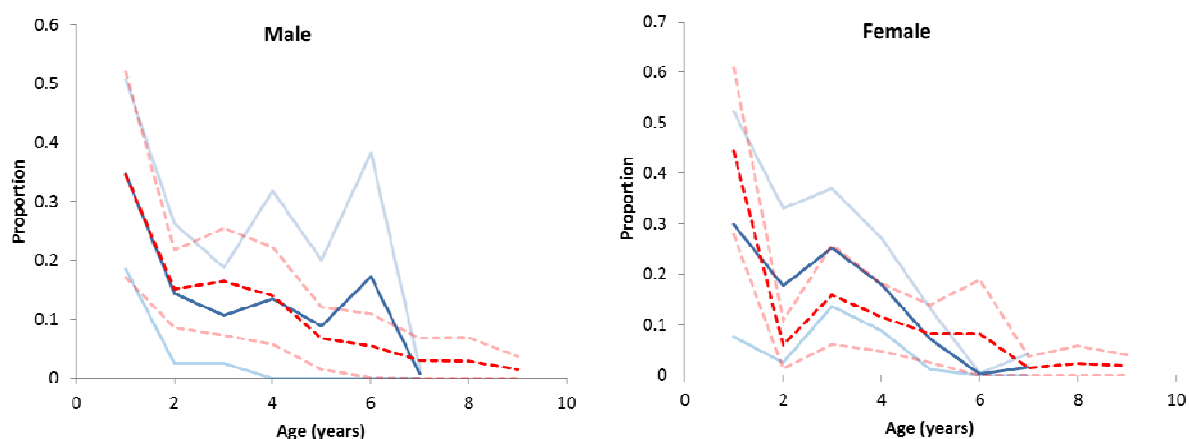
Figure 7: Estimated proportion at age (dark shaded lines) with 95% credible intervals (light shaded lines) for male and female John dory from the Hauraki Gulf (solid lines) and Bay of Plenty (broken lines). Estimates from Hanchet et al. (2001).
