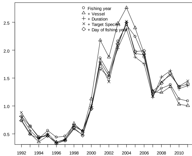
Figure A2.23: Annual CPUE indices for the Northern South Island stock normal model at each step in the variable selection process.
