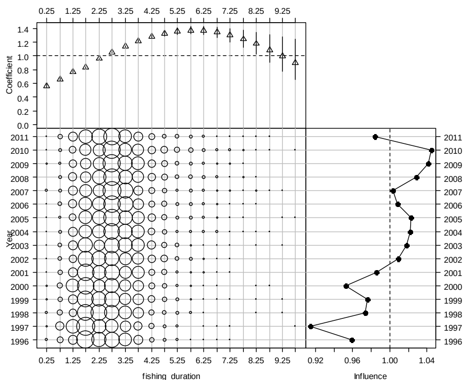
Figure A2.9: Effect and influence of fishing duration in the Bay of Plenty CPUE normal model. Top: relative effect by level of variable; Bottom-left, relative distribution of variables by fishing year; Bottom-right, influence of variable on unstandardized CPUE by fishing year.
