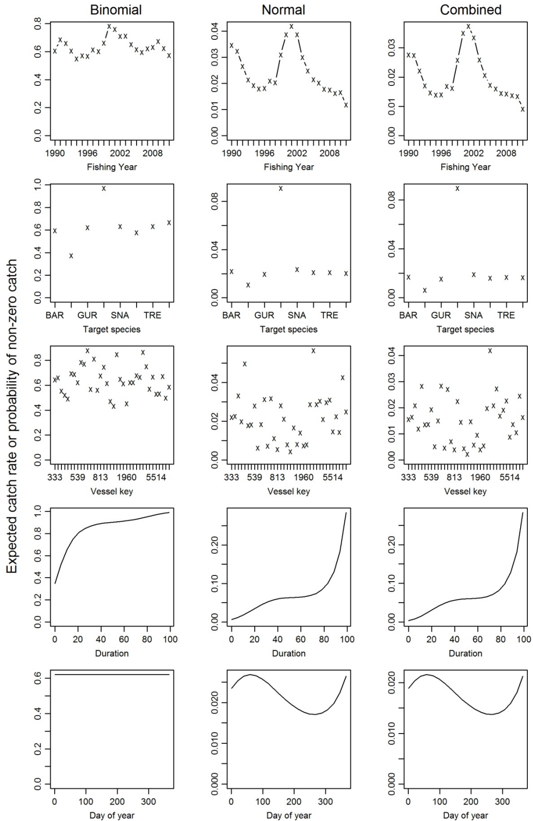
Figure 44: Model predictions for the Southeast North Island index, by fishing year (labelled as year ending, i.e., 1991 means 1990–91) and other selected predictors, for the binomial, normal and combined model, made with all other predictors set to the median (fixed) values. The target species are labelled in ascending alphabetical order; John dory is between the GUR and SNA labels.
