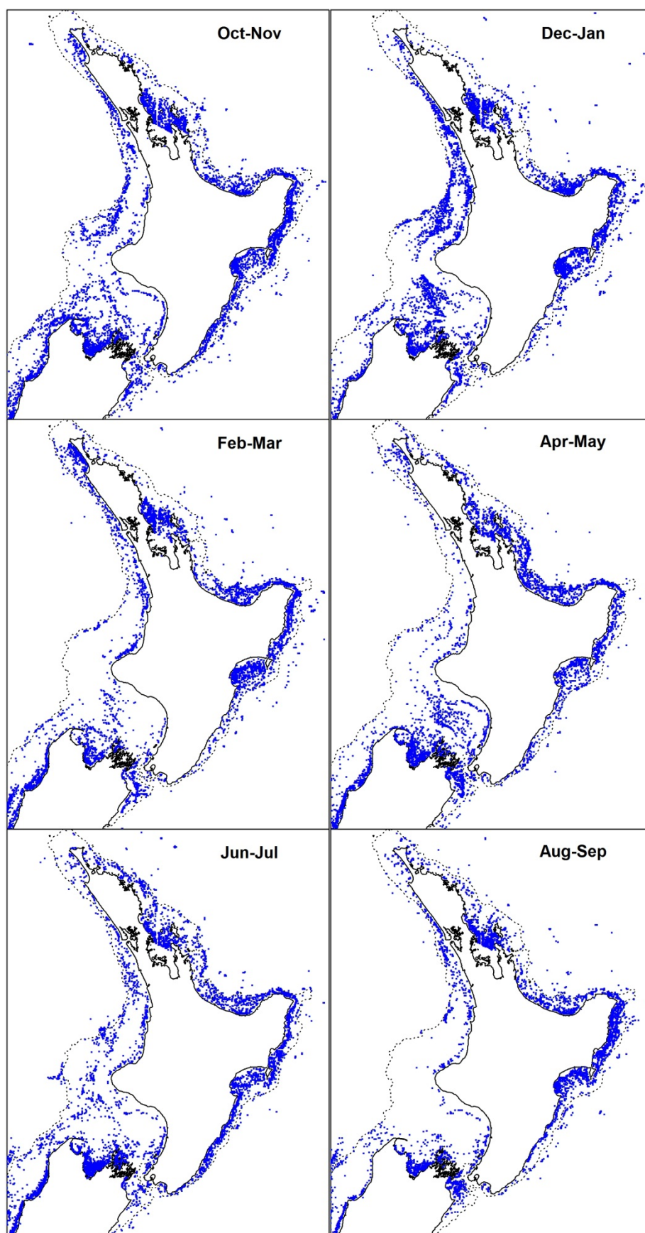
Figure 22: Location of bottom trawls from tow-by-tow data (points) in 2009–10, by bi-monthly groups.
