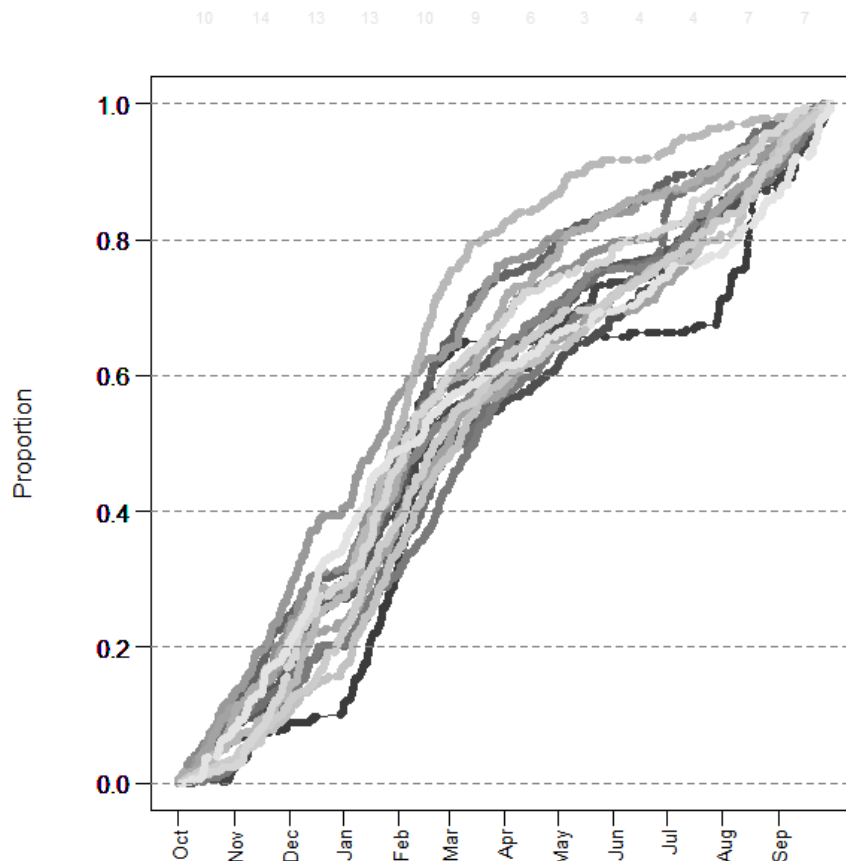
Figure 38: Cumulative catches of John dory in West Coast North Island, by fishing year, by day of fishing year, after applying the target species and vessel selection criteria. Catches are summed in chronological order through the fishing year. Fishing years are shown by the degree of shading, with the earliest year in black (1994–95), through to the most recent year in light grey (2010–11).
