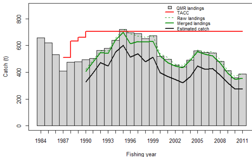
Figure A1.1: John dory official (Quota Management Reports: QMR) landings and TACC, and the raw, merged, and estimated catches in the catch-effort dataset, for JDO1.
