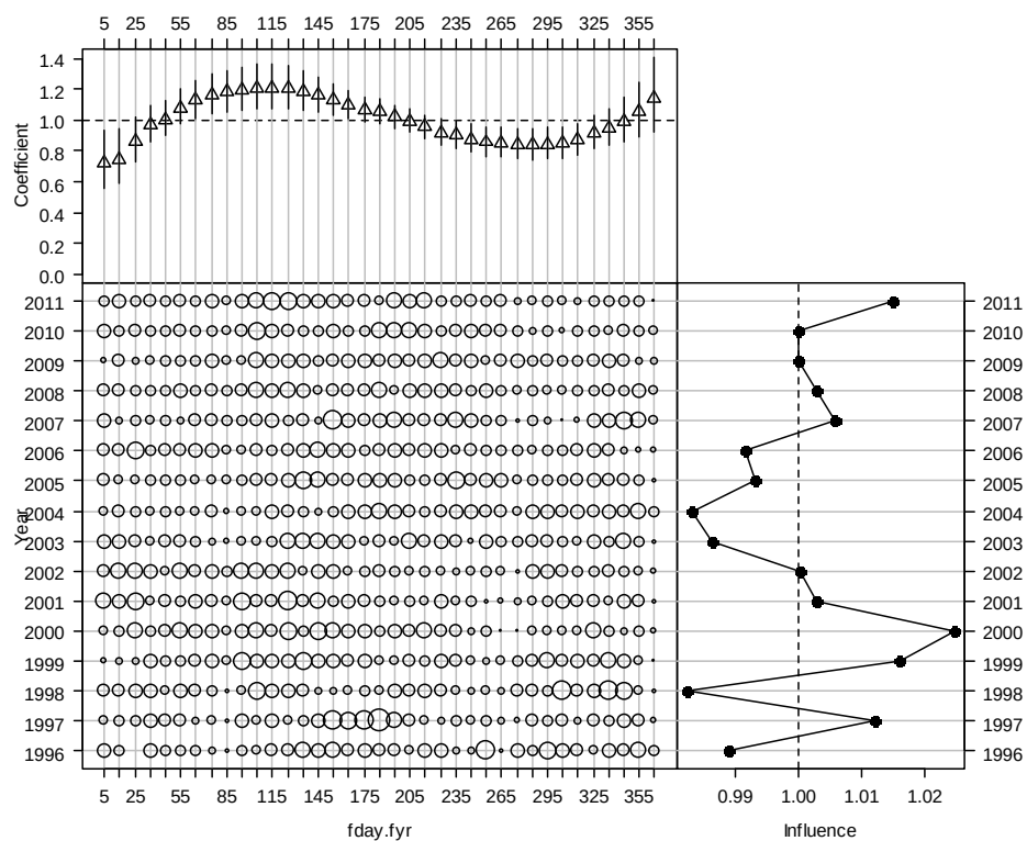
Figure A2.10: Effect and influence of fishing day (labelled here as fday.fyr: day of the fishing year) in the Bay of Plenty CPUE normal model. Top: relative effect by level of variable; Bottom-left, relative distribution of variables by fishing year; Bottom-right, influence of variable on unstandardized CPUE by fishing year.
