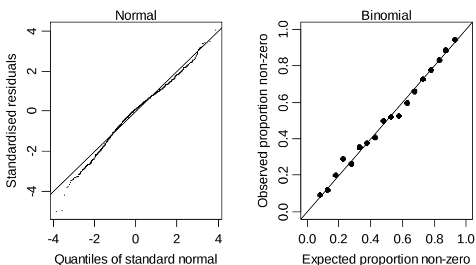
Figure 47: Q-Q plots for the fit of the Northern South Island index.
