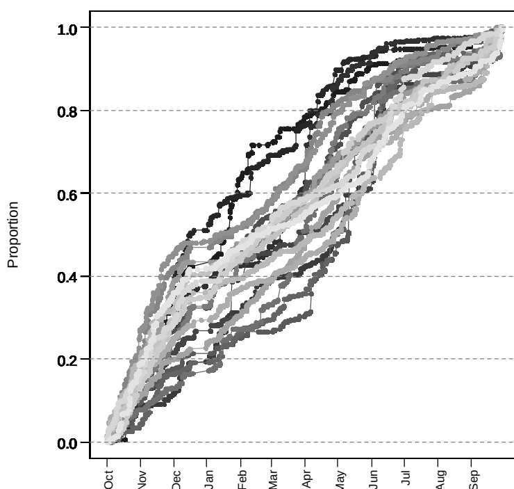
Figure 46: Cumulative catches of John dory in Northern South Island, by fishing year, by day of fishing year, after applying the target species and vessel selection criteria. Catches are summed in chronological order through the fishing year. Fishing years are shown by the degree of shading, with the earliest year in dark grey (1991–92), through to the most recent year in light grey (2010–11).
