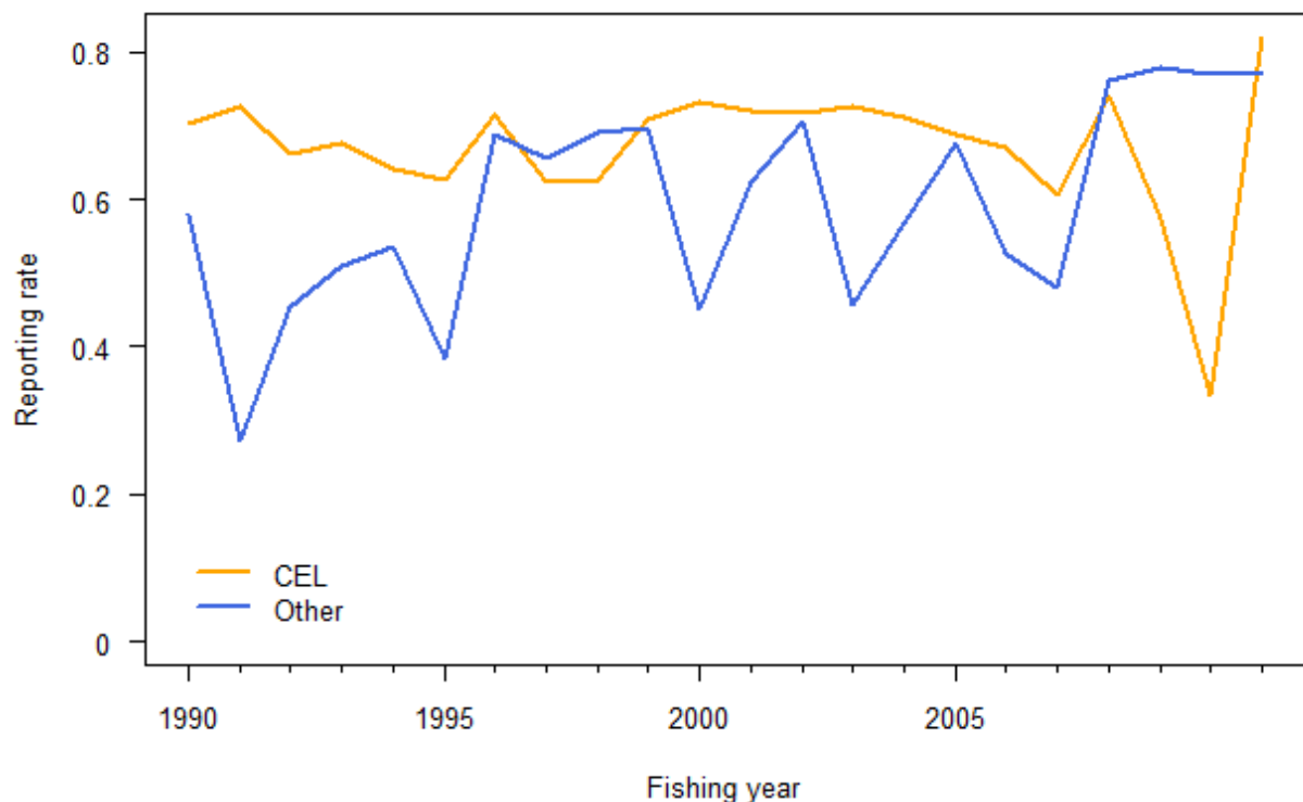
Figure A1.8: The reporting rate of John dory by form type for JDO 2. CEL, Catch Effort Landing Return. The reporting rate is the estimated catch divided by the trip-stratum (i.e., QMR) catch.
