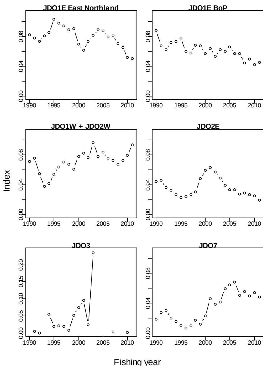
Figure 26: CPUE trends by fishstock estimated by GLM model 6 (see Table 4).
