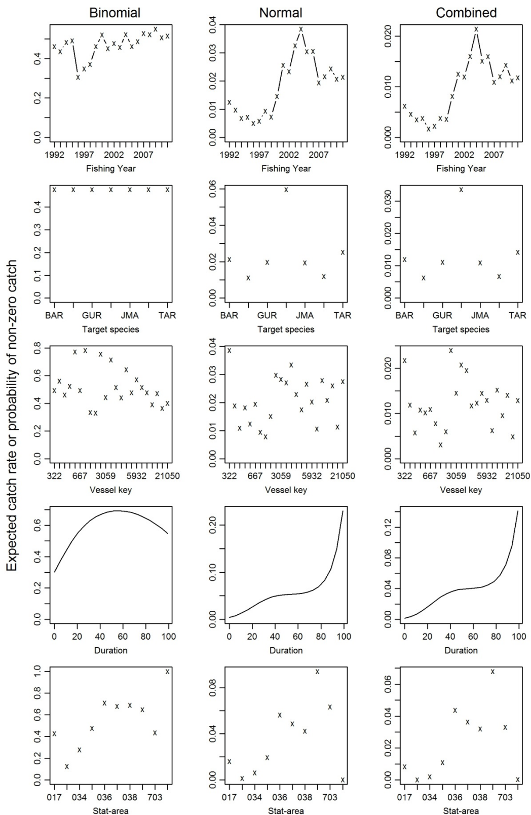
Figure 48: Model predictions for the northern South Island index, by fishing year (labelled as year ending, i.e., 1995 means 1994–95) and other selected predictors, for the binomial, normal and combined model, made with all other predictors set to the median (fixed) values. The target species are labelled in ascending alphabetical order; John dory is between the GUR and JMA labels.
