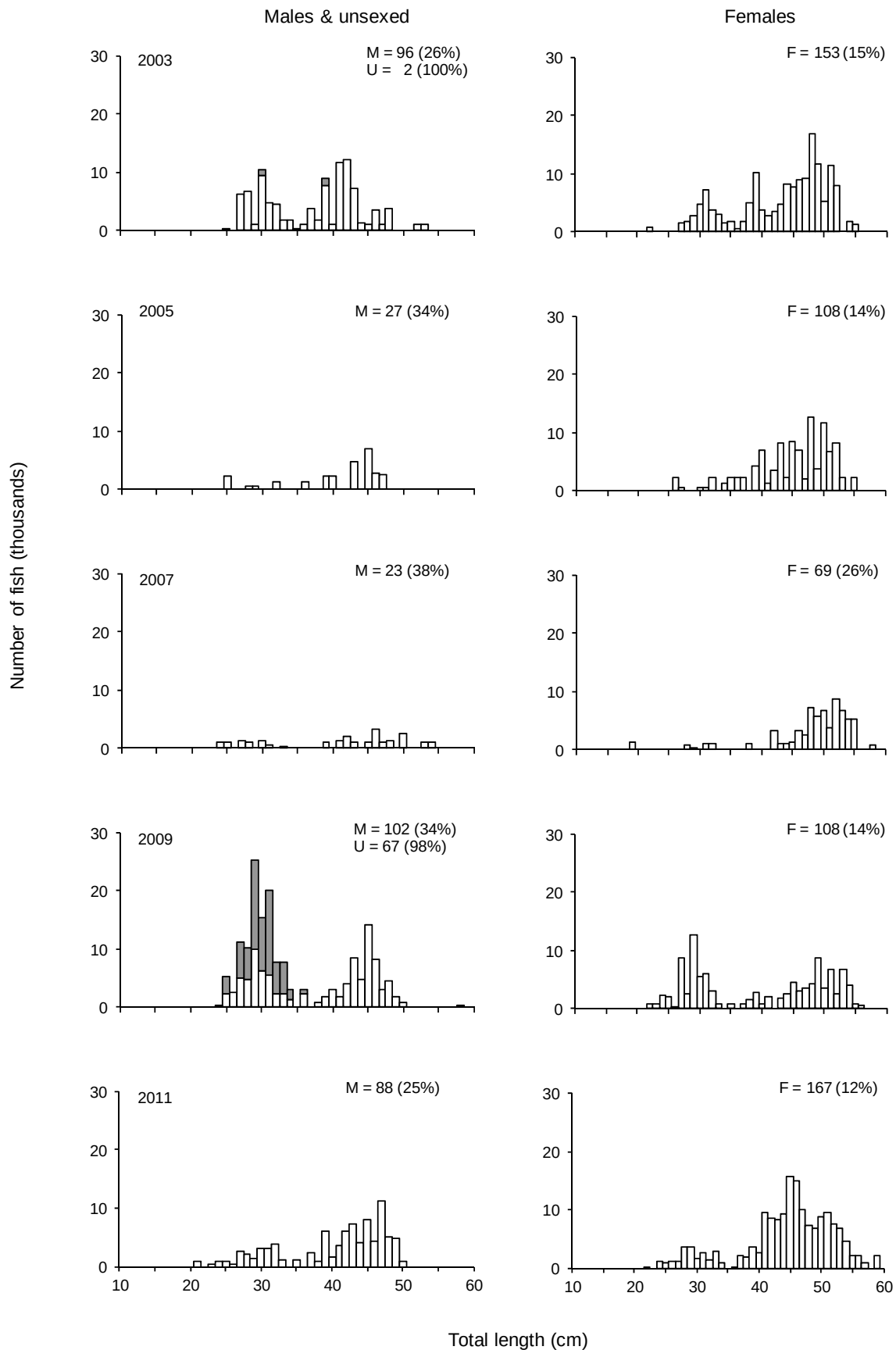
Figure 9(cont.): Scaled length frequency distributions for John dory sampled in the west coast South Island trawl survey (February–March), by year and sex (Stevenson, per.comm.).
