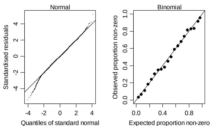
Figure 35: Q–Q plots for the fit of the Bay of Plenty index.
