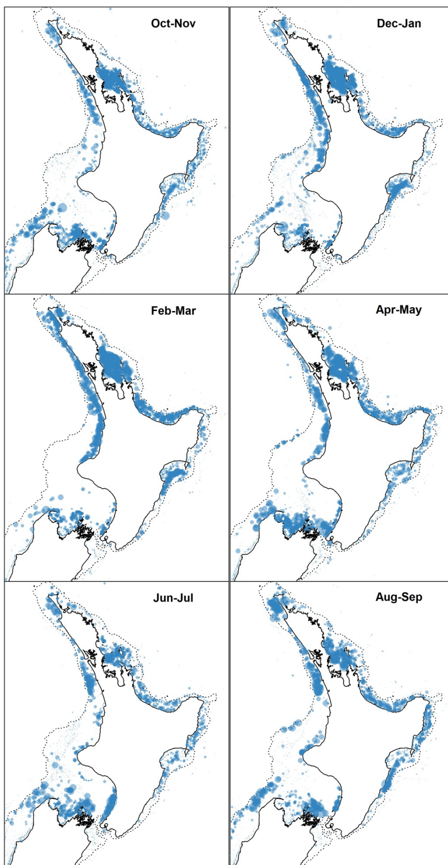
Figure 19: Catch of John dory per hour fished by bottom trawlers in 2007–08, by bi-monthly groups. Circle size is proportional to catch rate; the largest circle in each plot represents the largest catch rate in that two-month period. Dotted line, 200 m isobath.
