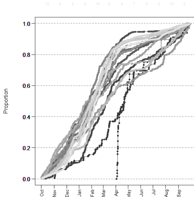
Figure 30: Cumulative catches of John dory in Hauraki Gulf and east Northland, by fishing year, by day of fishing year, after applying the target species and vessel selection criteria. Catches are summed in chronological order through the fishing year. Fishing years are shown by the degree of shading, with the earliest year in black (1993–94), through to the most recent year in light grey (2010–11)
