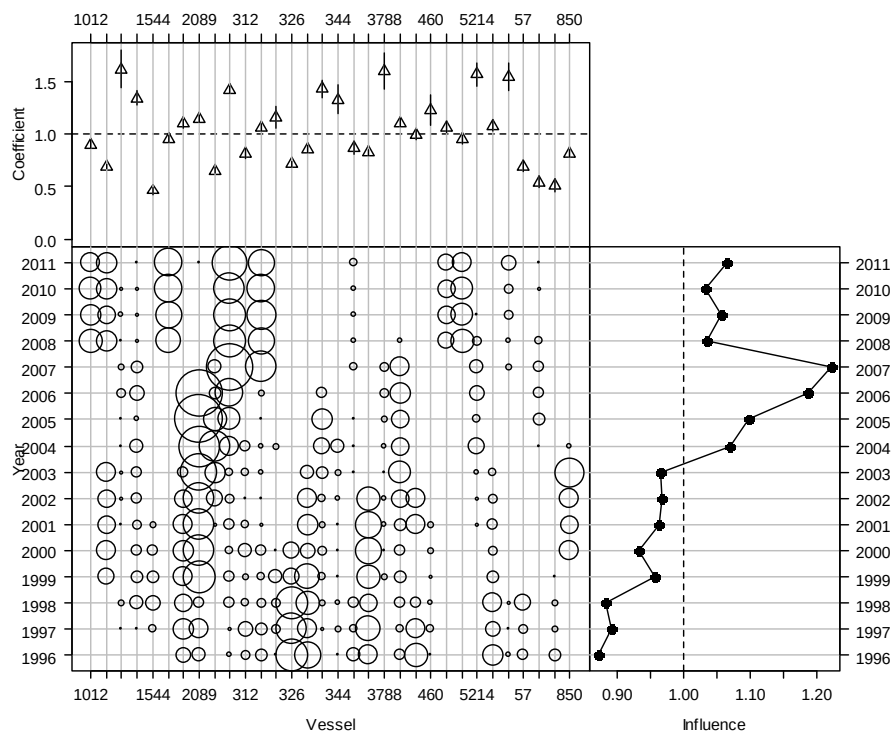
Figure A2.3: Effect and influence of vessel in the Hauraki Gulf and east Northland CPUE normal model. Top: relative effect by level of variable; Bottom left, relative distribution of variables by fishing year; Bottom right, influence of variable on unstandardized CPUE by fishing year.
