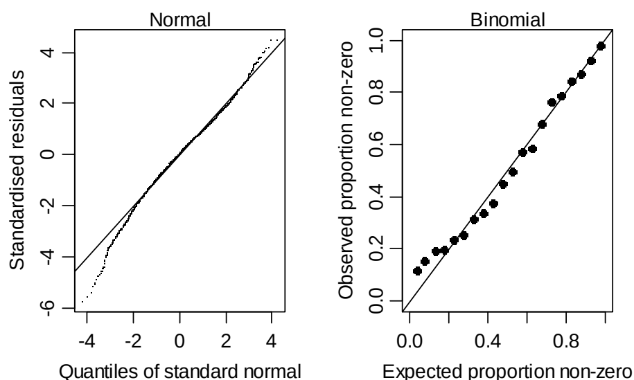
Figure 31: Q-Q plots for the fit of the Hauraki Gulf and east Northland index.
