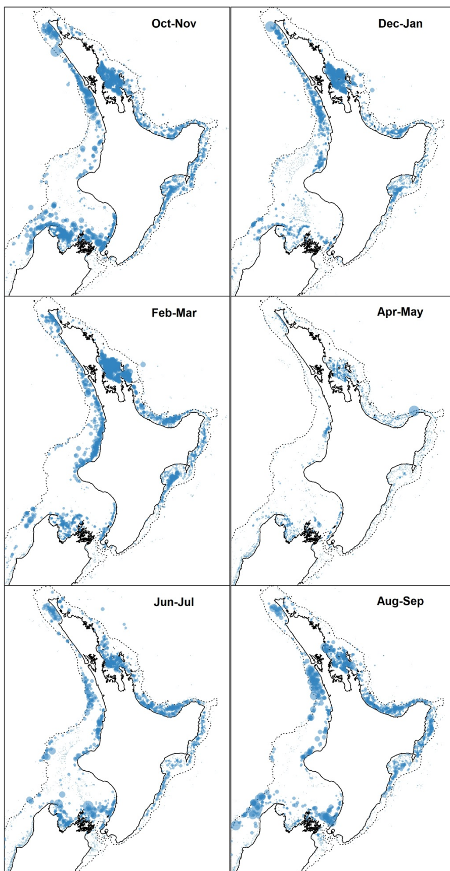
Figure 21: Catch of John dory per hour fished by bottom trawlers in 2008–09, by bi-monthly groups. Circle size is proportional to catch rate; the largest circle in each plot represents the largest catch rate in that two-month period. Dotted line, 200 m isobath.
