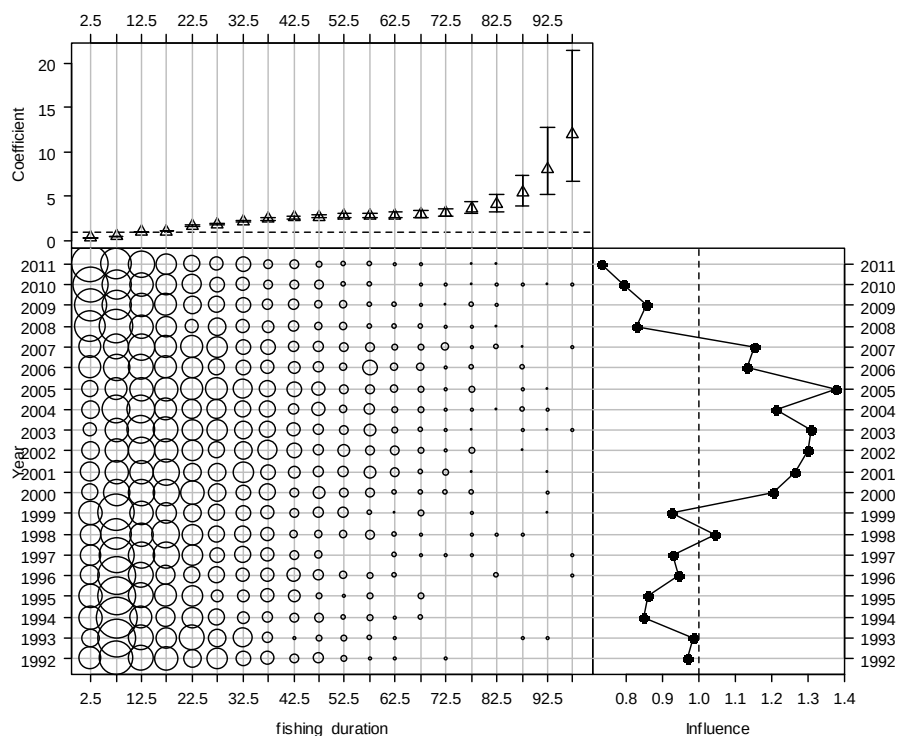
Figure A2.25: Effect and influence of fishing duration in the northern South Island CPUE normal model. Top: relative effect by level of variable; Bottom-left, relative distribution of variables by fishing year; Bottom-right, influence of variable on unstandardized CPUE by fishing year.
