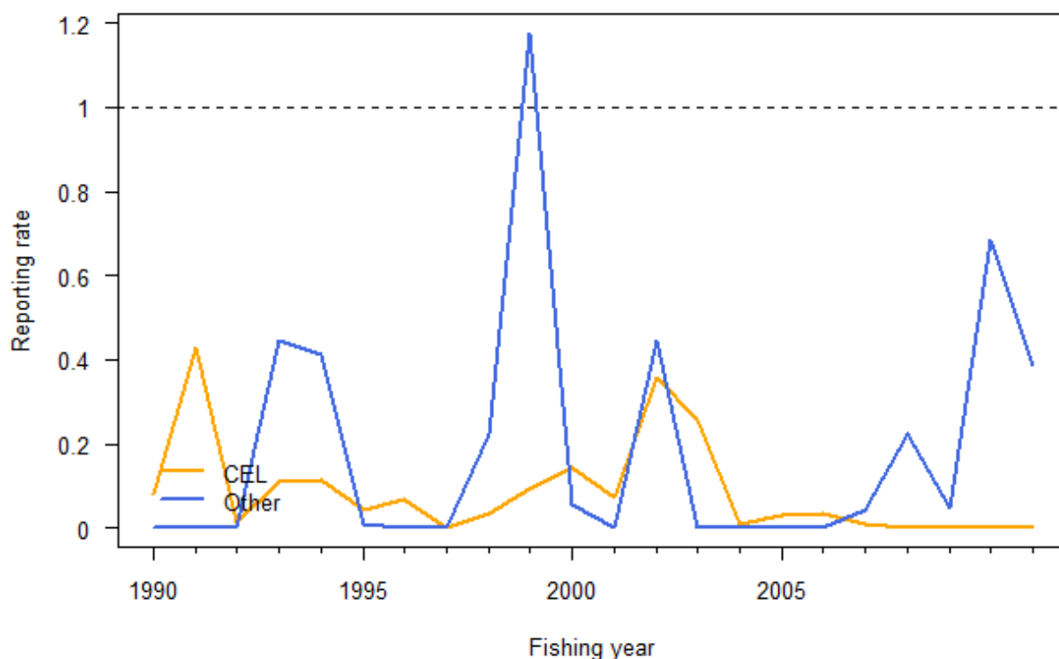
Figure A1.12: The reporting rate of John dory by form type for JDO 1. CEL, Catch Effort Landing Return. The reporting rate is the estimated catch divided by the trip-stratum (i.e., QMR) catch.
