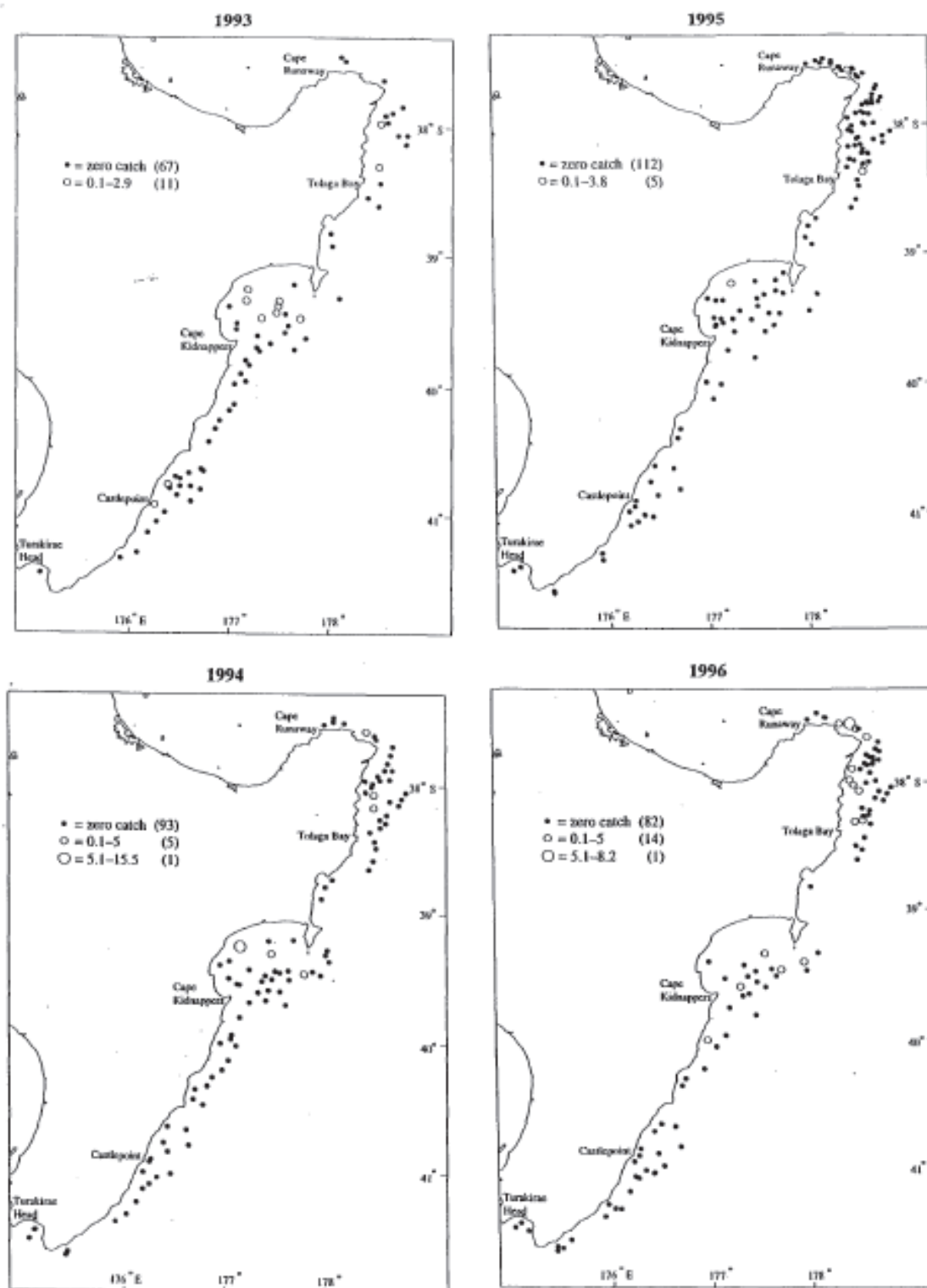
Figure 12: Research trawl catch rates of juvenile John dory during the east coast North Island trawl surveys, combined sexes, by year. Plotted circles are proportional to catch rate, which is \text{kg km}^{-1} . Juveniles were defined as John dory less than 34 cm total length. Numbers in parentheses give the number of stations within the given catch rate range. The years were selected at random from the trawl survey series. Reproduced from Stevenson (1998).
