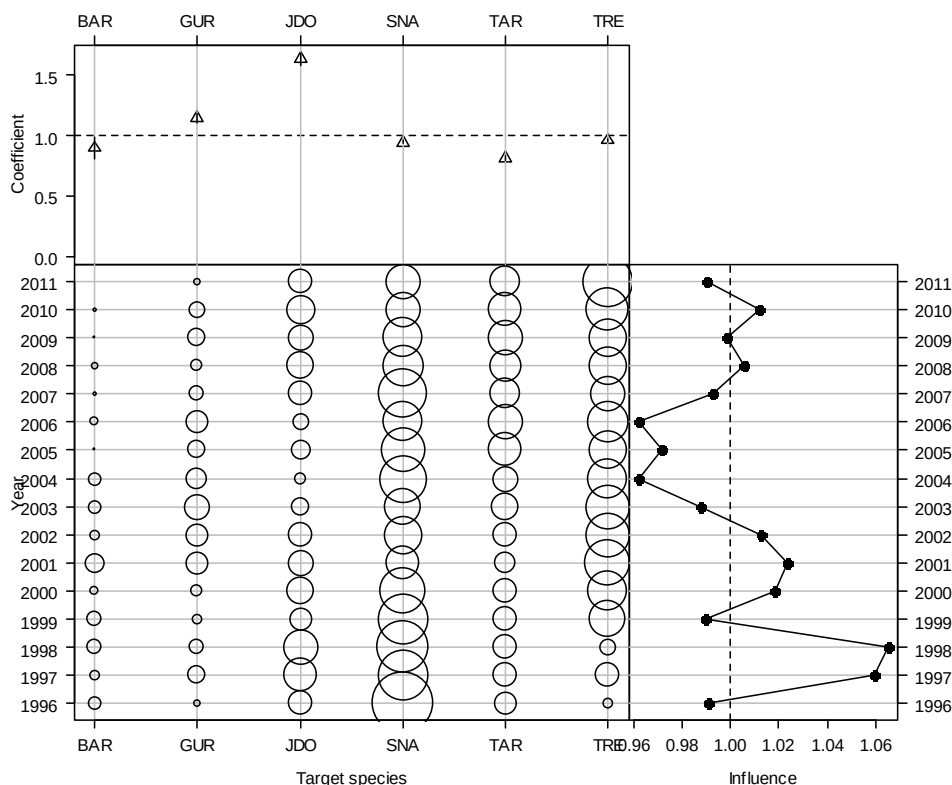
Figure A2.7: Effect and influence of target species in the Bay of Plenty CPUE normal model. Top: relative effect by level of variable; Bottom-left, relative distribution of variables by fishing year; Bottom-right, influence of variable on unstandardized CPUE by fishing year.
