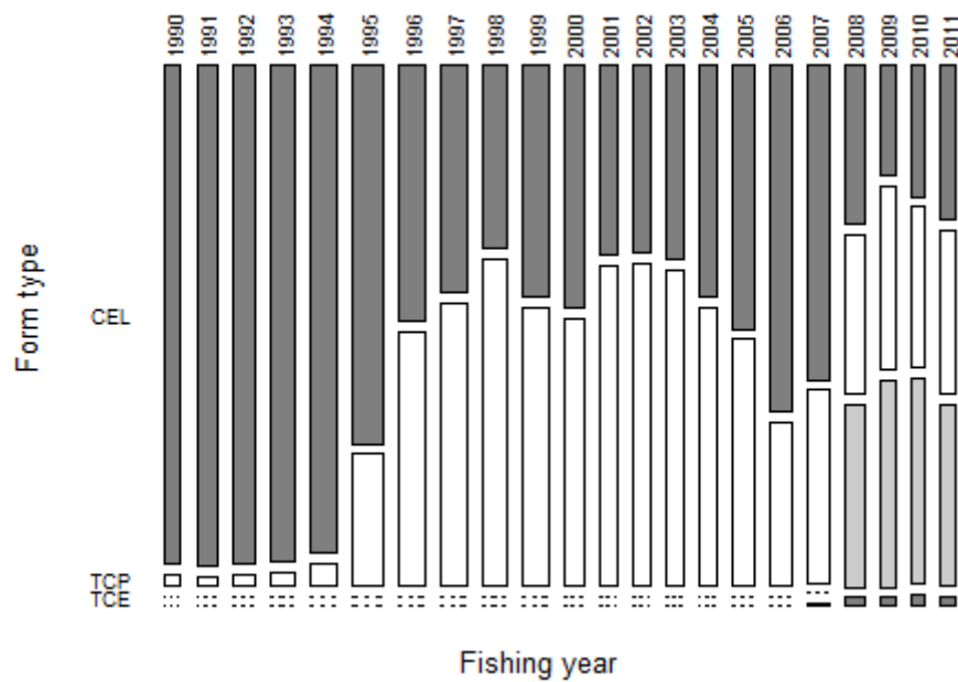
Figure A1.3: The proportion of estimated catches of John dory by form type for JDO 1. CEL, Catch Effort Landing Return; TCP, – Trawl Catch Effort Processing Return (for vessels >28 m in length); TCE, Trawl Catch Effort Return (for vessels 6–28 m in length).
