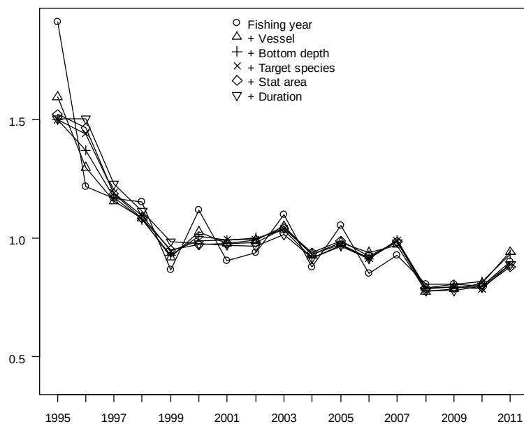
Figure A2.12: Annual CPUE indices for the West coast North Island stock normal model at each step in the variable selection process.
