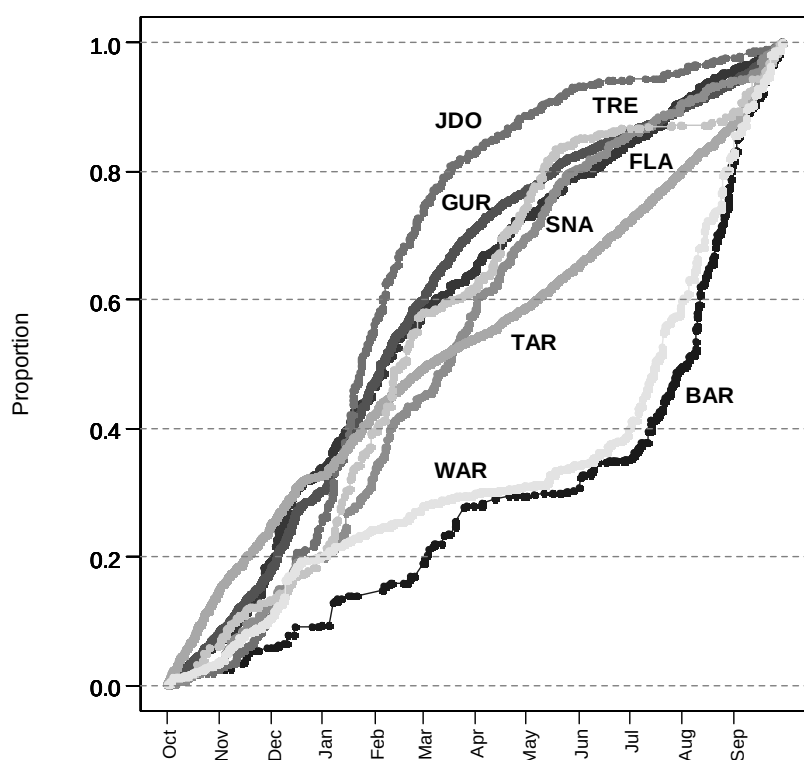
Figure 41: Cumulative catches of John dory in Southeast North Island, by target species, by day of fishing year and for 1989–90 to 2010–11, after applying the target species and vessel selection criteria. Catches are summed in chronological order through the fishing year.
