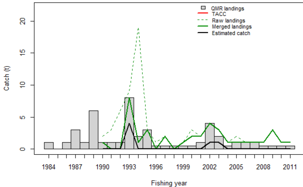
Figure A1.9: John dory official (Quota Management Reports: QMR) landings and TACC, and the raw, merged, and estimated catches in the catch-effort dataset, for JDO3.
