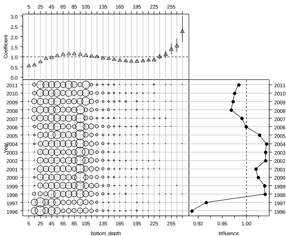
Figure A2.11: Effect and influence of bottom depth in the Bay of Plenty CPUE normal model. Top: relative effect by level of variable; Bottom-left, relative distribution of variables by fishing year; Bottom-right, influence of variable on unstandardized CPUE by fishing year.
