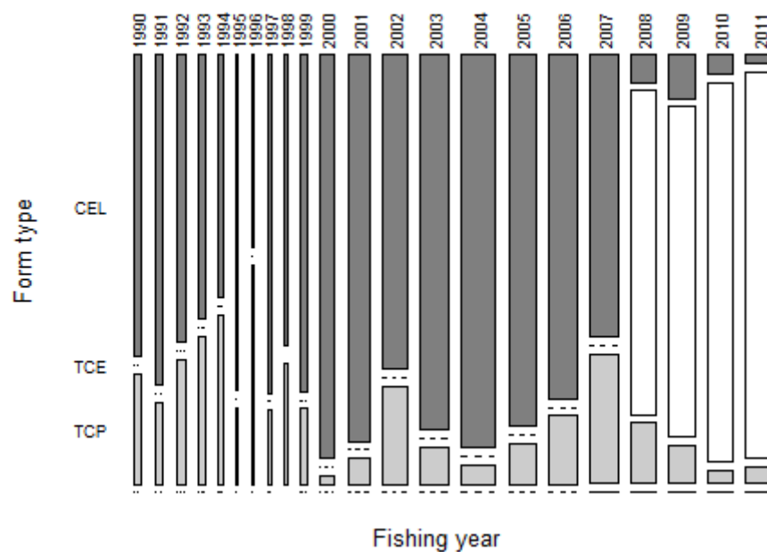
Figure A1.15: The proportion of estimated catches of John dory by form type for JDO 7. CEL, Catch Effort Landing Return; TCP, – Trawl Catch Effort Processing Return (for vessels >28 m in length); TCE, Trawl Catch Effort Return (for vessels 6–28 m in length).
