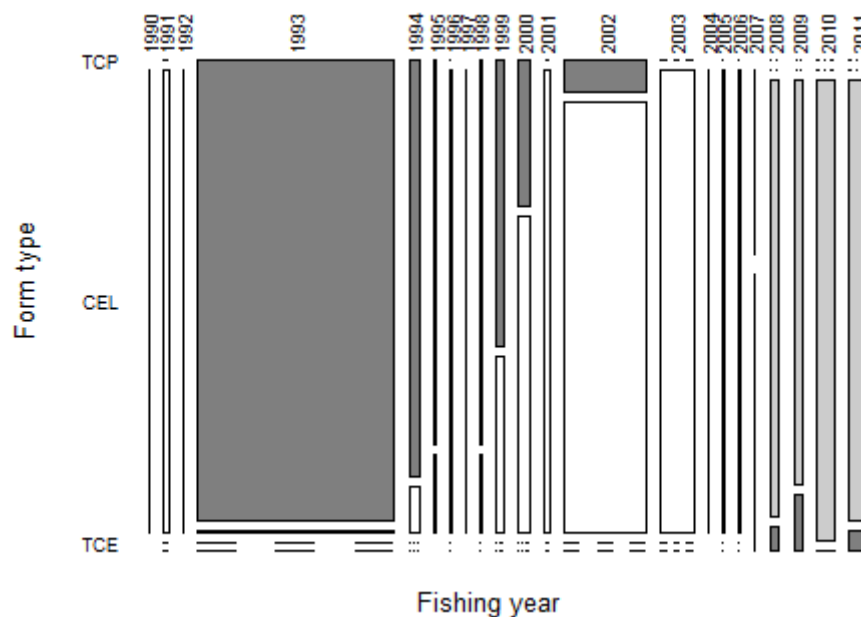
Figure A1.11: The proportion of estimated catches of John dory by form type for JDO 3. CEL, Catch Effort Landing Return; TCP, – Trawl Catch Effort Processing Return (for vessels >28 m in length); TCE, Trawl Catch Effort Return (for vessels 6–28 m in length).
