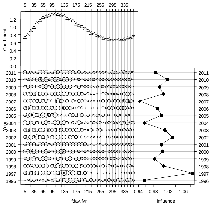
Figure A2.5: Effect and influence of fishing day (labelled here as fday.fyr: day of the fishing year) in the Hauraki Gulf and east Northland CPUE normal model. Top: relative effect by level of variable; Bottom left, relative distribution of variables by fishing year; Bottom right, influence of variable on unstandardized CPUE by fishing year.
