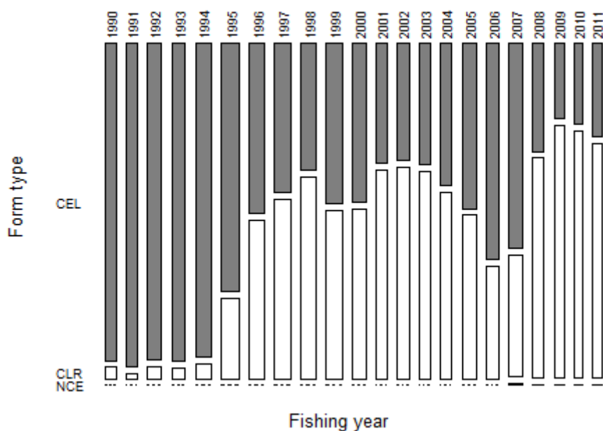
Figure A1.2: The proportion of reported landings of John dory by form type for JDO 1. Calculated from estimated greenweight. CEL, Catch Effort Landing Return; CLR, Catch Landing Return (for TCP and TCEPR forms); NCE, Netting Catch, Effort and Landing Return (for set nets, inshore drift nets, or pair set nets).
