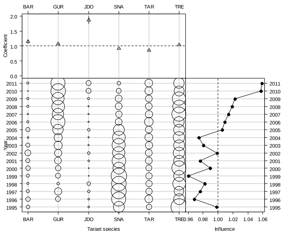
Figure A2.13: Effect and influence of target species in the West coast North Island CPUE normal model. Top: relative effect by level of variable; Bottom-left, relative distribution of variables by fishing year; Bottom-right, influence of variable on unstandardized CPUE by fishing year.
