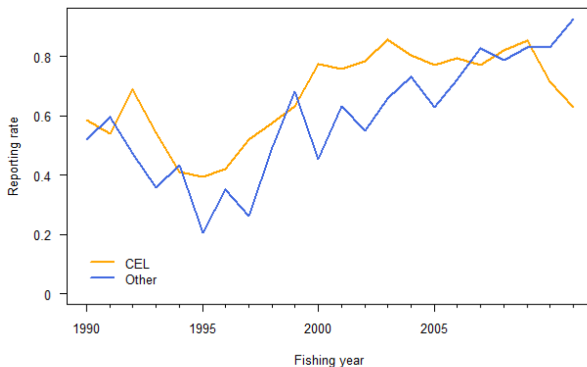
Figure A1.16: The reporting rate of John dory by form type for JDO 7. CEL, Catch Effort Landing Return. The reporting rate is the estimated catch divided by the trip-stratum (i.e., QMR) catch.
