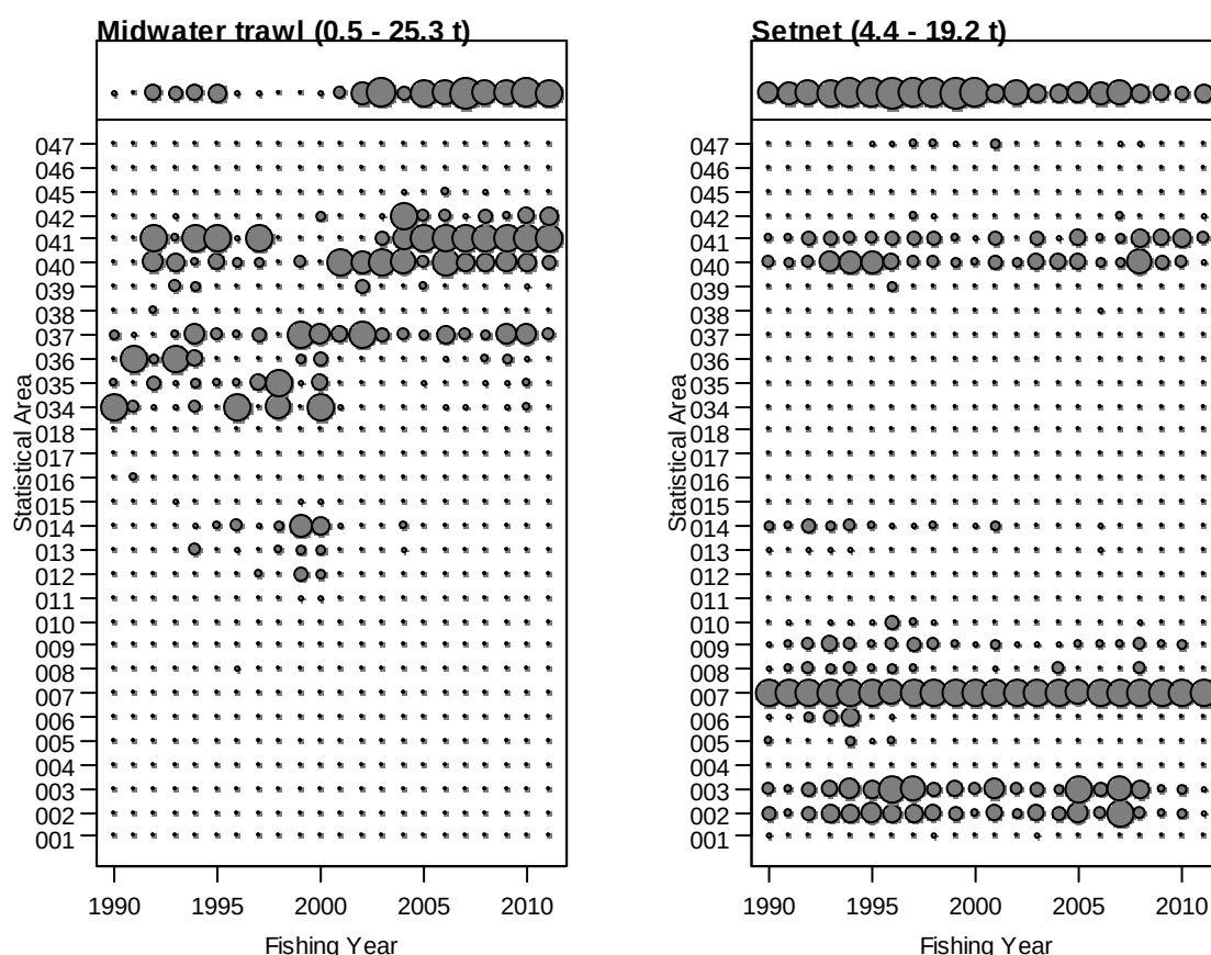
Figure 27 (cont.): Bubble plots of John dory catch by method, statistical area, and fishing year. Bubble area is proportional to catch size. Catches by area are normalised within each year. The top panel shows the catch by year, with bubble sizes varying between the catch sizes shown in the title. Fishing year is labelled as the year ending.
