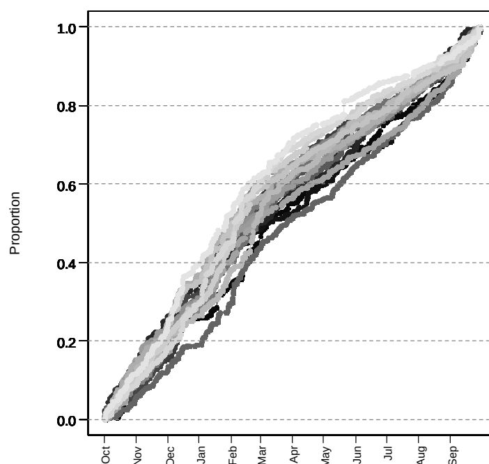
Figure 42: Cumulative catches of John dory in Southeast North Island, by fishing year, by day of fishing year, after applying the target species and vessel selection criteria. Catches are summed in chronological order through the fishing year. Fishing years are shown by the degree of shading, with the earliest year in black (1989–90), through to the most recent year in light grey (2010–11).
