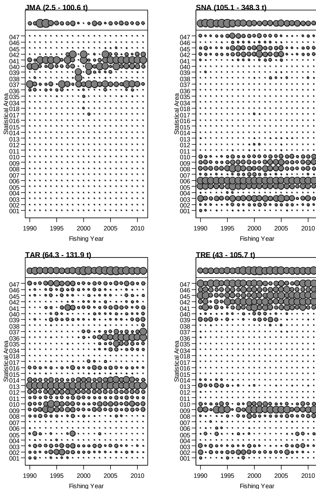
Figure 28 (cont.): Bubble plots of John dory catch by target species, statistical area, and fishing year. Bubble area is proportional to catch size. Catches by area are normalised within each year. The top panel shows the catch by year, with bubble sizes varying between the catch sizes shown in the title. Fishing year is labelled as the year ending.
