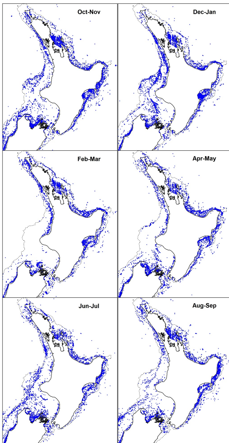
Figure 18: Location of bottom trawls from tow-by-tow data (points) in 2007–08, by bi-monthly groups.
