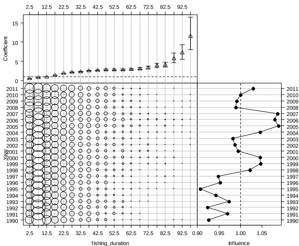
Figure A2.21: Effect and influence of fishing duration in the Southeast North Island CPUE normal model. Top: relative effect by level of variable; Bottom-left, relative distribution of variables by fishing year; Bottom-right, influence of variable on unstandardized CPUE by fishing year.
