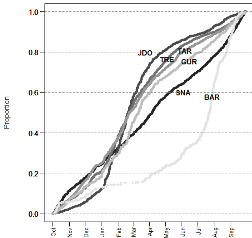
Figure 33: Cumulative catches of John dory in Bay of Plenty, by target species, by day of fishing year and for 1995–96 to 2010–11, after applying the target species and vessel selection criteria. Catches are summed in chronological order through the fishing year.
