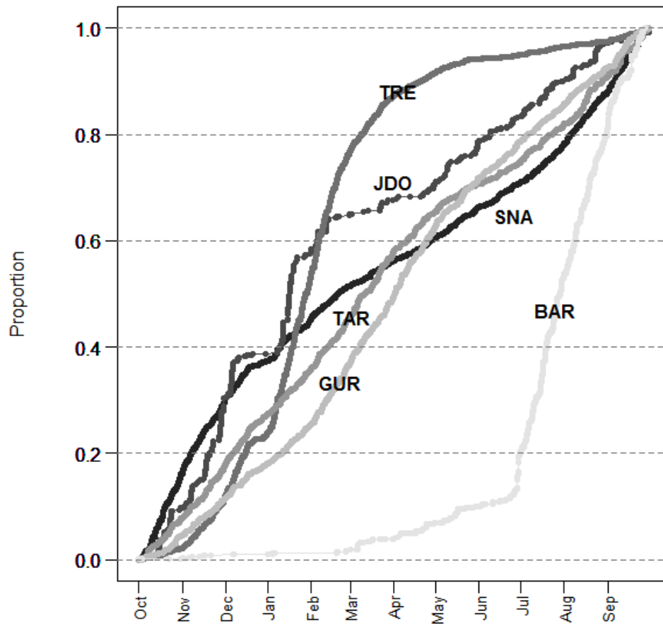
Figure 37: Cumulative catches of John dory in West Coast North Island, by target species, by day of fishing year and for 1994-95 to 2010-11, after applying the target species and vessel selection criteria. Catches are summed in chronological order through the fishing year.
