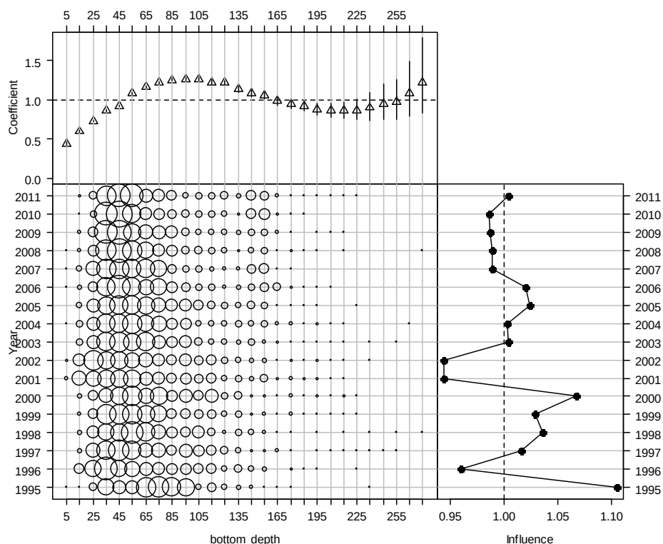
Figure A2.15: Effect and influence of bottom depth in the West coast North Island CPUE normal model. Top: relative effect by level of variable; Bottom-left, relative distribution of variables by fishing year; Bottom-right, influence of variable on unstandardized CPUE by fishing year.
