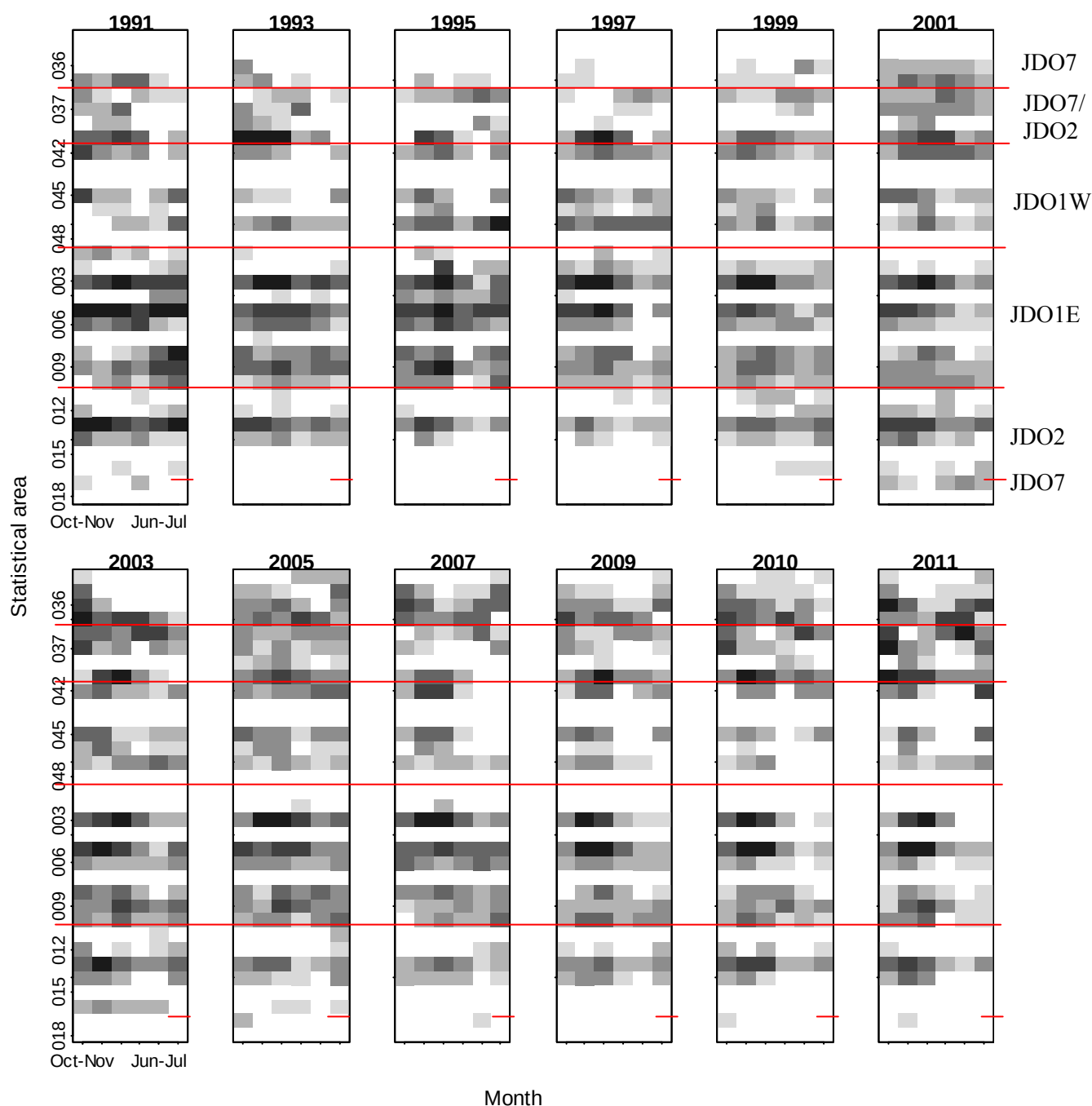
Figure 17: Image plot of the raw catch of John dory per unit effort (CPUE) by bottom trawlers within statistical areas, for selected fishing years, and by bi-monthly groups. CPUE is catch per hour for tows where John dory catches were reported. From top to bottom, statistical areas are ordered numerically from south to north from the northern South Island up the west coast of the North Island, and then south down the east coast of the North Island. On the west coast, the areas are ordered 040, 037, 039, 038, 036, 035, 034. The top right panel is labelled with the splits between the quota management areas (note that statistical area 017, nominally within the JDO2 section, is actually in JDO7).
