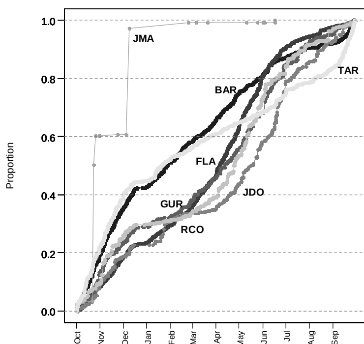
Figure 45: Cumulative catches of John dory in Northern South Island, by target species, by day of fishing year and for 2007–08 to 2010–11, after applying the target species and vessel selection criteria. Catches are summed in chronological order through the fishing year.
