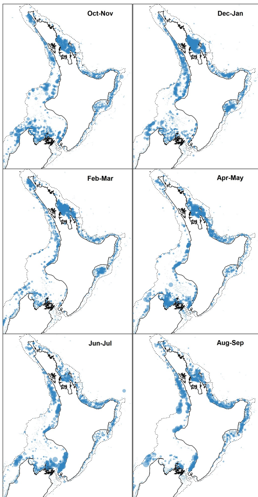
Figure 23: Catch of John dory per hour fished by bottom trawlers in 2009–10, by bi-monthly groups. Circle size is proportional to catch rate; the largest circle in each plot represents the largest catch rate in that two-month period. Dotted line, 200 m isobath.
