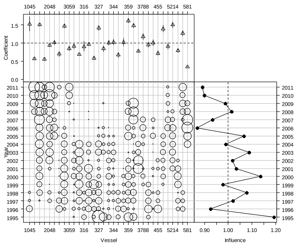
Figure A2.14: Effect and influence of vessel in the West coast North Island CPUE normal model. Top: relative effect by level of variable; Bottom-left, relative distribution of variables by fishing year; Bottom-right, influence of variable on unstandardized CPUE by fishing year.
