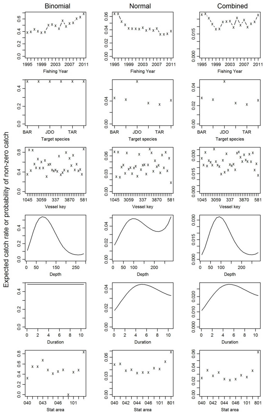
Figure 40: Model predictions for the West Coast North Island index, by fishing year (labelled as year ending, i.e., 1991 means 1990–91) and other selected predictors, for the binomial, normal and combined model, made with all other predictors set to the median (fixed) values.
