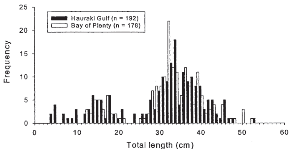
Figure 8: Length frequency distribution of John dory from research surveys of the Hauraki Gulf and Bay of Plenty in May 1987. Reproduced from Hanchet et al. (2001).
