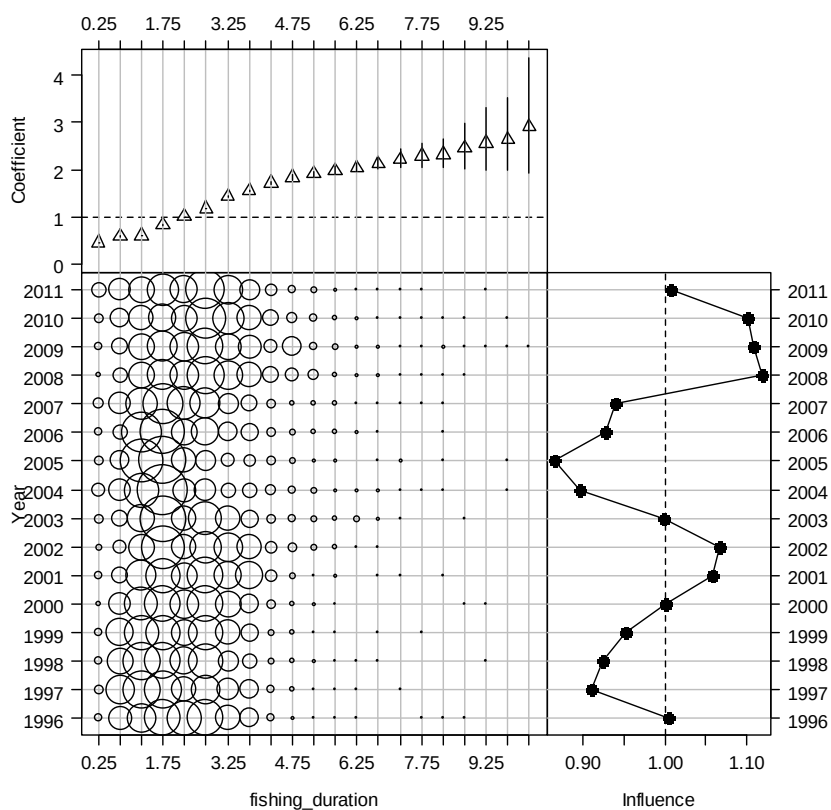
Figure A2.4: Effect and influence of fishing duration in the Hauraki Gulf and east Northland CPUE normal model. Top: relative effect by level of variable; Bottom left, relative distribution of variables by fishing year; Bottom right, influence of variable on unstandardized CPUE by fishing year.
