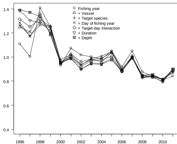
Figure A2.6: Annual CPUE indices for the Bay of Plenty stock normal model at each step in the variable selection process.
