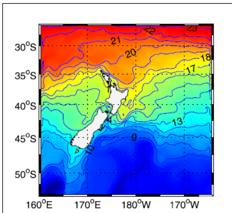
Figure 49: Average sea surface temperature from the New Zealand Regional Simulation Model (Chiswell & Rickard 2006).
