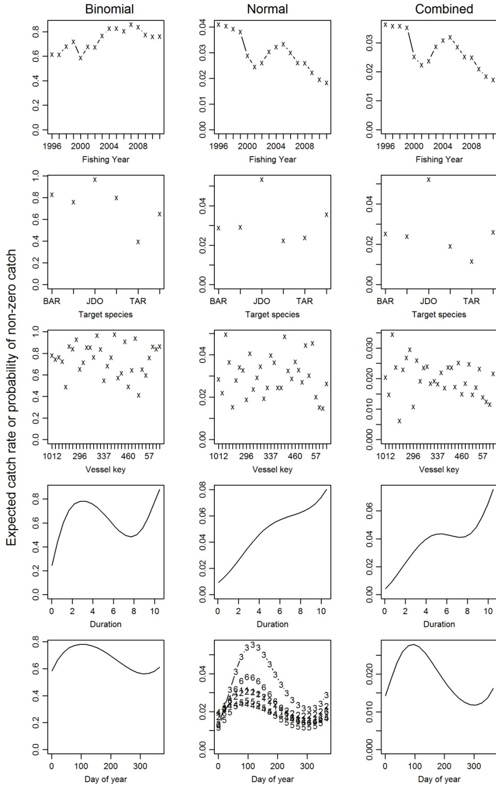
Figure 32: Model predictions for the Hauraki Gulf and east Northland index, by fishing year (labelled as year ending, i.e., 1991 means 1990–91) target species, vessel key, tow duration, day of year, and statistical area, for the binomial, normal and combined model, made with all other predictors set to the median (fixed) values. The day of year \times target species interaction is shown in the centre bottom panel: 1 BAR; 2 GUR; 3 JDO; 4 SNA; 5 TAR; 6 TRE.
