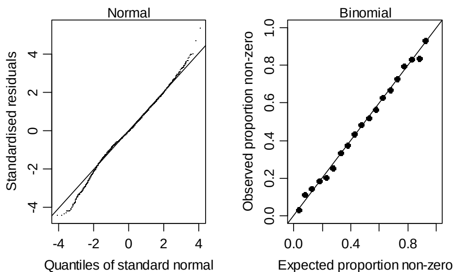
Figure 39: Q-Q plots for the fit of the West Coast North Island index.
