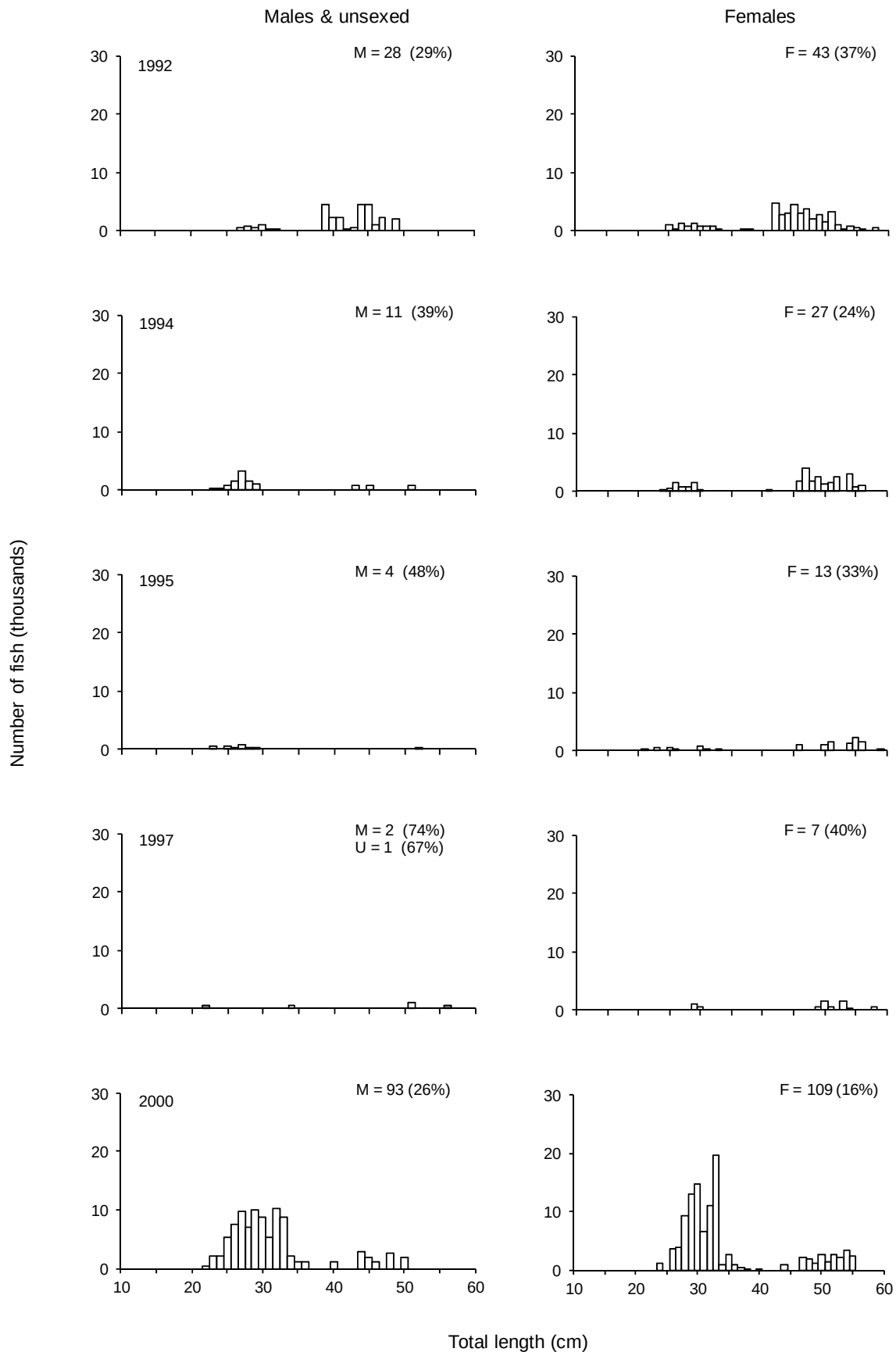
Figure 9: Scaled length frequency distributions for John dory sampled in the west coast South Island trawl survey (February–March), by year and sex (Stevenson, pers.comm.).
