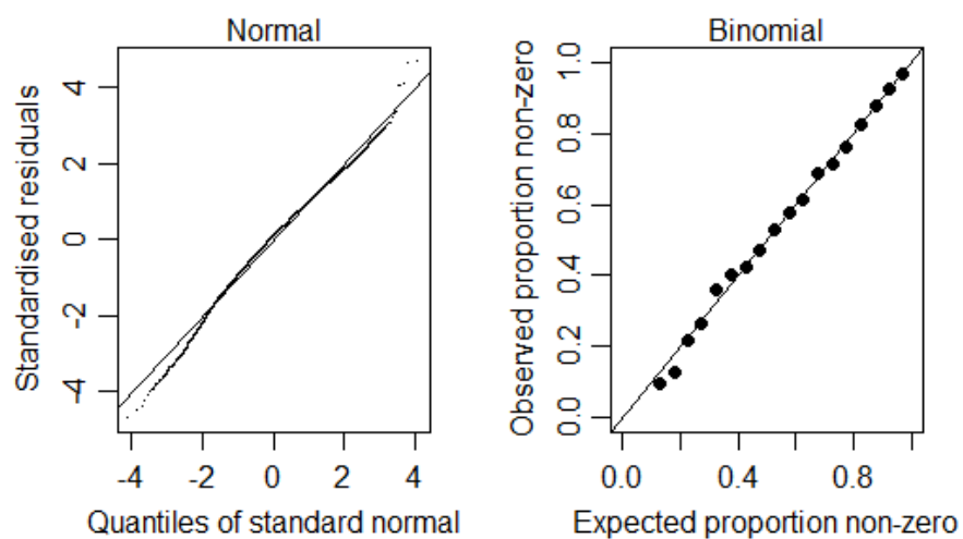
Figure 43: Q–Q plots for the fit of the Southeast North Island index.
