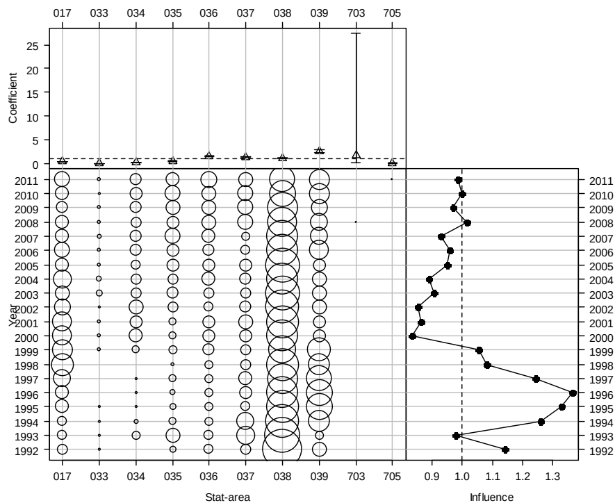
Figure A2.24: Effect and influence of statistical area in the northern South Island CPUE normal model. Top: relative effect by level of variable; Bottom-left, relative distribution of variables by fishing year; Bottom-right, influence of variable on unstandardized CPUE by fishing year.
