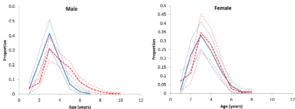
Figure 5: Estimated proportion at age (dark shaded lines) with 95% credible intervals (light shaded lines) for male and female John dory from the east coast of JDO1 (solid lines) and west coast JDO1 (broken lines). Estimates from Phillips & Horn (2004).
