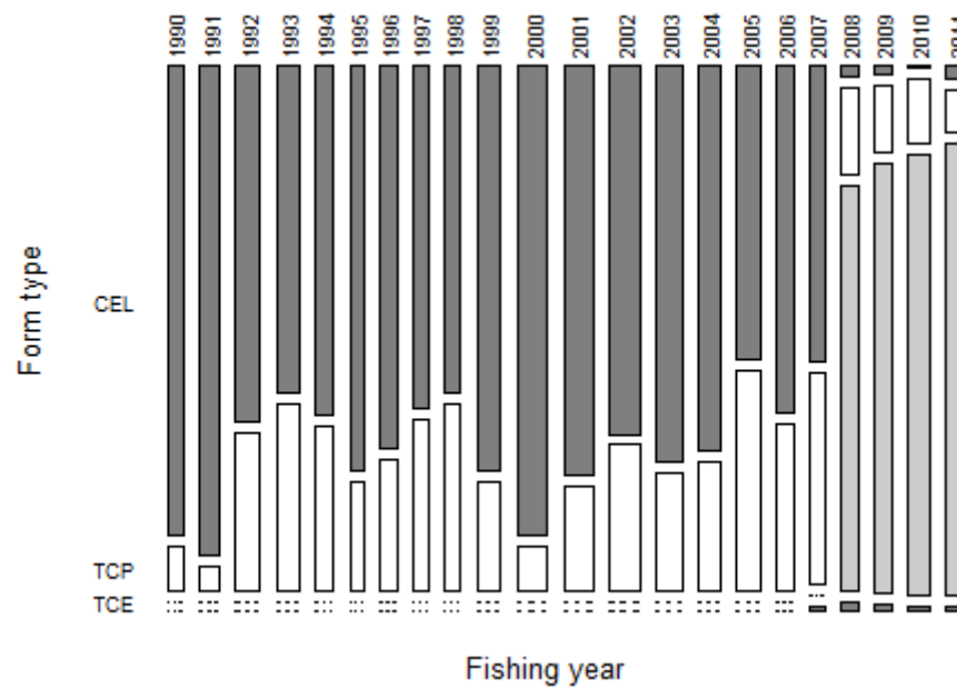
Figure A1.7: The proportion of estimated catches of John dory by form type for JDO 2. CEL, Catch Effort Landing Return; TCP, – Trawl Catch Effort Processing Return (for vessels >28 m in length); TCE, Trawl Catch Effort Return (for vessels 6–28 m in length).
