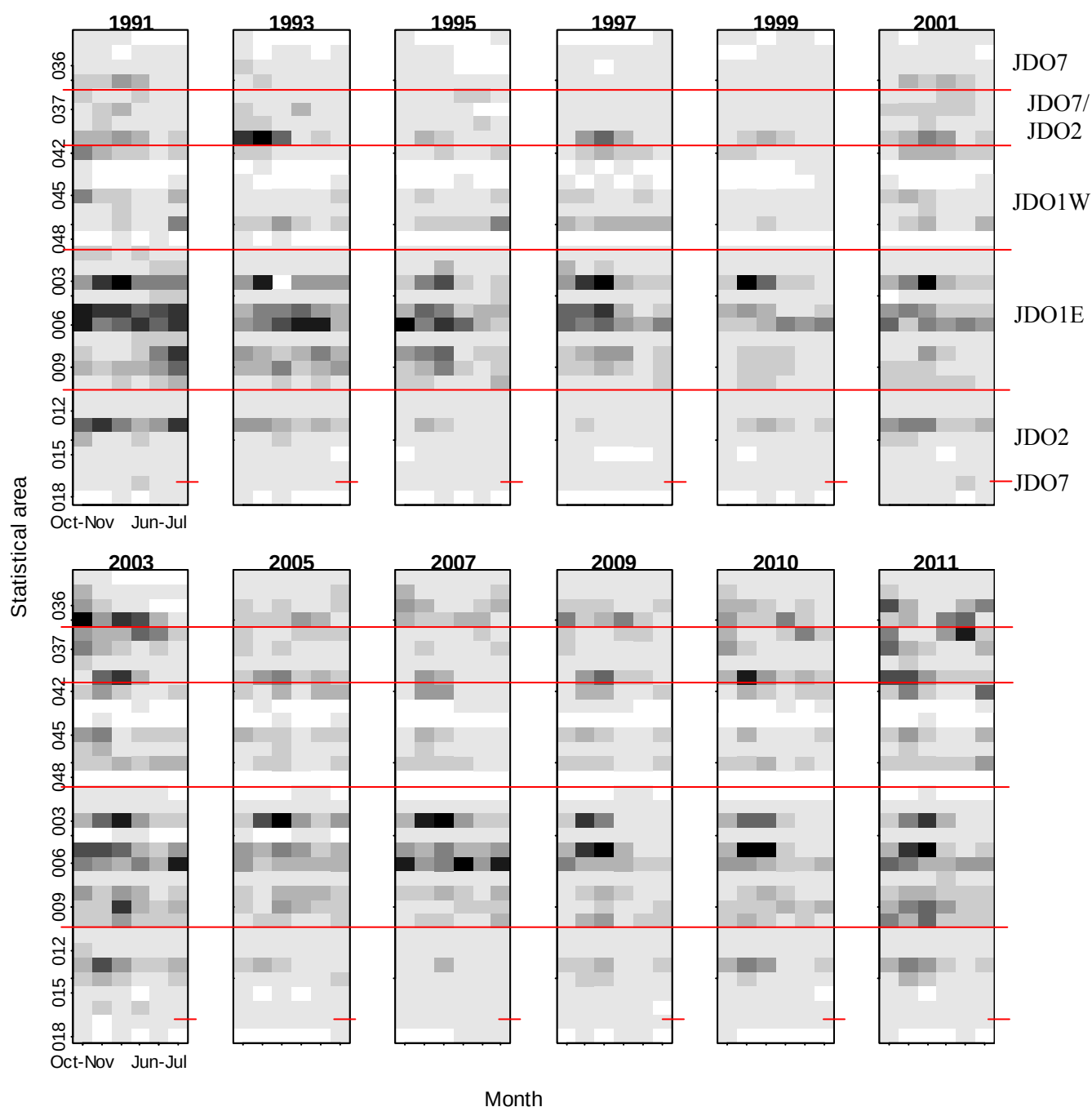
Figure 15: Image plot of the total catch of John dory for selected fishing years, by statistical area and bi-monthly groups. Darker cells indicate greater catches. From top to bottom, statistical areas are ordered numerically from south to north from the northern South Island up the west coast of the North Island, and then south down the east coast of the North Island. On the west coast, the areas are ordered 040, 037, 039, 038, 036, 035, 034. The top right panel is labelled with the splits between the quota management areas (note that statistical area 017, nominally within the JDO2 section, is actually in JDO7).
