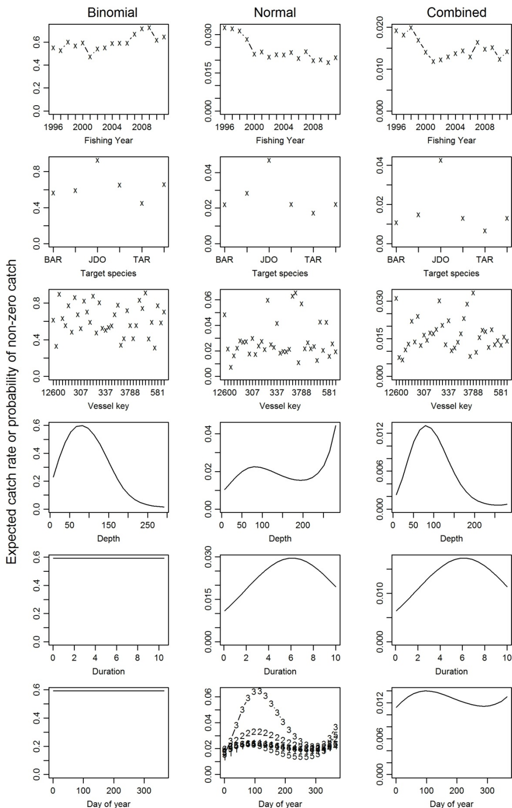
Figure 36: Model predictions for the Bay of Plenty index, by fishing year (labelled as year ending, i.e., 1991 means 1990–91) and other selected predictors, for the binomial, normal and combined model, made with all other predictors set to the median (fixed) values. The day of year \times target species interaction is shown in the centre bottom panel: 1 BAR; 2 GUR; 3 JDO; 4 SNA.
