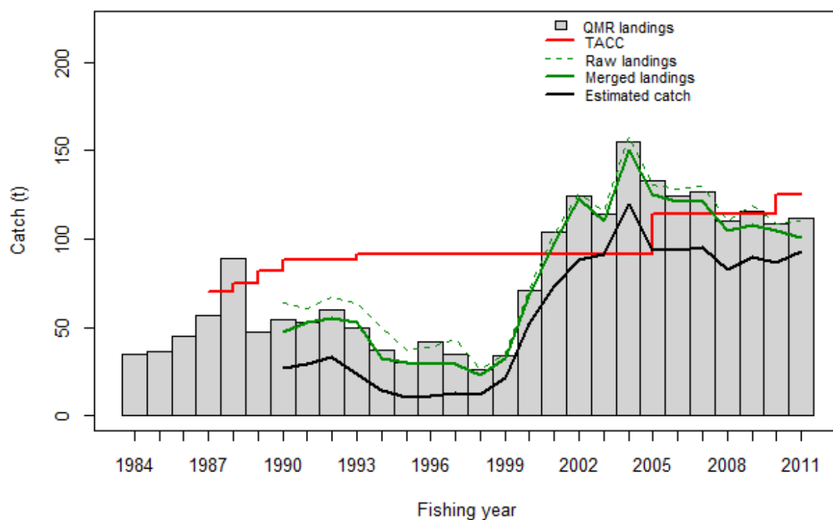
Figure A1.13: John dory official (Quota Management Reports: QMR) landings and TACC, and the raw, merged, and estimated catches in the catch-effort dataset, for JDO7.
