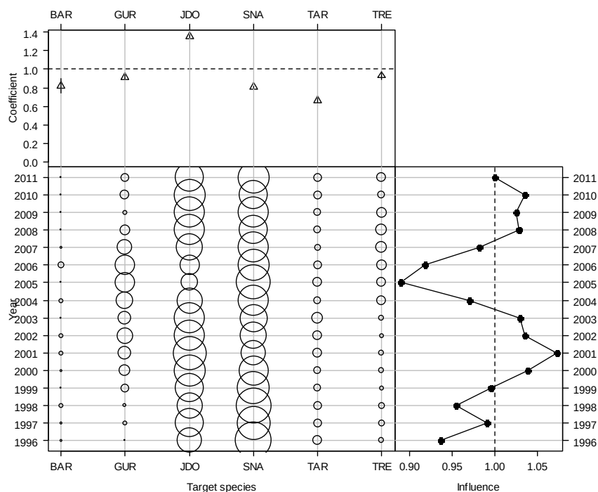
Figure A2.2: Effect and influence of target species in the Hauraki Gulf and east Northland CPUE normal model. Top: relative effect by level of variable; Bottom left, relative distribution of variables by fishing year; Bottom right, influence of variable on unstandardized CPUE by fishing year.
