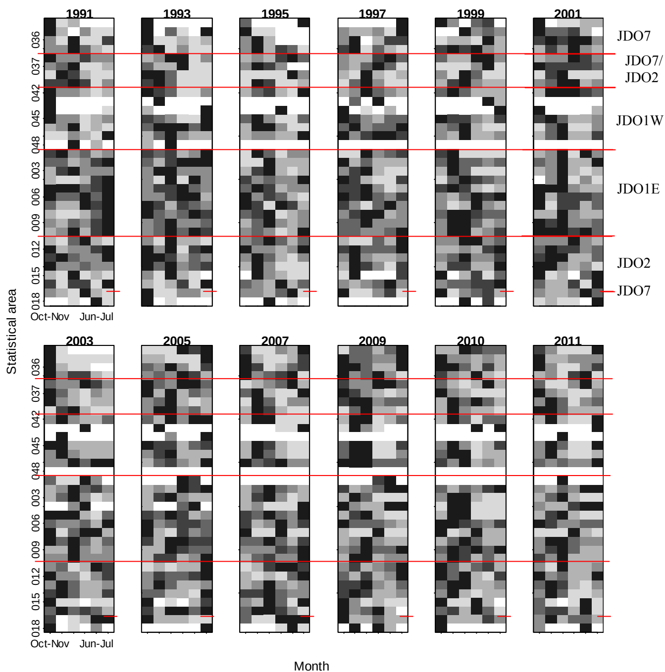
Figure 16: Image plot of the normalised catch of John dory within statistical areas, for selected fishing years, and by bi-monthly groups. Darker cells indicate greater relative catch within each statistical area. From top to bottom, statistical areas are ordered numerically from south to north from the northern South Island up the west coast of the North Island, and then south down the east coast of the North Island. On the west coast, the areas are ordered 040, 037, 039, 038, 036, 035, 034. The top right panel is labelled with the splits between the quota management areas (note that statistical area 017, nominally within the JDO2 section, is actually in JDO7).
