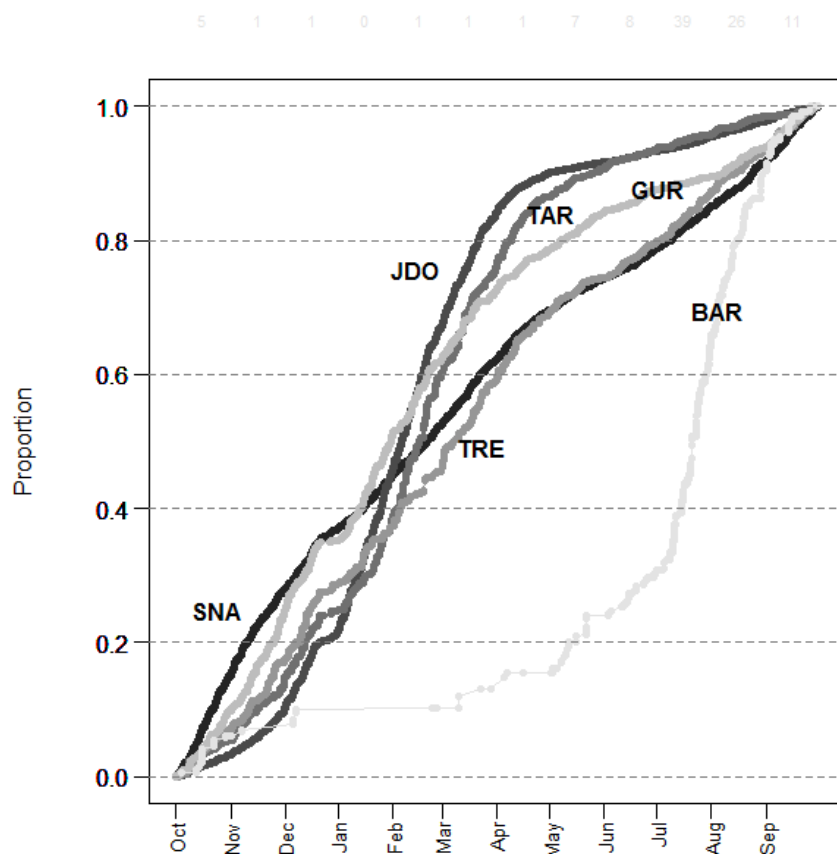
Figure 29: Cumulative catches of John dory in Hauraki Gulf and east Northland, by target species, by day of fishing year from 1995–96 to 2010–11, after applying the target species and vessel selection criteria. Catches are summed in chronological order through the fishing year.
