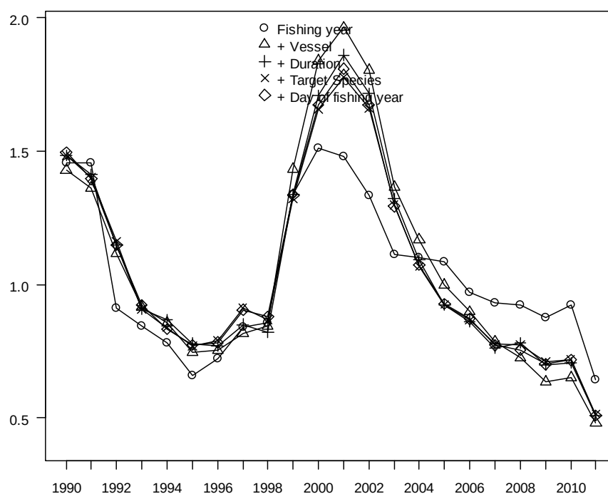
Figure A2.18: Annual CPUE indices for the Southeast North Island stock normal model at each step in the variable selection process.
