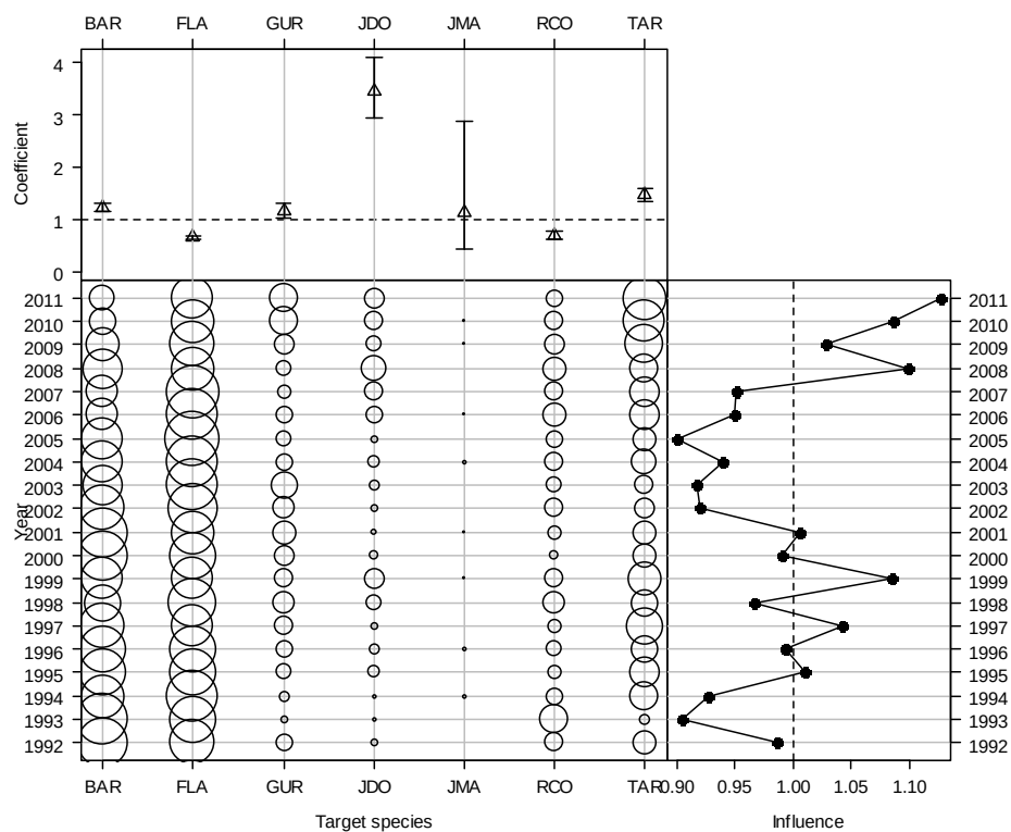
Figure A2.27: Effect and influence of target species in the northern South Island CPUE normal model. Top: relative effect by level of variable; Bottom-left, relative distribution of variables by fishing year; Bottom-right, influence of variable on unstandardized CPUE by fishing year.
