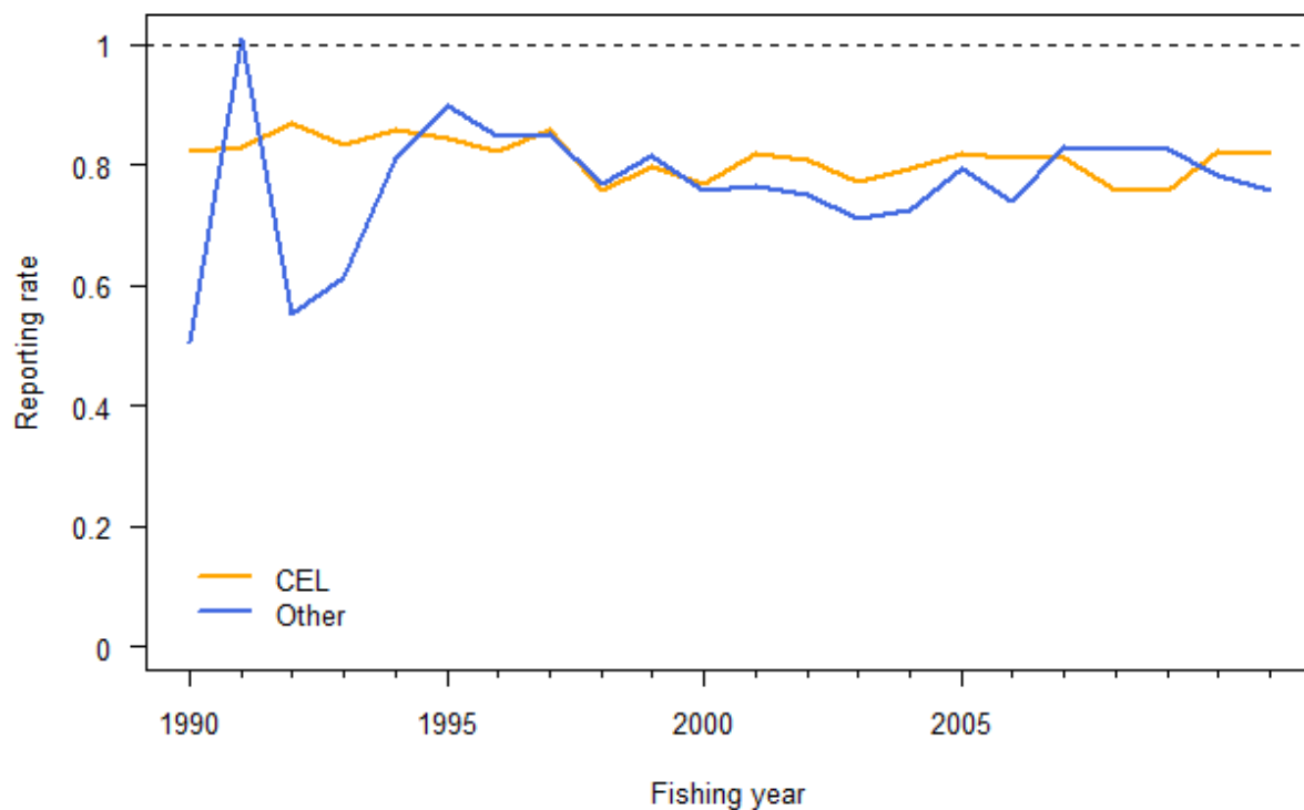
Figure A1.4: The reporting rate of John dory by form type for JDO 1. CEL, Catch Effort Landing Return. The reporting rate is the estimated catch divided by the trip-stratum (i.e., QMR) catch.
