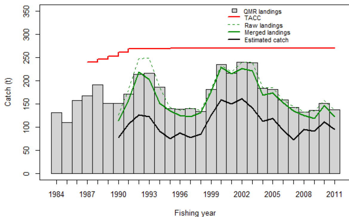
Figure A1.5: John dory official (Quota Management Reports: QMR) landings and TACC, and the raw, merged, and estimated catches in the catch-effort dataset, for JDO2.
