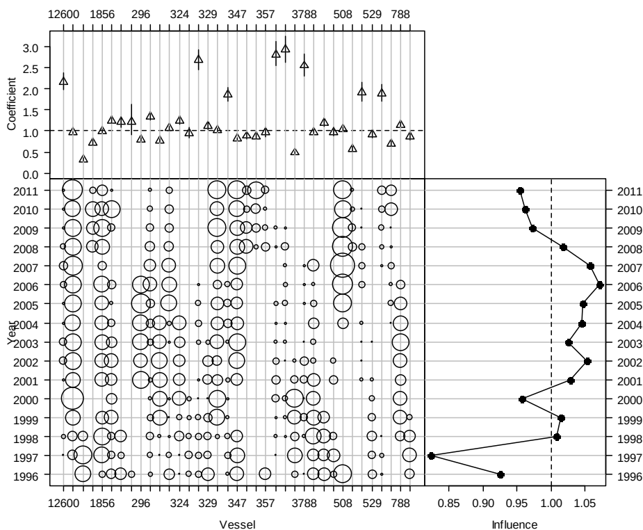
Figure A2.8: Effect and influence of vessel in the Bay of Plenty CPUE normal model. Top: relative effect by level of variable; Bottom-left, relative distribution of variables by fishing year; Bottom-right, influence of variable on unstandardized CPUE by fishing year.
