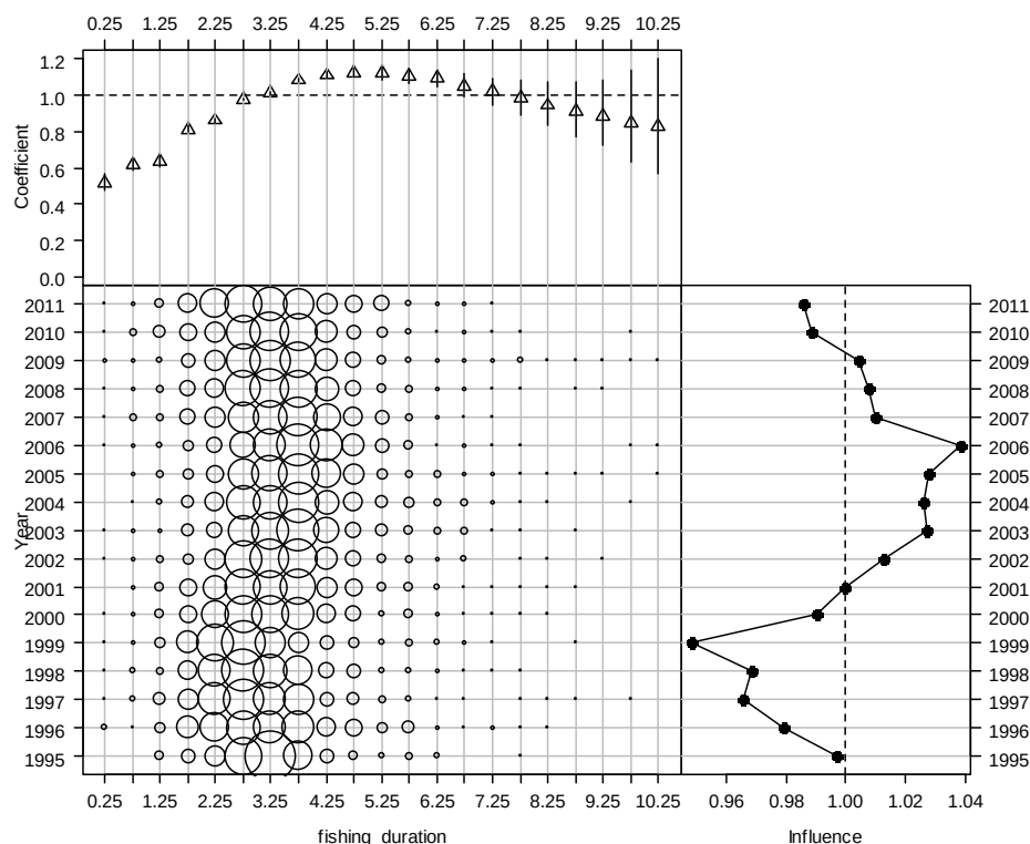
Figure A2.17: Effect and influence of fishing duration in the West coast North Island CPUE normal model. Top: relative effect by level of variable; Bottom-left, relative distribution of variables by fishing year; Bottom-right, influence of variable on unstandardized CPUE by fishing year.
