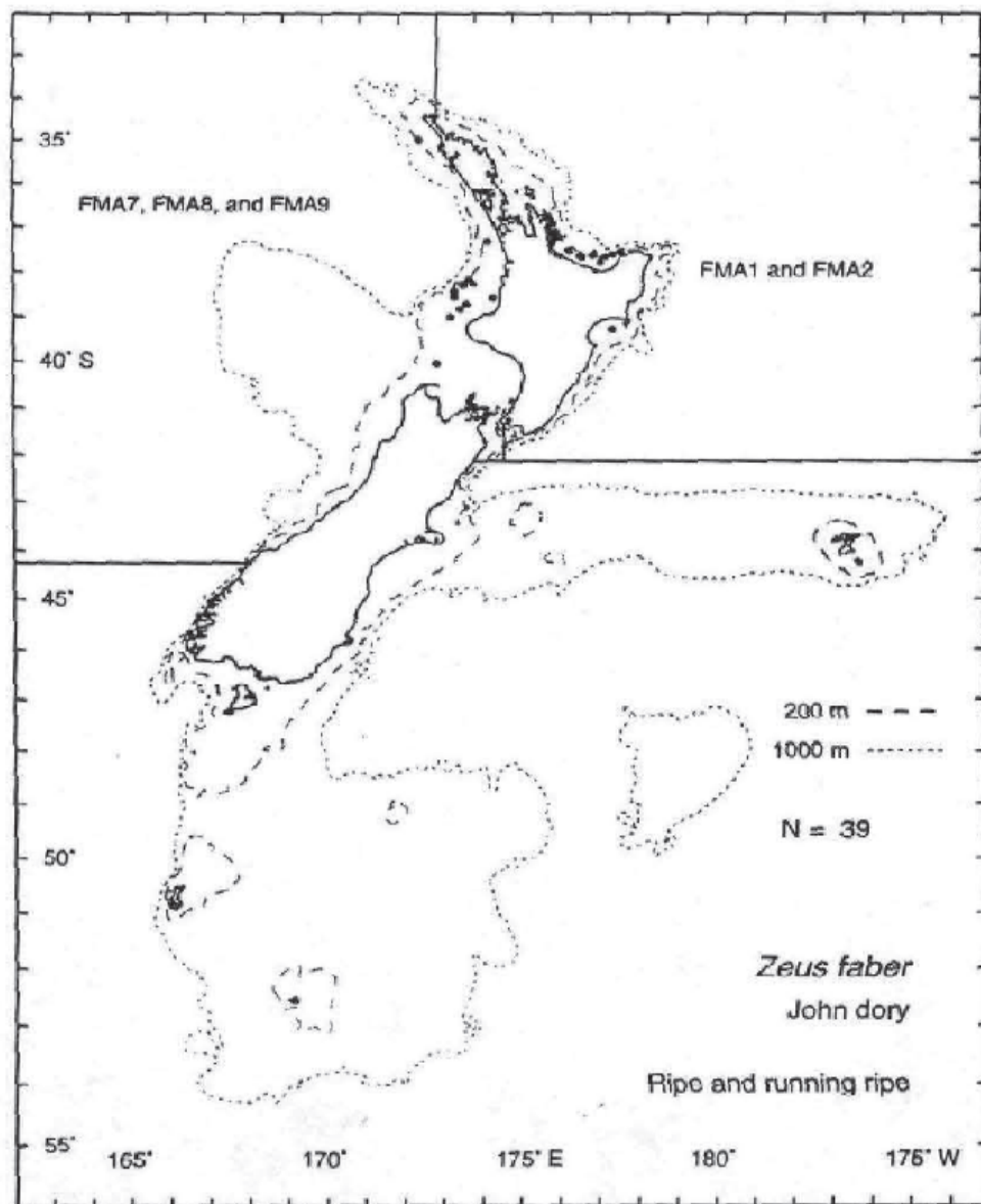
Figure 2: Observations of ripe and running ripe female John dory (black dots). Reproduced from Hurst et al. (2000).
