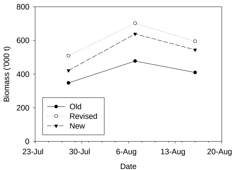
Figure 32: Estimated hoki abundance on the WCSI by snapshot over the 2012 survey period. Data were analysed using three methods (see text for details).
