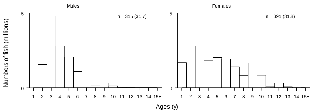
Figure 18: Scaled age frequency for hoki from core strata in the 2012 trawl survey. Number of fish aged ( n values) are given with CVs in parentheses. Hoki were not aged for the 2000 survey.
