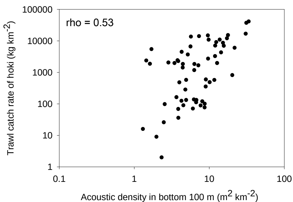
Figure 26: Relationship between trawl catch rate of hoki and bottom-referenced acoustic backscatter recorded during bottom tows during the 2012 WCSI survey. Rho value is Spearman's rank correlation coefficient.
