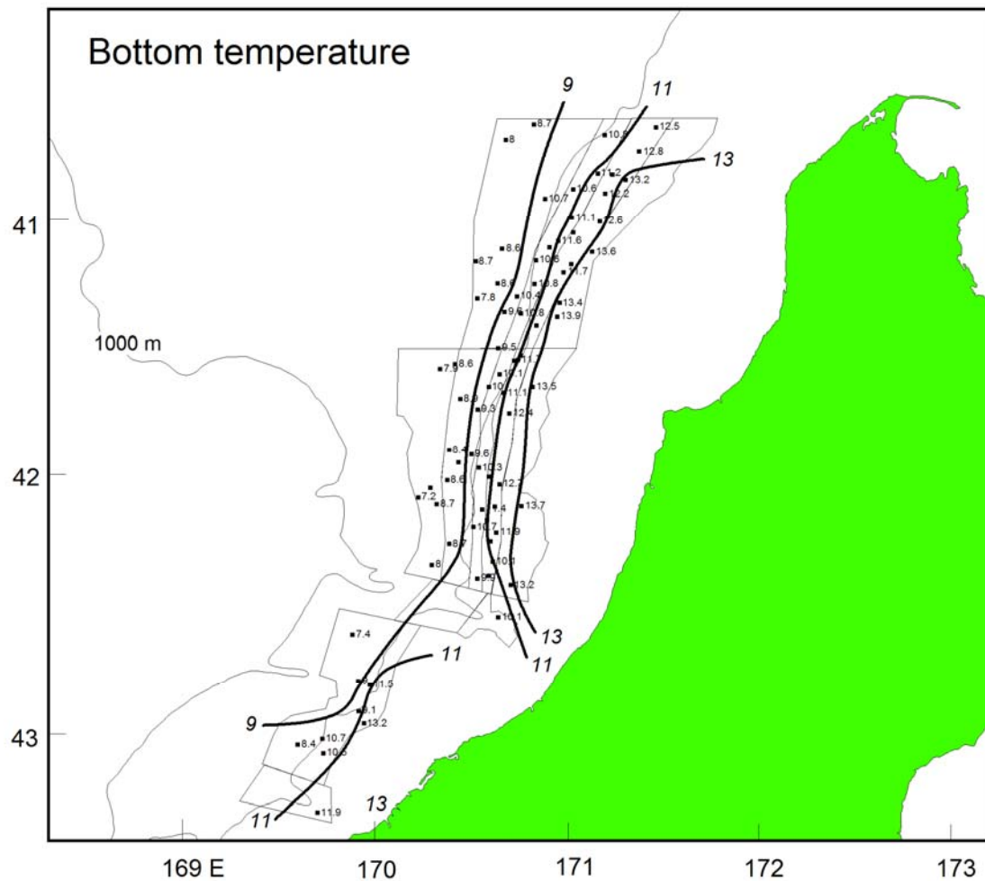
Figure 39: Bottom water temperatures (°C) during the 2012 WCSI survey. Squares indicate bottom trawl tow positions. Not all temperatures are labelled where two or more tows were close together. Contours show isotherms estimated by eye.
