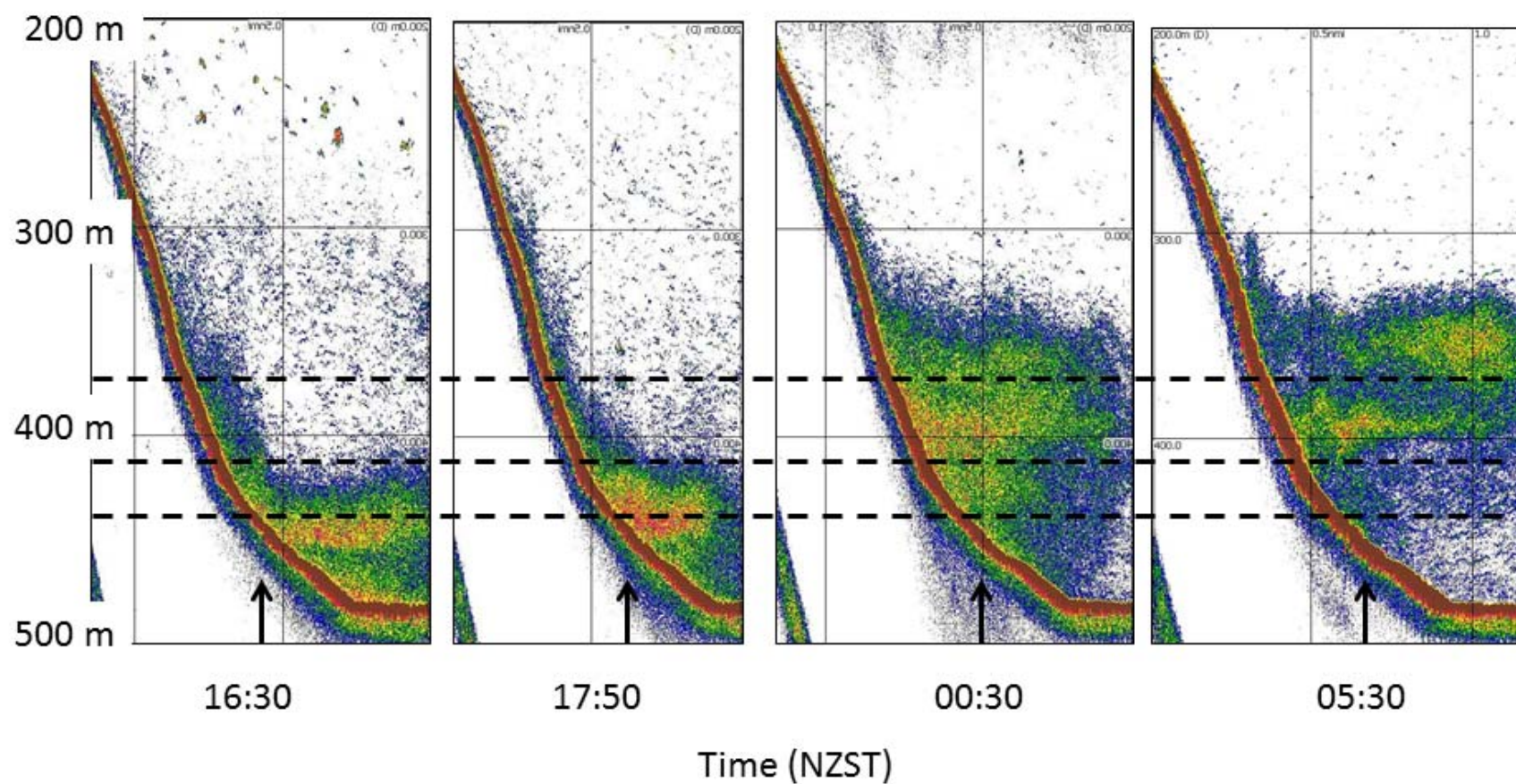
Figure 35: Echograms from four passes over the mooring on the south side of Hokitika Canyon on 26–27 July. Echograms have been oriented so that the south side is on the left. Arrows indicate approximate mooring location in each echogram. Dotted lines show approximate camera positions 8, 30, and 70 m above the seabed.
