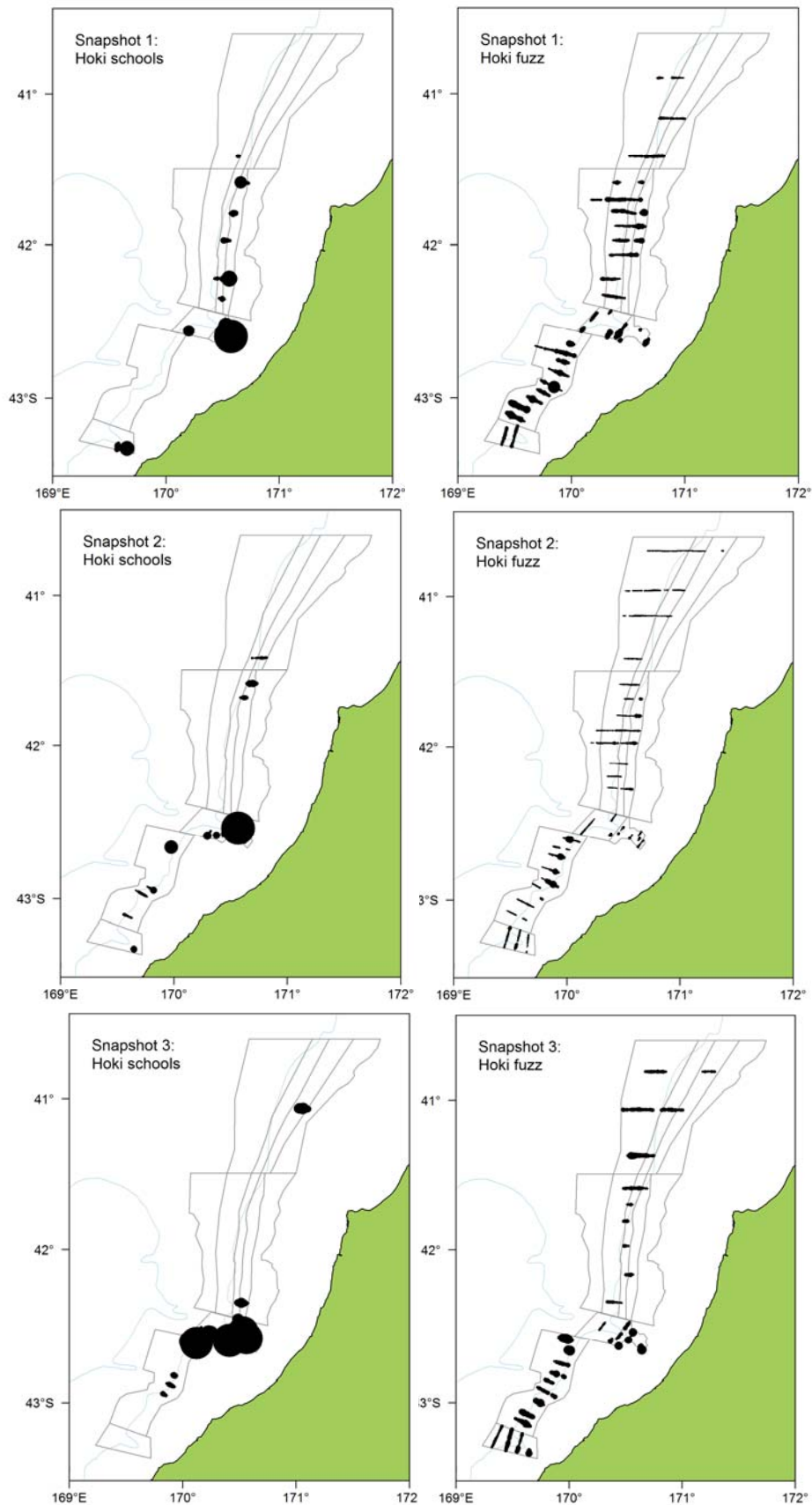
Figure 27: Spatial distribution of acoustic backscatter from hoki schools and hoki fuzz marks plotted in 10 ping (about 100 m) bins for the three snapshots of the WCSI. Symbol size is proportional to the log of the acoustic backscatter.
