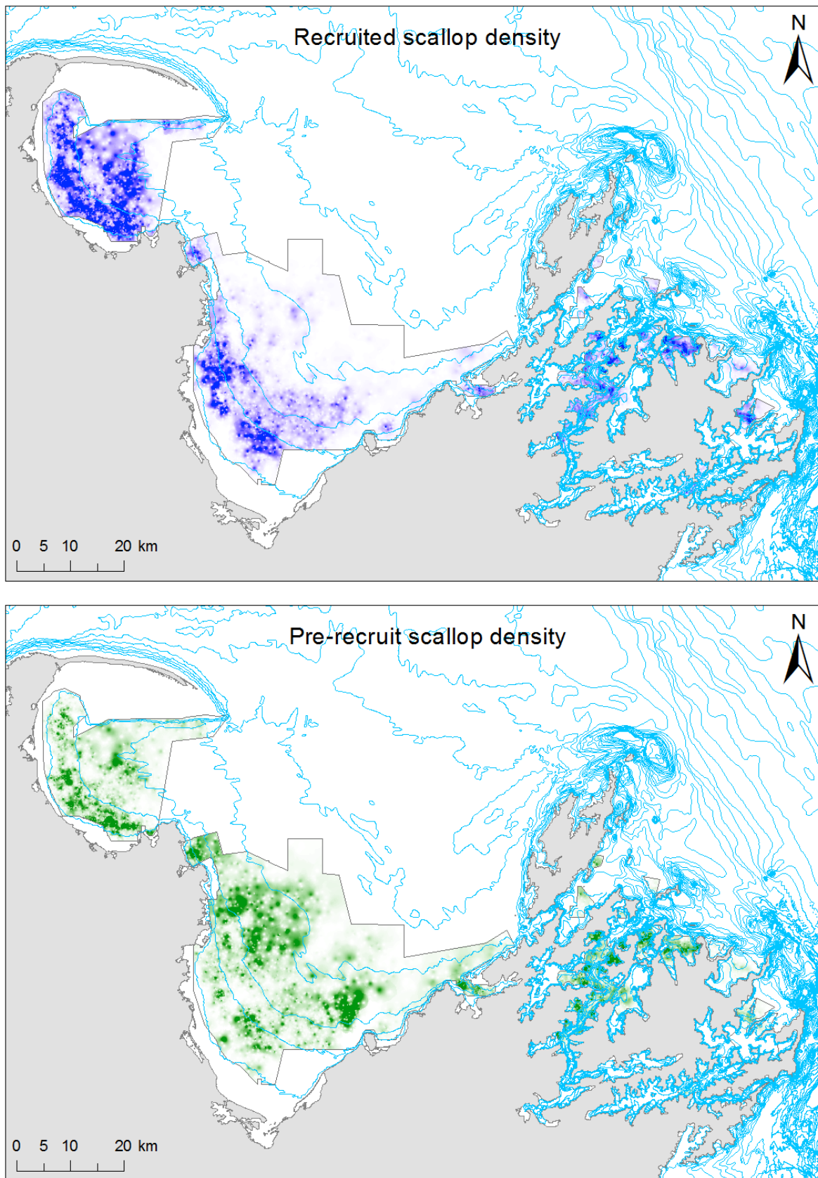
Figure 23: Spatial density of recruited (top) and pre-recruit (bottom) scallops in SCA 7 from an inverse density weighted (IDW) interpolation of SCA 7 survey estimates to 2011. Depth contours at 10 m intervals are shown overlaid for reference.
