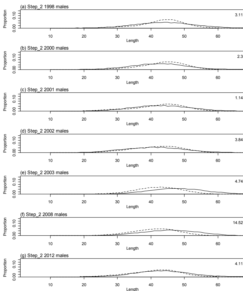
A5. 15: Observed (solid line) and fitted (dashed line) length frequency distributions for photographic survey scampi size estimation. Number in top right of each plot is effective sample size.
