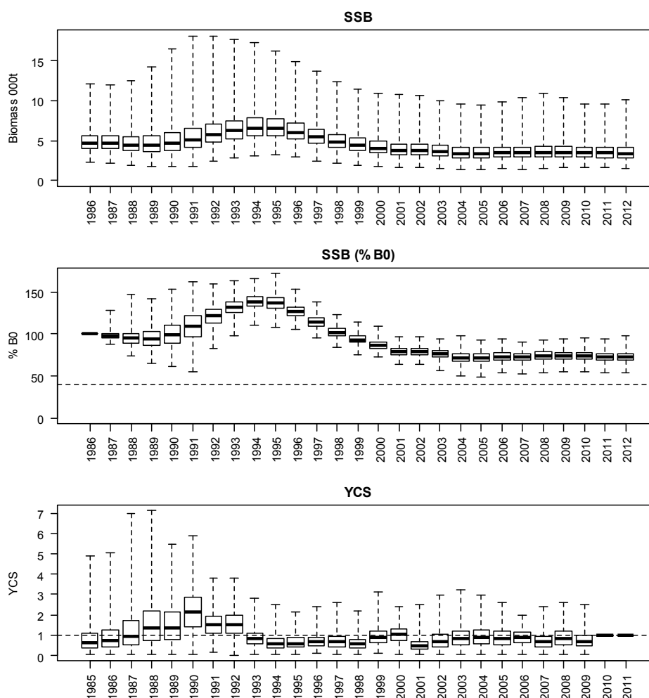
Figure 54: Posterior trajectory of SSB, SSB_{2012}/B_0 and YCS of MCMC run for SCI 1 Base3 model.
