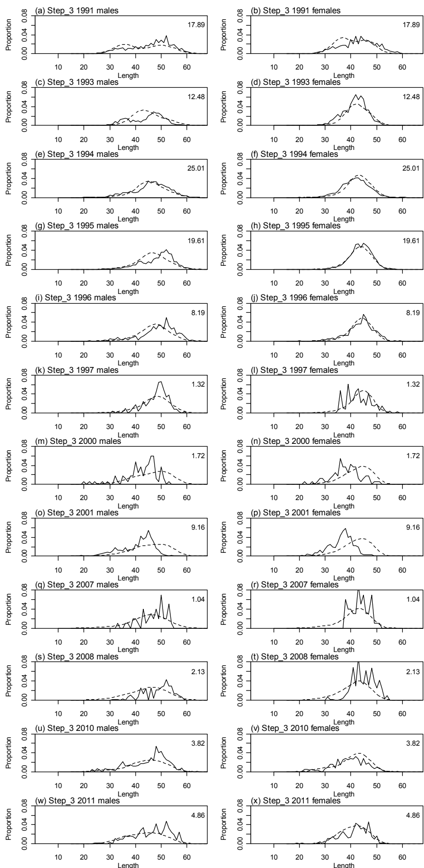
A6. 7: Observed (solid line) and fitted (dashed line) length frequency distributions for observer samples, time step 3. Number in top right of each plot is effective sample size.
