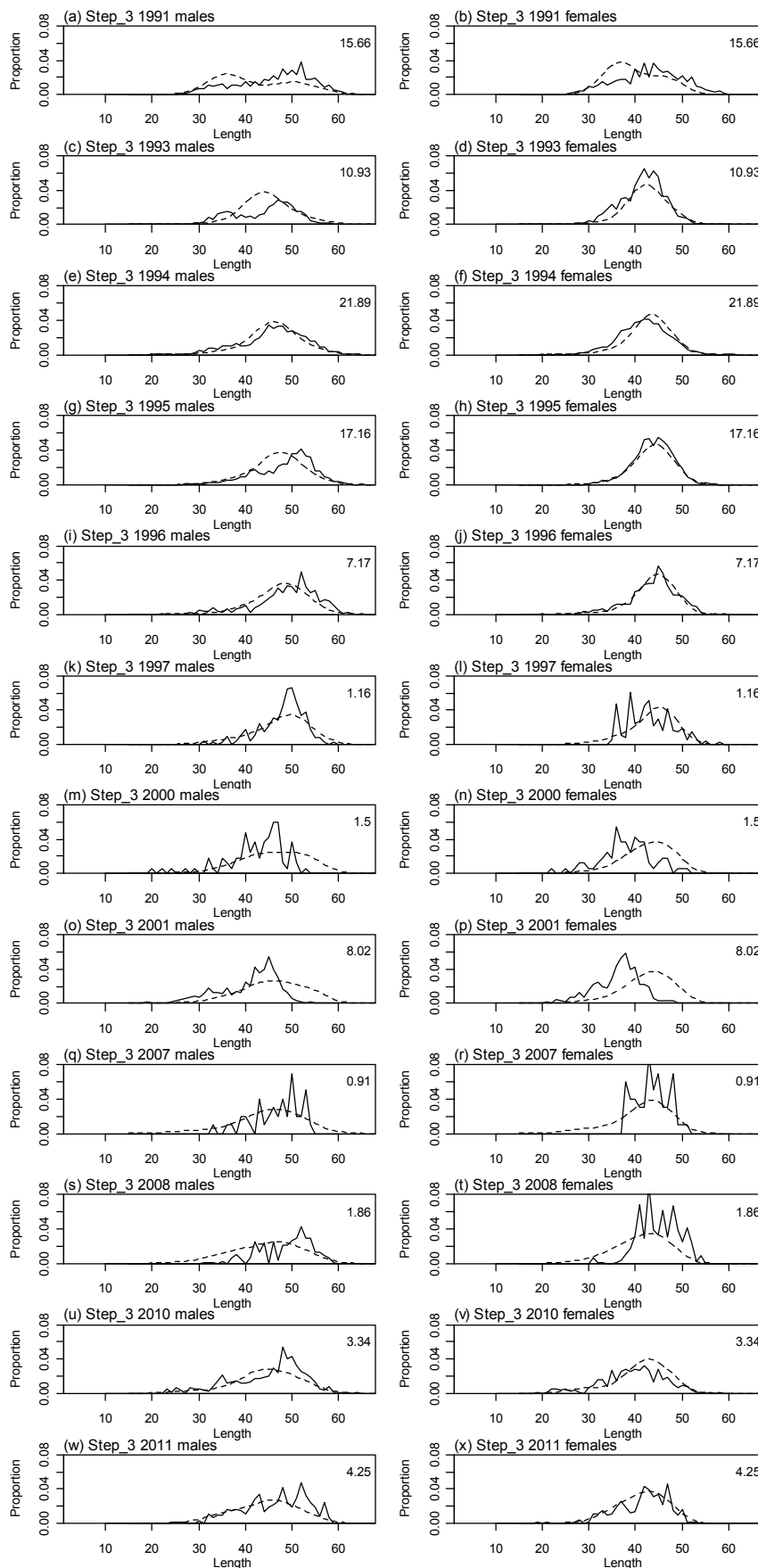
A7. 7: Observed (solid line) and fitted (dashed line) length frequency distributions for observer samples, time step 3. Number in top right of each plot is effective sample size.
