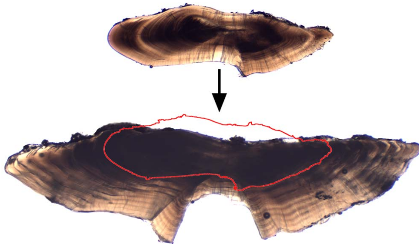
Figure 4: Thin section otolith from a 2 year old pre-recruit tarakihi (18 cm) with perimeter outline overlaid onto an adult tarakihi otolith to compare the position of the first annulus (reference set slide #48-5: 37cm, 8L, agreed age 8).
