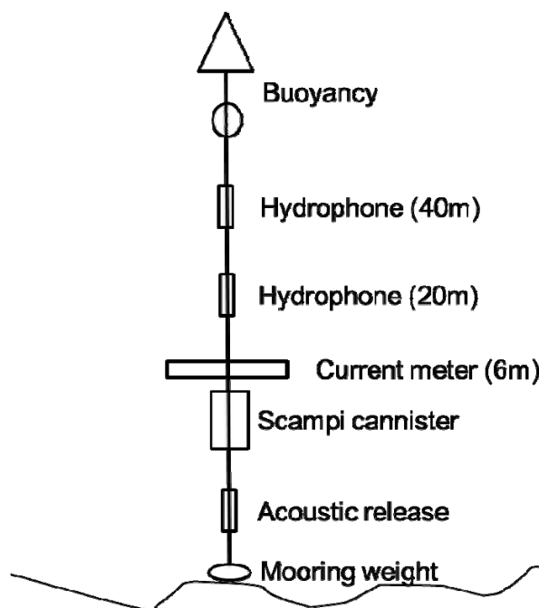
Figure 7: Diagram of acoustic mooring for deployment of scampi and hydrophones.
