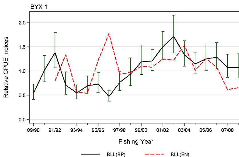
Comparison of the lognormal indices from the two bottom longline CPUE series for BYX 1: a) BLL[EN]: target bluenose/hapuku in East Northland; b) BLL[BP]: target bluenose/hapuku in Bay of Plenty. Each series is scaled so that the geometric mean = 1.
