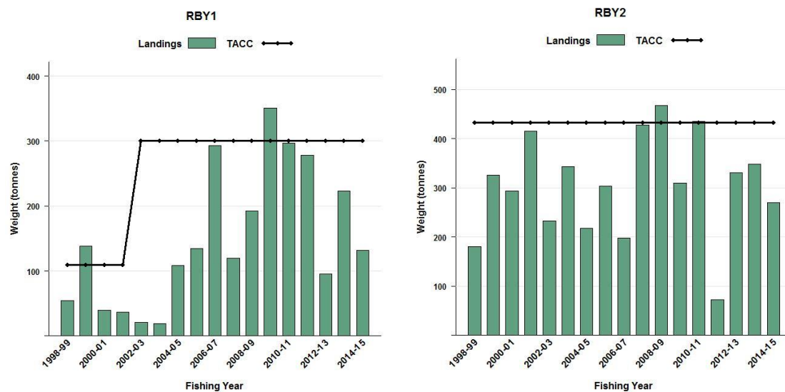
Figure 1: Reported commercial landings and TACC for the two main RBY stocks. Left to right: RBY 1 (Auckland East) and RBY 2 (Central East). Note that these figures do not show data prior to entry into the QMS.
