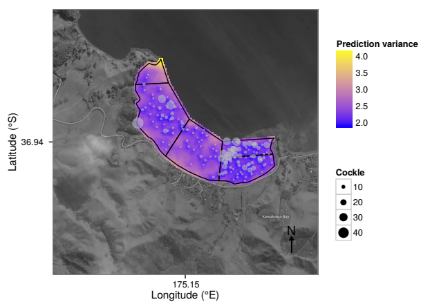
Figure B-1: Cockle abundance within existing stratification (black lines) at Okoromai Bay and Kawakawa Bay (West). Shown are sampling densities (size of the circles proportional to the number of cockles sampled per 0.035 m 2 ) with predicted densities (number of individuals per m 2 ) (left-hand column) and the prediction variance (right-hand column).
