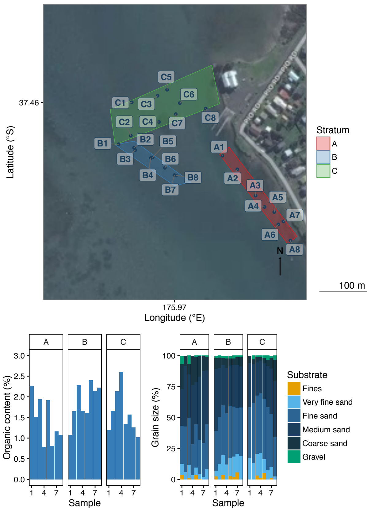
Figure 2: Sediment sample locations and characteristics at Bowentown Beach. Labels correspond to stratum and sample number. Graphs show organic content (% dry weight) and cumulative grain size (%). Sediment grain size fractions include fines (silt and clay; <63\ \mu\text{m} ), sands (very fine, >63\ \mu\text{m} ; fine, >125\ \mu\text{m} ; medium, >250\ \mu\text{m} ; coarse, >500\ \mu\text{m} ), and gravel ( >2000\ \mu\text{m} ) (see details in Table C-4).
