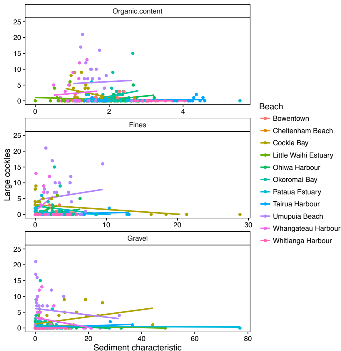
Figure 52: Sediment characteristics (organic content, proportion of fines, and proportion of gravel) and number of large (≥ 30 mm shell length) cockles in each sample. Regression lines relate to the two variables at each of the 2015–16 survey sites.
