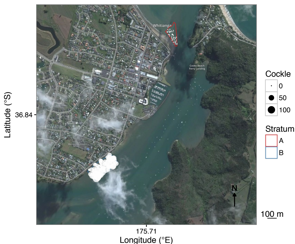
Figure 47: Map of sample strata and individual sample locations for cockles at Whitianga Harbour, with the size of the circles proportional to the number of cockles (per 0.035 m 2 ) found at each location. Samples with zero counts are shown as small dots.
