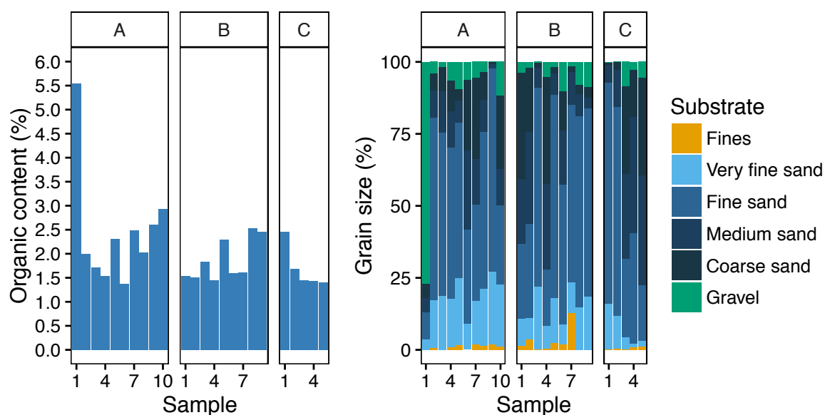
Figure 28: Sediment sample locations and characteristics at Pataua Estuary. Labels correspond to stratum and sample number. Graphs show organic content (% dry weight) and cumulative grain size (%). Sediment grain size fractions include fines (silt and clay; <63 µm), sands (very fine, >63 µm; fine, >125 µm; medium, >250 µm; coarse, >500 µm), and gravel (>2000 µm) (see details in Table C-4).
