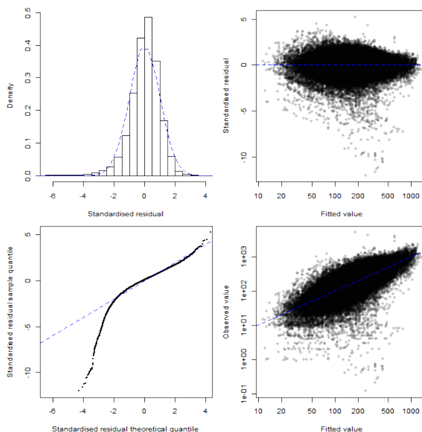
Figure 22: Residual diagnostics for the CPUE model for the Hauraki Gulf fishery. Top left: histogram of standardised residuals compared to standard normal distribution. Bottom left: quantile-quantile plot of standardised residuals. Top right: fitted values versus standardised residuals. Bottom right: observed values versus fitted values.
