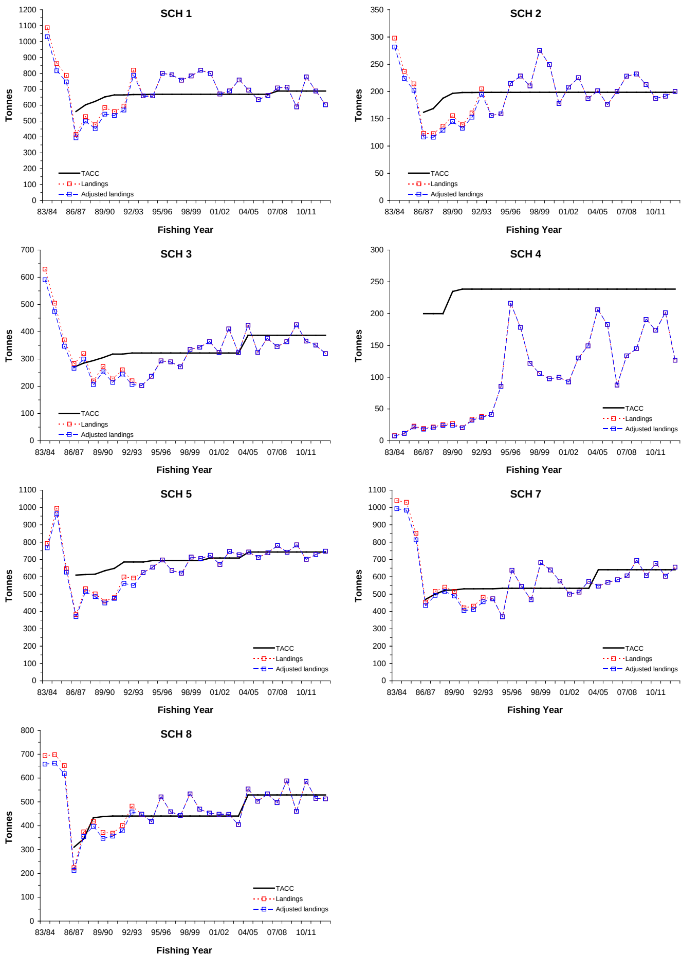
Figure 2: Plots of SCH 1, SCH 2, SCH 3, SCH 4, SCH 5, SCH 7 and SCH 8 landings and TACCs from 1983–84 to 2012–13 (see Table C.1 for list of landings and TACCs by SCH QMA).
