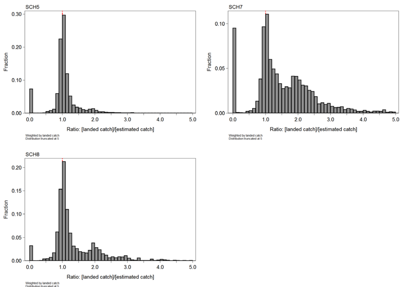
Figure F.3B: Distribution (weighted by the landed catch) of the ratio of landed to estimated catch per trip in each of the SCH 5, SCH 7 and SCH 8 analysis datasets. Trips where the estimated catch=0 have been assigned a ratio=0.
