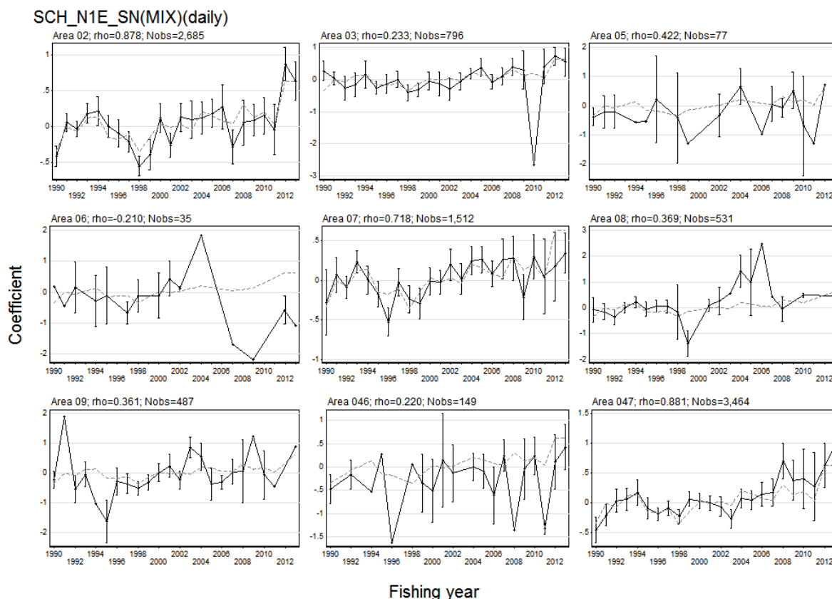
Figure I.11: Residual implied coefficients for area×fishing year interaction (not offered) in the school shark SN-N1E(MIX) lognormal model. Implied coefficients (black points) are calculated as the normalised fishing year coefficient (grey line) plus the mean of the standardised residuals in each fishing year and area. These values approximate the coefficients obtained when an area × year interaction term is fitted, particularly for those area × year combinations which have a substantial proportion of the records. The error bars indicate one standard error of the standardised residuals. The information at the top of each panel identifies the plotted category, provides the correlation coefficient ( \rho ) between the category year index and the overall model index, and the number of records supporting the category.
