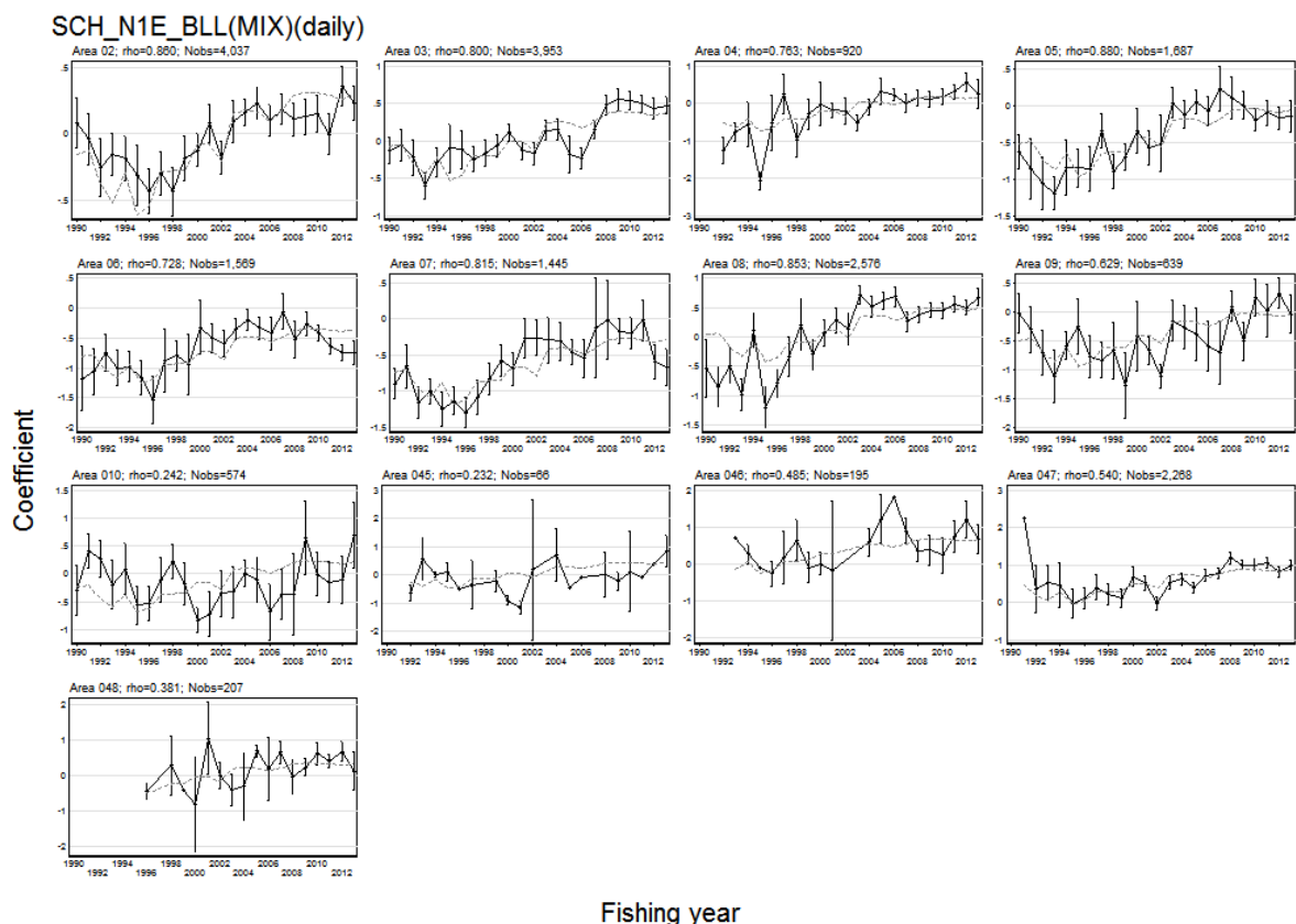
Figure J.11: Residual implied coefficients for area×fishing year interaction (not offered) in the school shark BLL-N1E(MIX) lognormal model. Implied coefficients (black points) are calculated as the normalised fishing year coefficient (grey line) plus the mean of the standardised residuals in each fishing year and area. These values approximate the coefficients obtained when an area × year interaction term is fitted, particularly for those area × year combinations which have a substantial proportion of the records. The error bars indicate one standard error of the standardised residuals. The information at the top of each panel identifies the plotted category, provides the correlation coefficient ( \rho ) between the category year index and the overall model index, and the number of records supporting the category.
