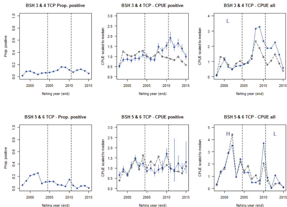
Figure 25: Proportion of positive trawl tows (left), standardised CPUE for all positive tows (middle) and standardised CPUE for all tows (right) estimated for seal shark reported on TCP forms in FMAs 3 & 4 (top) and FMAs 5 & 6 (bottom). Blue lines are the standardised series and whiskers are 95% confidence intervals; black lines are the nominal CPUE series. “L” and “H” indicate significantly low or high time periods.
