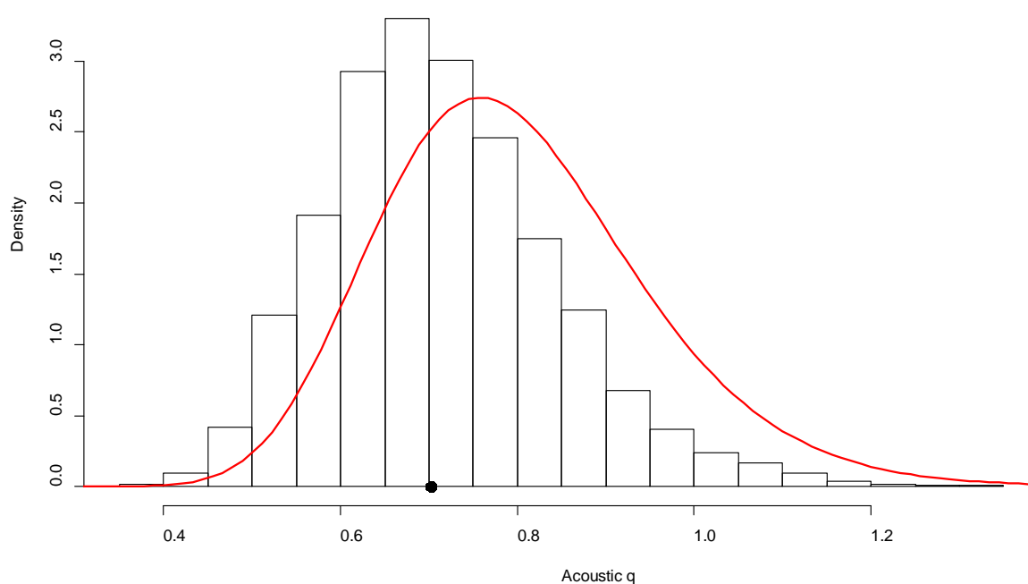
Figure 27: Puysegur: the marginal posterior distribution of the acoustic q (histogram) compared to its prior (red line). The black dot marks the median of the marginal posterior.
