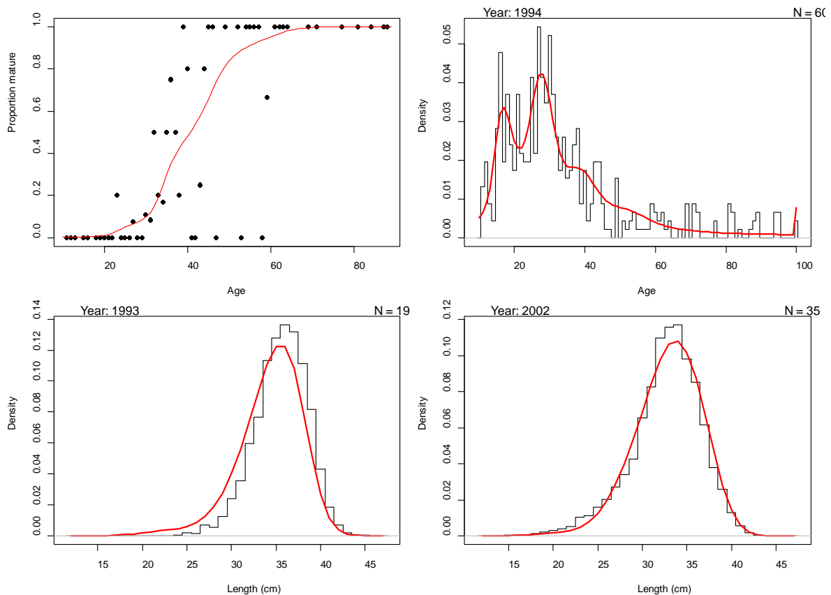
Figure 4: NWCR, base, MPD fits: (observations in black; predictions in red): (top) proportion mature at age; trawl survey age frequency ; (bottom) commercial length frequencies (N is the effective sample size).
