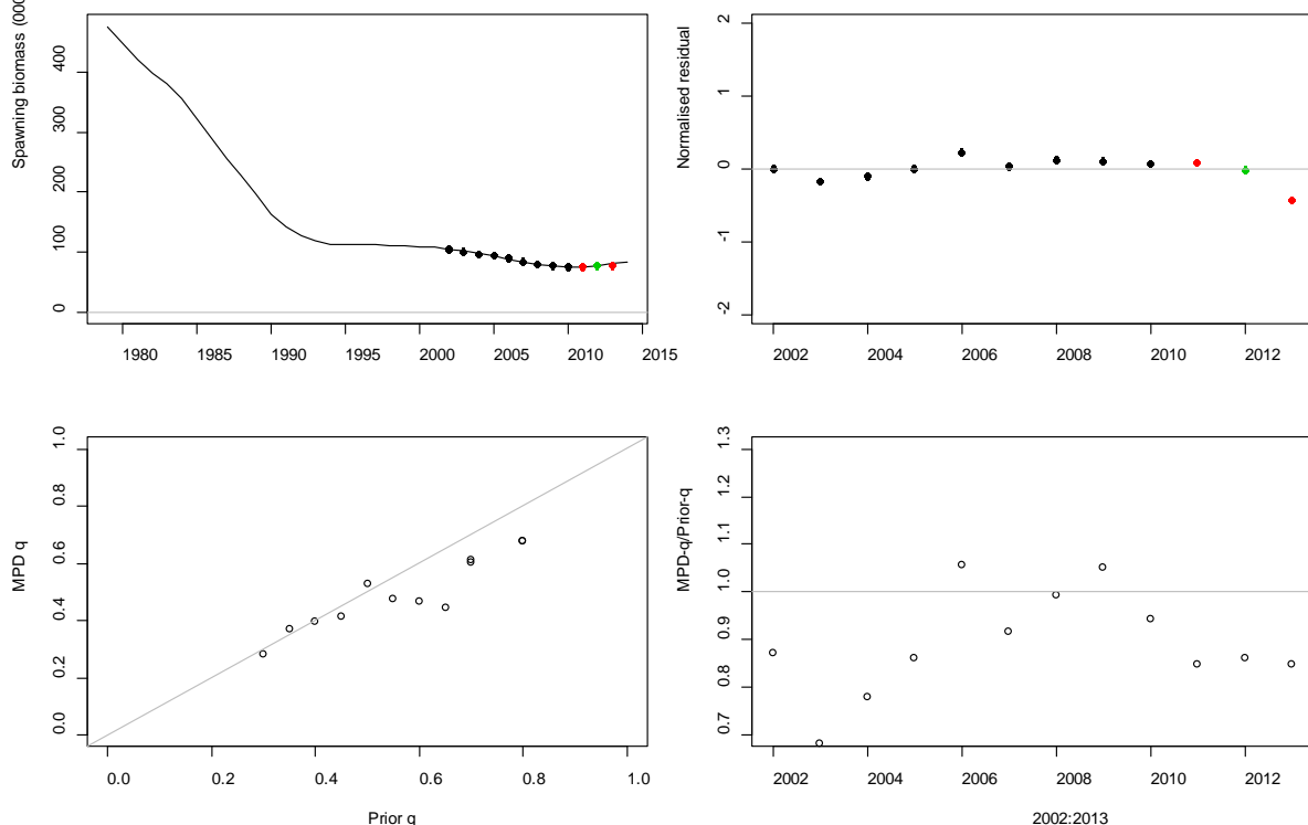
Figure 12: ESCR, MPD, base: fit to the acoustic indices: (top) spawning biomass trajectory and unscaled acoustic indices; normalised residuals; (bottom) estimated q_s as a function of the mean of the q prior; the ratio of the estimated q to the mean of the q prior.
