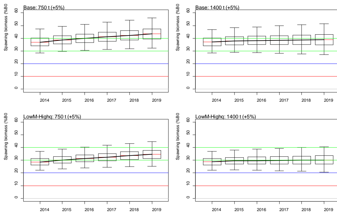
Figure 9: NWCRC base, MCMC projections. The box in each year covers 50% of the distribution and the whiskers extend to 95% of the distribution. The projections are for the model and annual catch indicated (a 5% over-run was included in each year). The target range is indicated by horizontal green lines.
