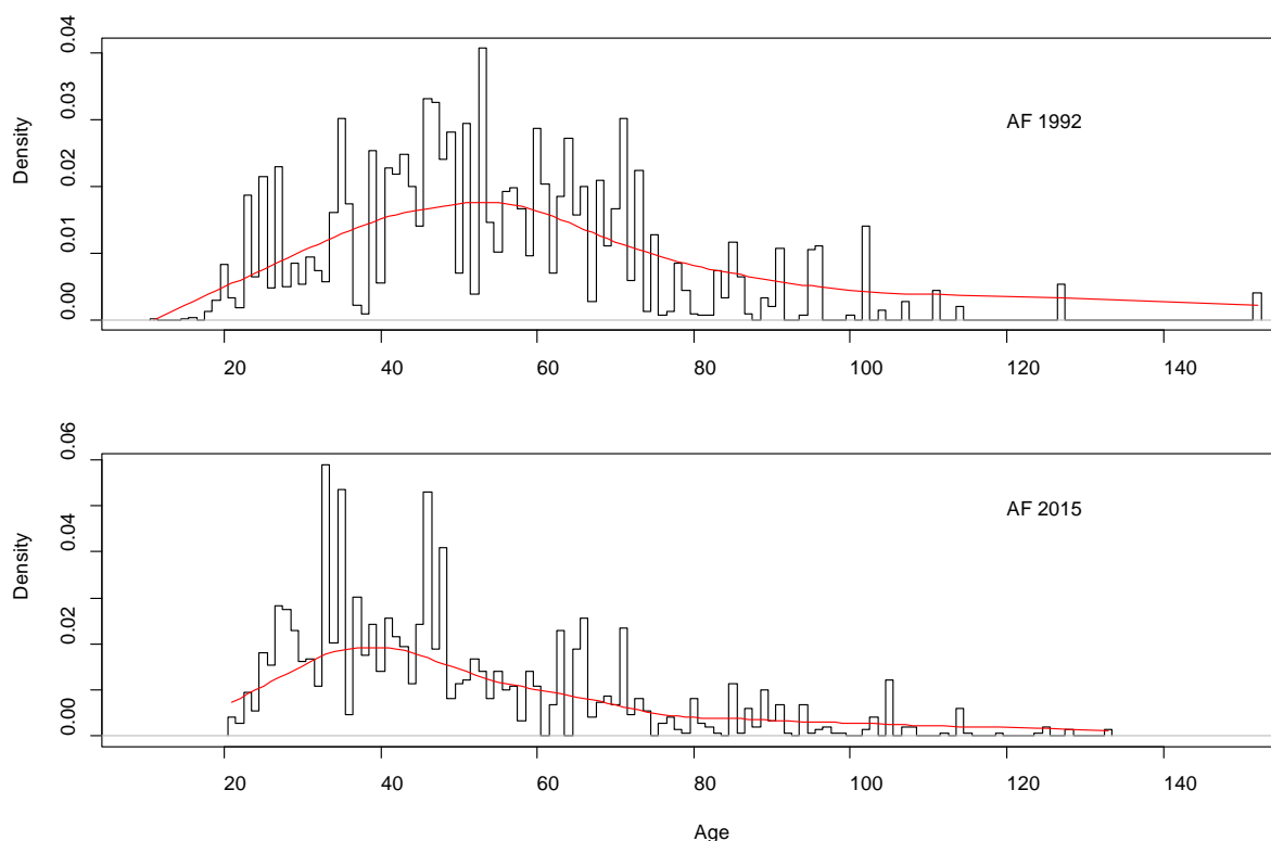
Figure 25: Puysegur: age frequencies from 1992 and 2015 used in the base model. The red lines were produced using the loess smoother in R.
