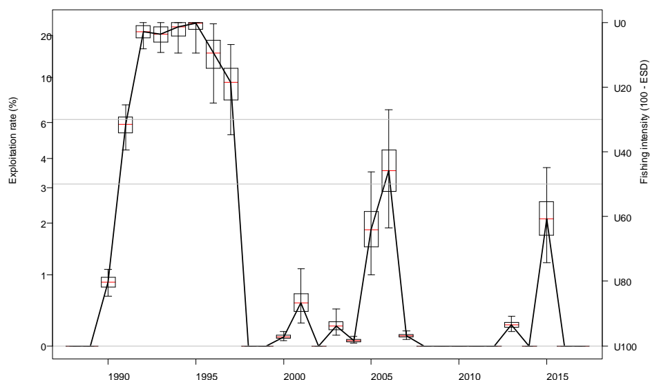
Figure 30: Puysegur base, MCMC estimated fishing-intensity trajectory. The box in each year covers 50% of the distribution and the whiskers extend to 95% of the distribution. The fishing-intensity range associated with the biomass target of 30–50% B_0 is marked by horizontal lines.
