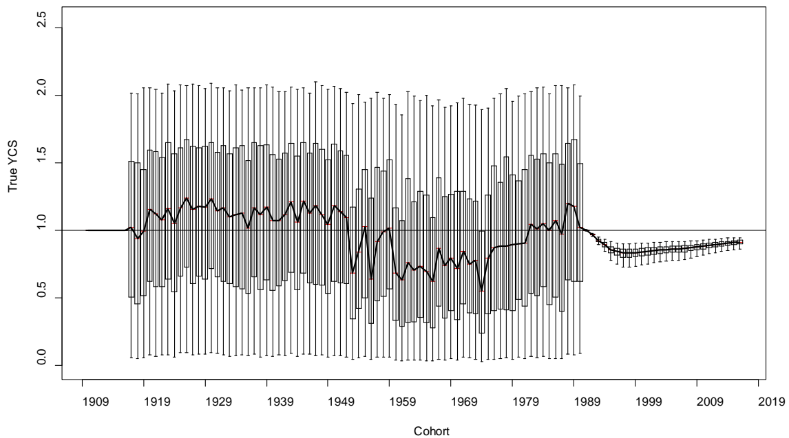
Figure 28: Puysegur base, MCMC estimated “true” YCS ( R_t/R_0 ). The box in each year covers 50% of the distribution and the whiskers extend to 95% of the distribution.
