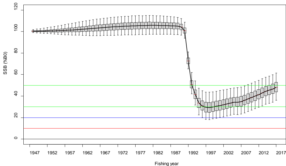
Figure 29: Puysegur base, MCMC estimated spawning-stock biomass trajectory. The box in each year covers 50% of the distribution and the whiskers extend to 95% of the distribution. The hard limit (red), soft limit (blue), and biomass target range (green) are marked by horizontal lines.
