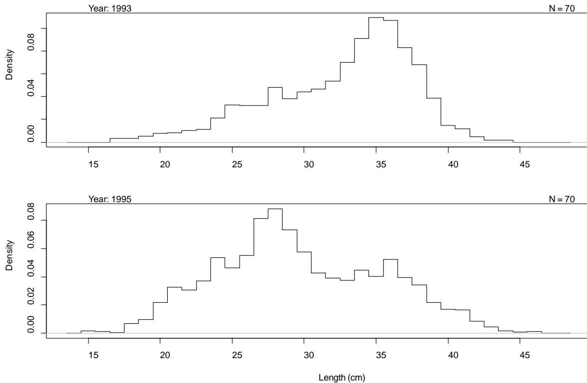
Figure 26: Puysegur: length frequencies for the Tangaroa trawl surveys in 1992 and 1994 (fitted in the model as beginning of year in 1993 and 1995). The effective sample sizes of N = 70 were the approximate number of stations in each survey.
