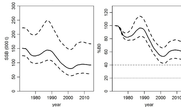
Figure 17: Ling, Chatham Rise — Estimated median trajectories (with 95% credible intervals shown as dashed lines) for absolute spawning biomass and biomass as a percentage of B_0 . Horizontal lines in the right panels show the management target of 40% B_0 and the soft limit of 20% B_0 .
