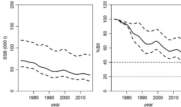
Figure 23: Ling, West Coast South Island, Lognormal CPUE & M=0.18 model — Estimated median trajectories (with 95% credible intervals shown as dashed lines) for absolute spawning biomass and biomass as a percentage of B_0 . Horizontal lines in the right panels show the management target of 40% B_0 and the soft limit of 20% B_0 .
