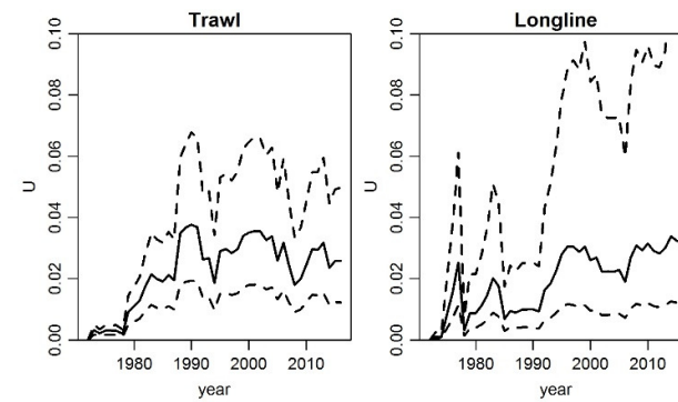
Figure 24: Ling, West Coast South Island, Combined CPUE model — Estimated median trajectory of fishing intensity (with 95% credible intervals shown as dashed lines).
