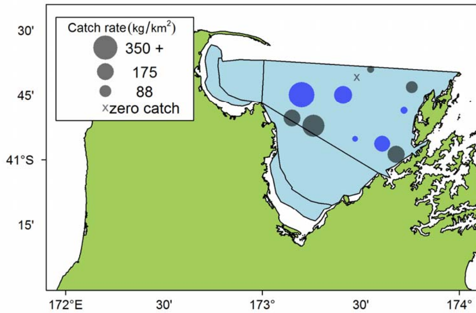
Appendix 5 continued: Catch rates of snapper caught in stratum 19 showing phase 1 (black circles) and phase 2 (blue circles) separately.
