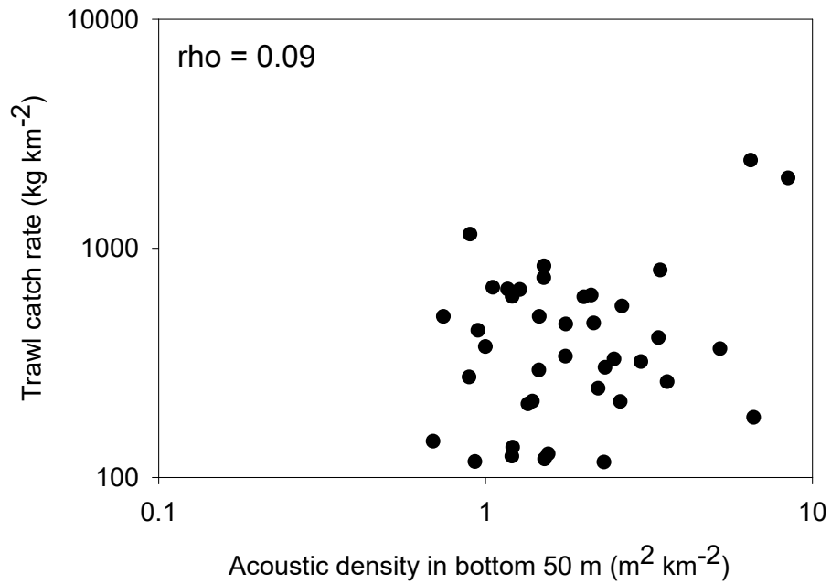
Figure 16: Relationship between total trawl catch rate (all species excluding benthic invertebrates) and acoustic backscatter recorded during the trawl in the Sub-Antarctic in 2016. Rho value is the Spearman's rank correlation coefficient.
