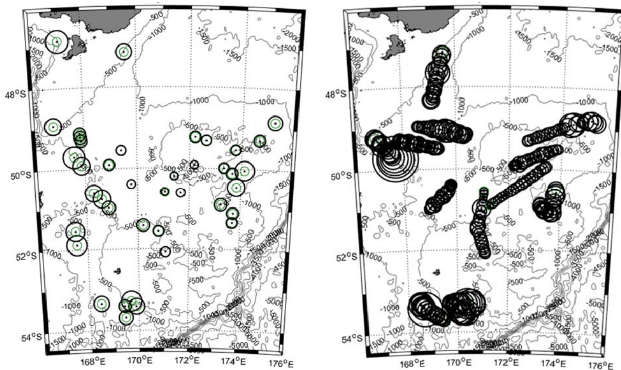
Figure 13: Spatial distribution of total acoustic backscatter ( \text{m}^2 \text{km}^{-2} ) in the Sub-Antarctic observed during day trawl stations (left panel) and night steams (right panel). Circle area is proportional to the acoustic backscatter. Maximum circle size is 154 \text{ m}^2 \text{km}^{-2} .
