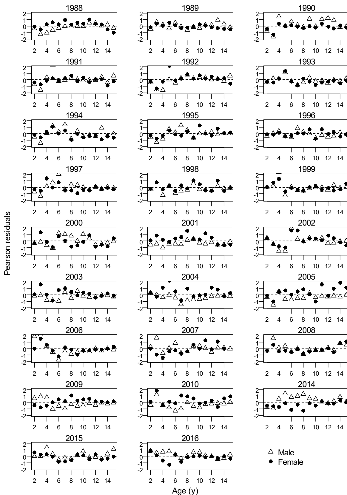
Figure 80: MPD Pearson residuals for the fits to Espage data in run 1.1 (estimate process error).
