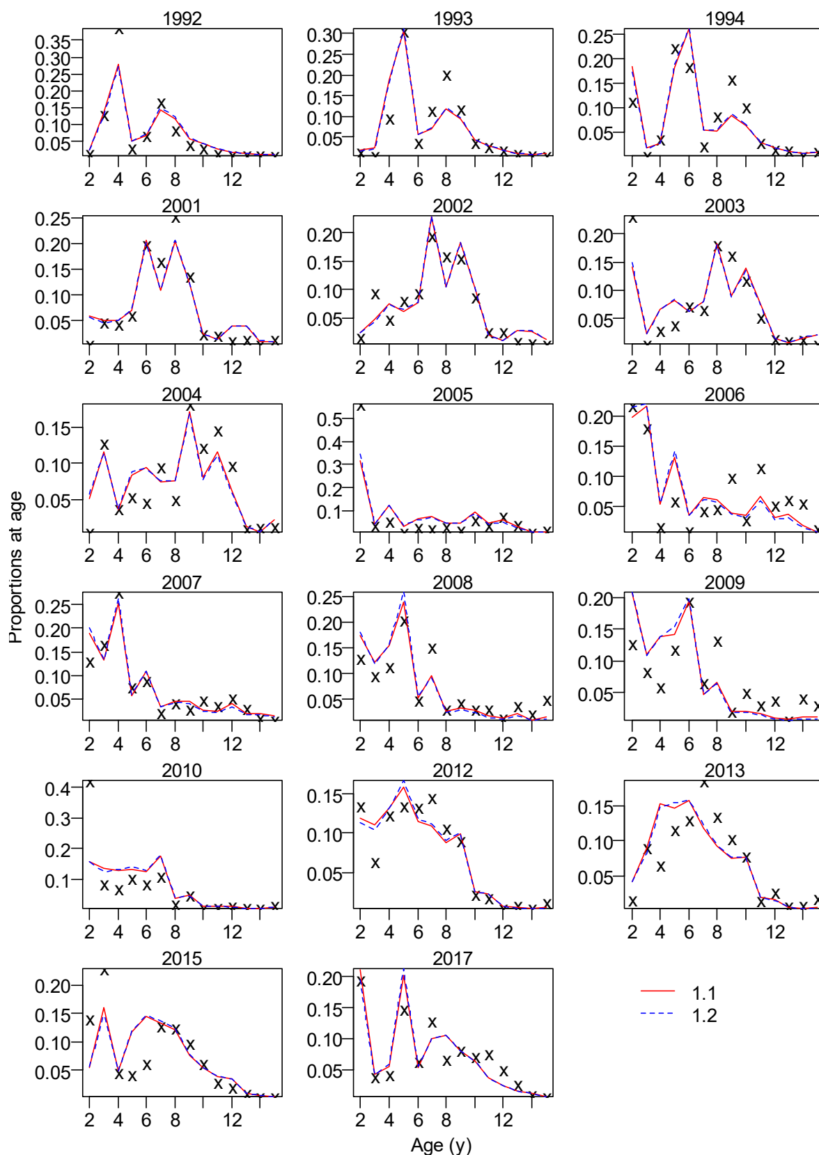
Figure 76: MPD fits to the SAsuage data. Observed ('x') and expected (lines) for runs 1.1 (red solid lines) and 1.2 (blue broken lines). Note that the expected value lines overlap substantially. Male and female observed and expected proportions are summed for an age group.
