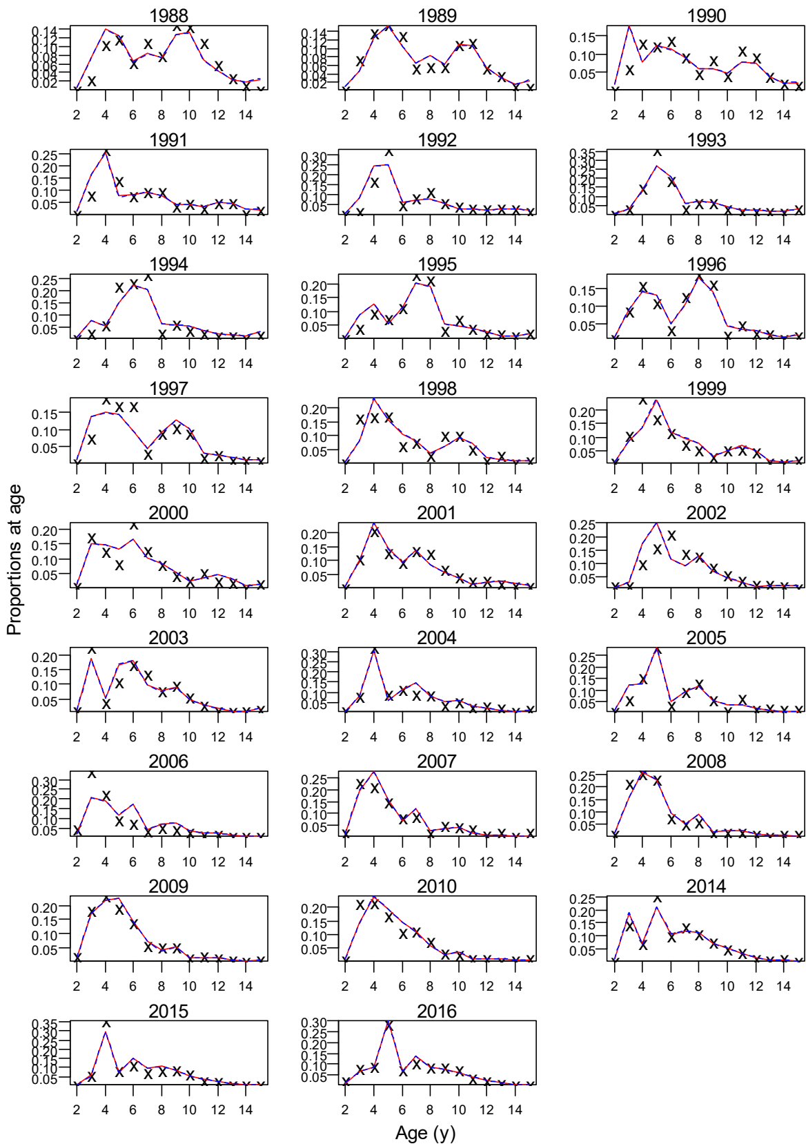
Figure 79: MPD fits to the Espace data. Observed ('x') and expected (lines) for runs 1.1 (red solid lines) and 1.2 (blue broken lines). Note that the expected value lines overlap substantially. Male and female observed and expected proportions are summed for an age group.
