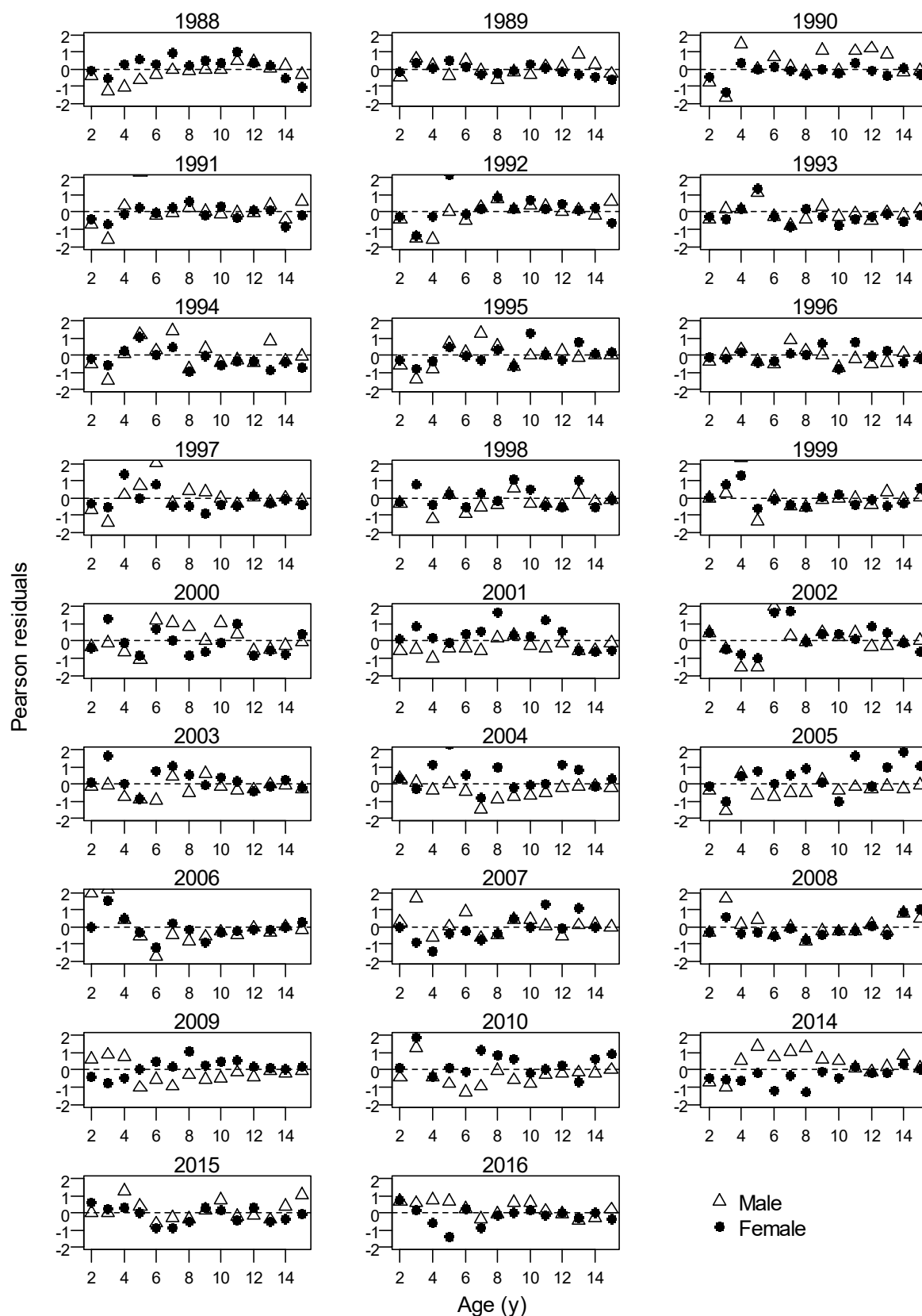
Figure 81: MPD Pearson residuals for the fits to Espage data in run 1.2 (process error 0.20).
