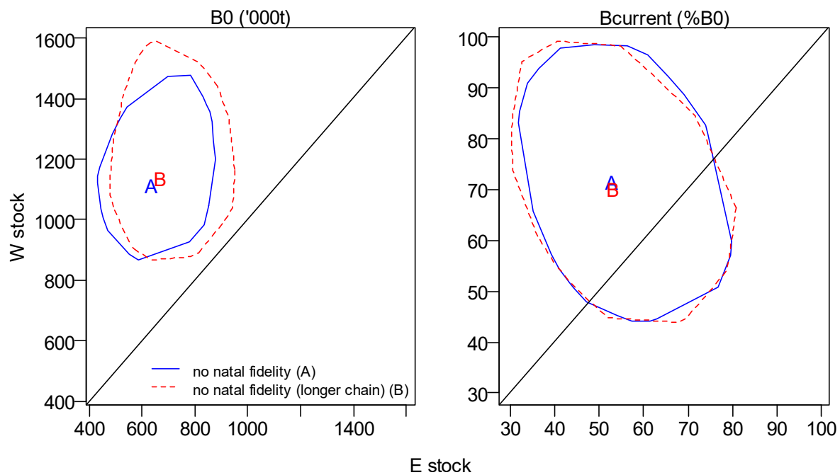
Figure 68: Estimates and approximate 95% confidence intervals for virgin ( B_0 ) and current ( B_{\text{current}} as \%B_0 ) biomass by stock for the no natal fidelity model run, for a chain of length 4 million (A), and longer chain of length 22.5 million (B). In each panel the points 'A' and 'B' indicate best estimates (median of the posterior distribution) for these two runs, and the polygons (with solid, broken and dotted lines, respectively) enclose approximate 95% confidence intervals. Diagonal lines indicate equality ( y = x ).
