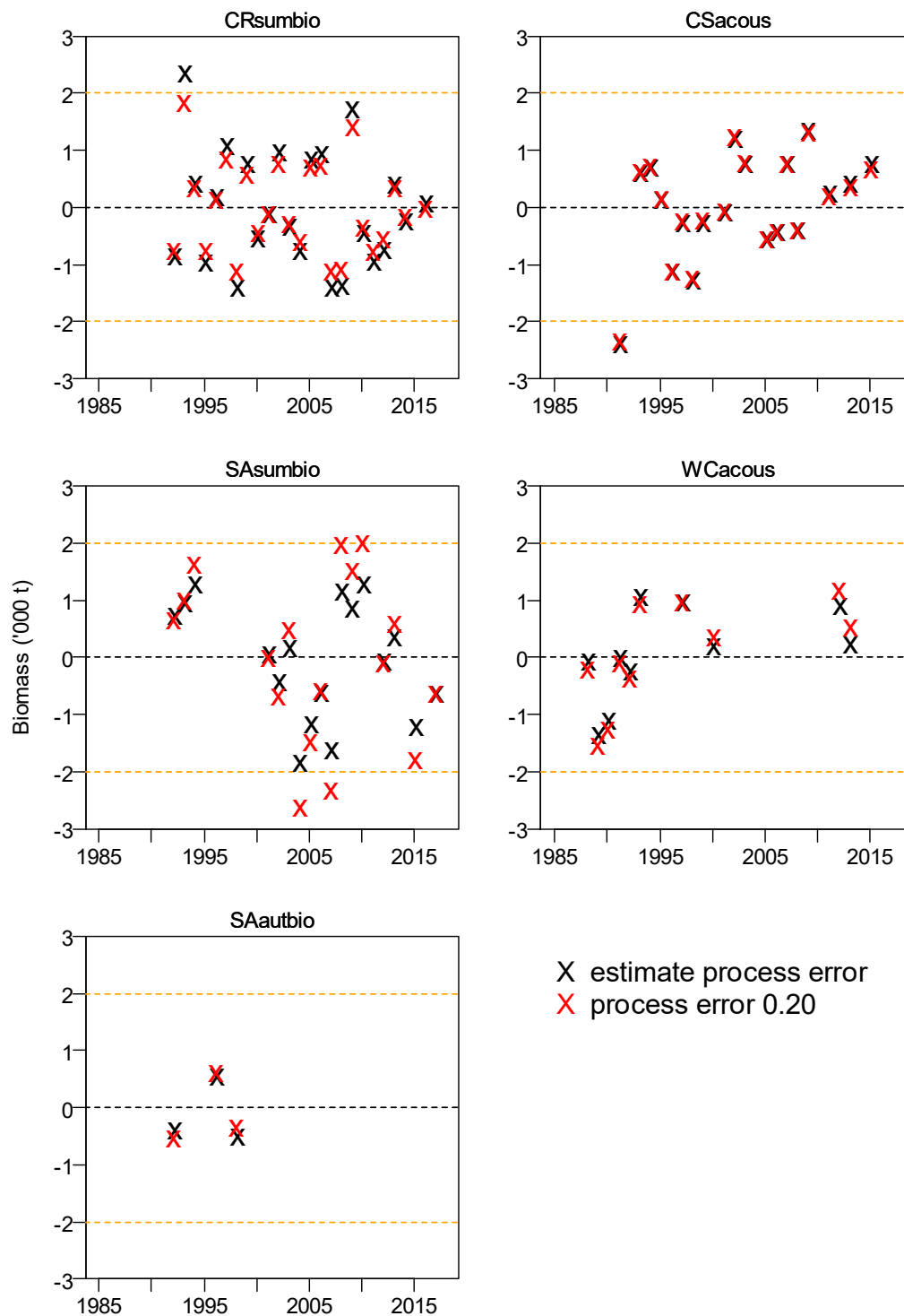
Figure 31: Normalised residuals for fits to biomass indices for 2017 assessment run 1.1 (estimate process error) and 1.2 (process error 0.20).
