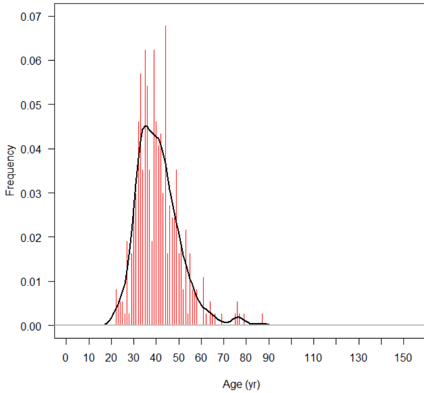
Figure 3: 2016 Rekohu Plume estimated age frequency (red bars) with a smoothed density through the age estimates (black curve).
