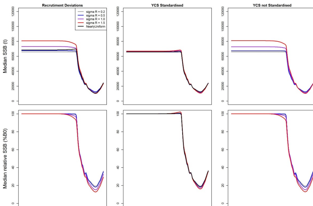
Figure 8: Absolute and relative median SSB trajectories for converged MCMC runs for the ORH-like assessment.
