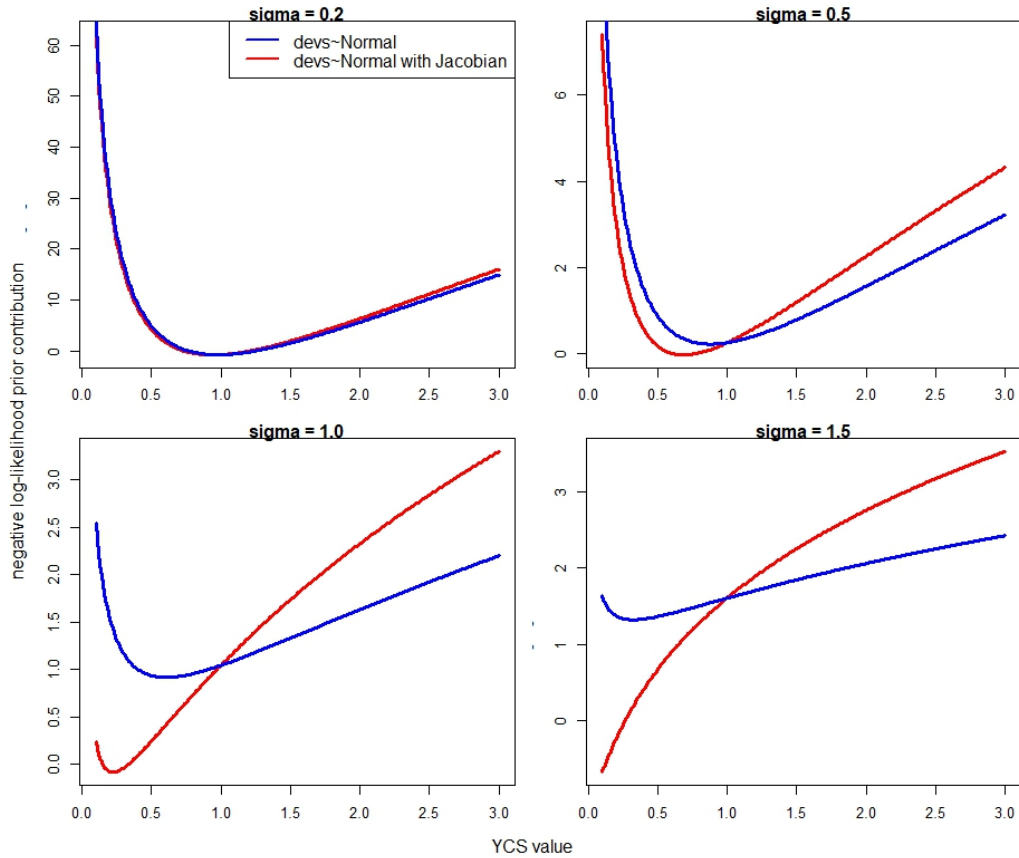
Figure 3: Comparison of negative log-likelihood prior contributions for a given YCS value, when the Jacobian is included (red) and excluded (blue).
