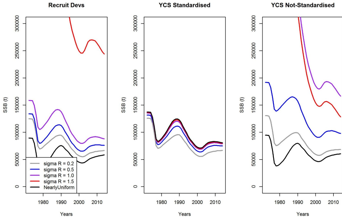
Figure 7: SSB trajectories for the LIN-like assessment after an MPD estimation for each scenario.
