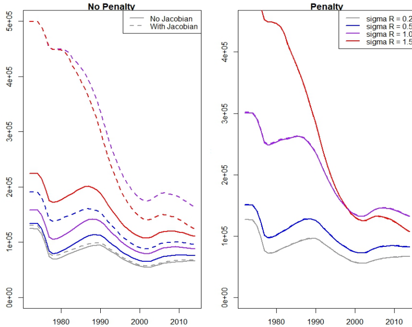
Figure 4: The implications of adding penalties to MPD estimates of SSB(t) and whether or not the Jacobian has been included in the objective function (results shown are for the ling based assessment).
