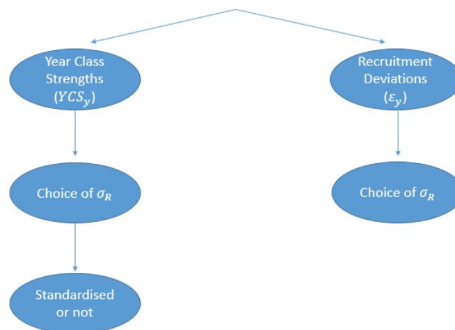
Figure 1: A diagram showing the different parameterisations run for the stock recruitment residuals.
