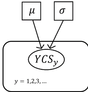
Figure 2: A directed acyclic graph demonstrating the relationship between priors and estimated parameters for a current Bayesian model, where squares indicate fixed constants and circles represent estimated parameters.
