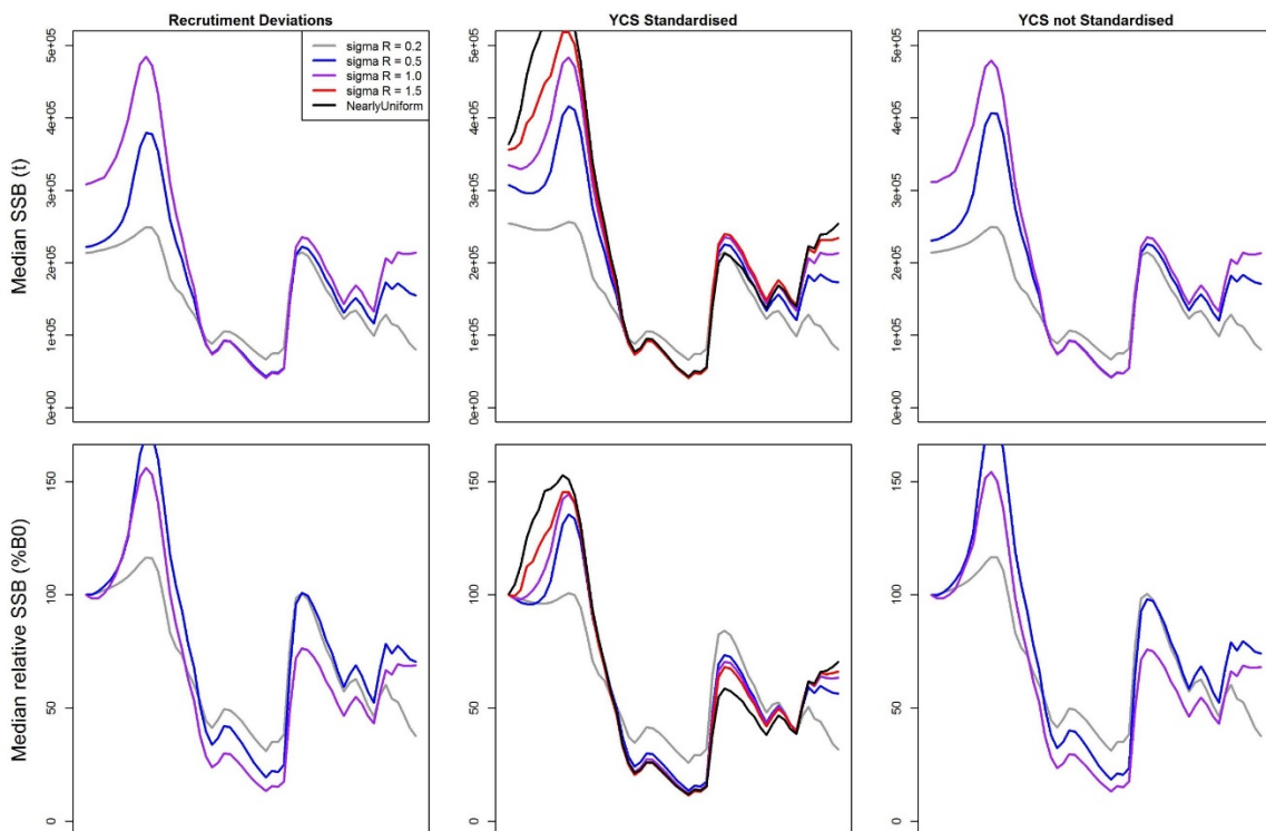
Figure 9: Absolute and relative median SSB trajectories for converged MCMC runs for the SBW-like assessment.
