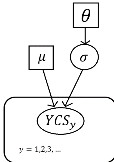
Figure 2: A directed acyclic graph demonstrating the relationship between priors and estimated parameters for a Bayesian hierarchical model. Squares indicate fixed constants and circles represent estimated parameters.
