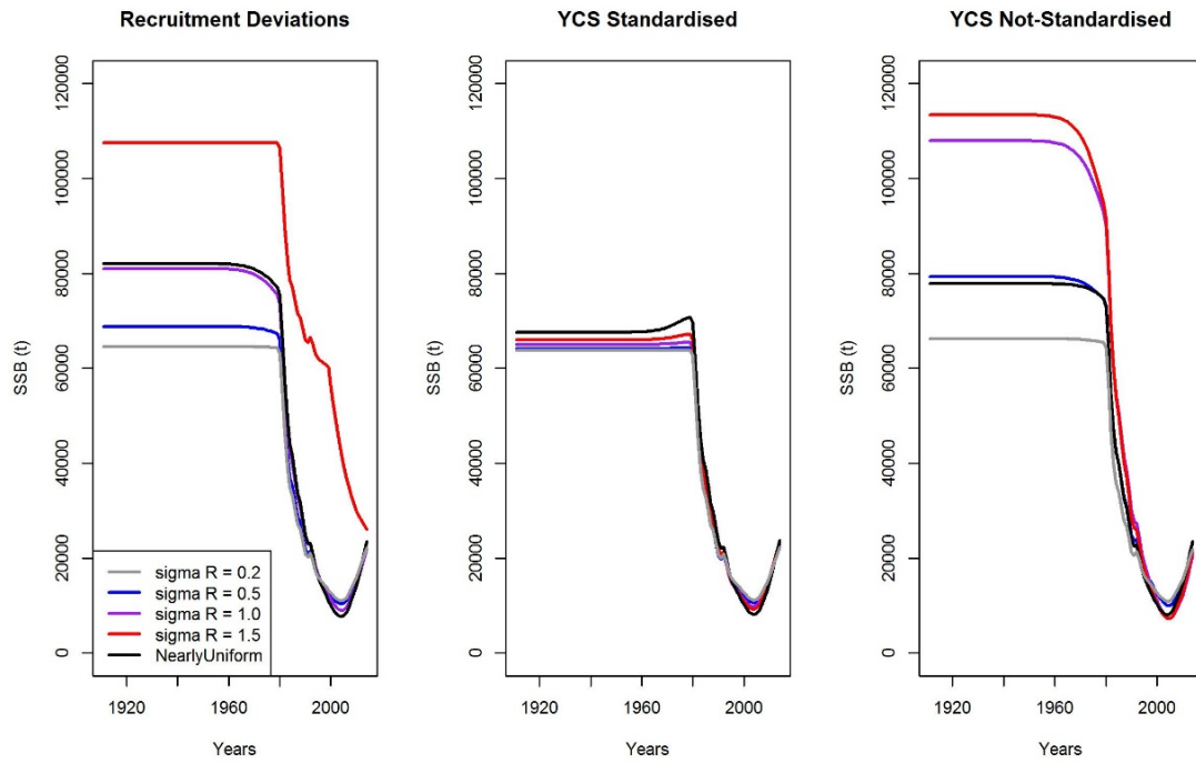
Figure 5: SSB trajectories for the ORH-like assessment after an MPD estimation for each scenario.
