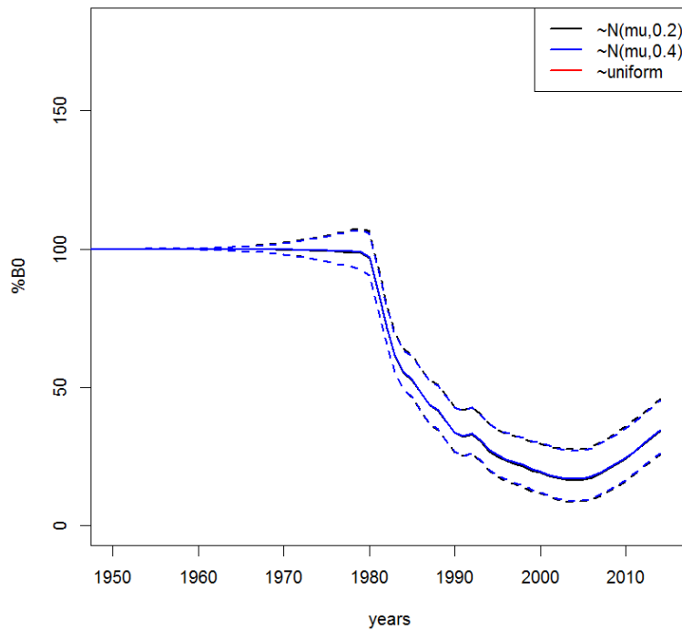
Figure 11: Relative SSB trajectories with 95% credible intervals for the ORH-like assessment using different hyper-priors on \sigma_R .
