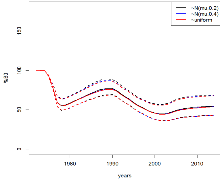
Figure 14: Relative SSB trajectories with 95% credible for the LIN-like assessment using different hyper-priors on \sigma_R .
