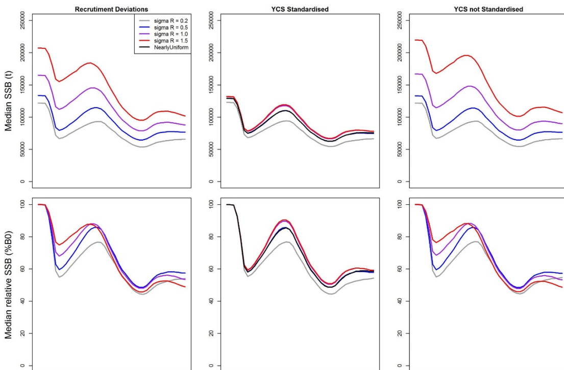
Figure 10: Absolute and relative median SSB trajectories for converged MCMC runs for the LIN-like assessment.
