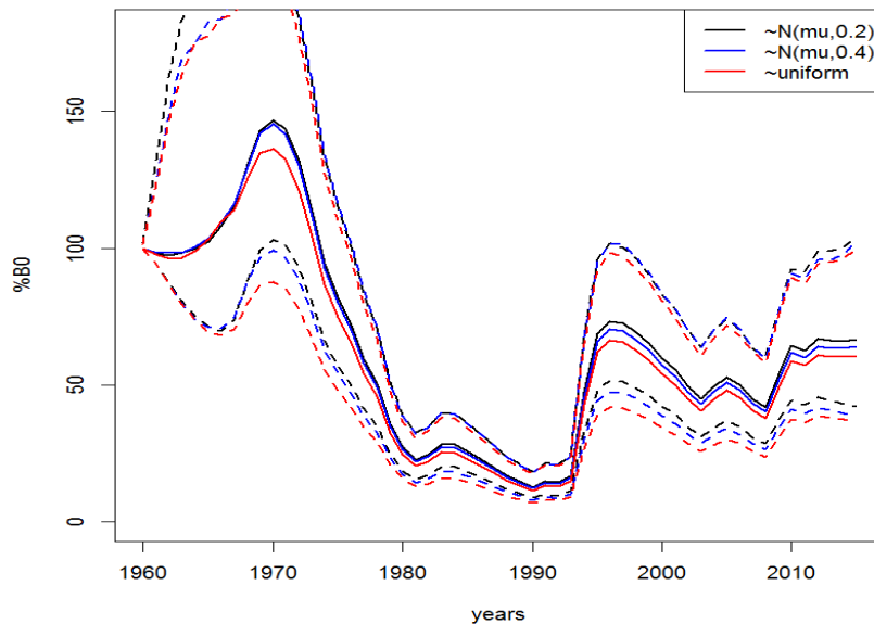
Figure 13: Relative SSB trajectories with 95% credible intervals for the SBW-like assessment using different hyper-priors on \sigma_R .
