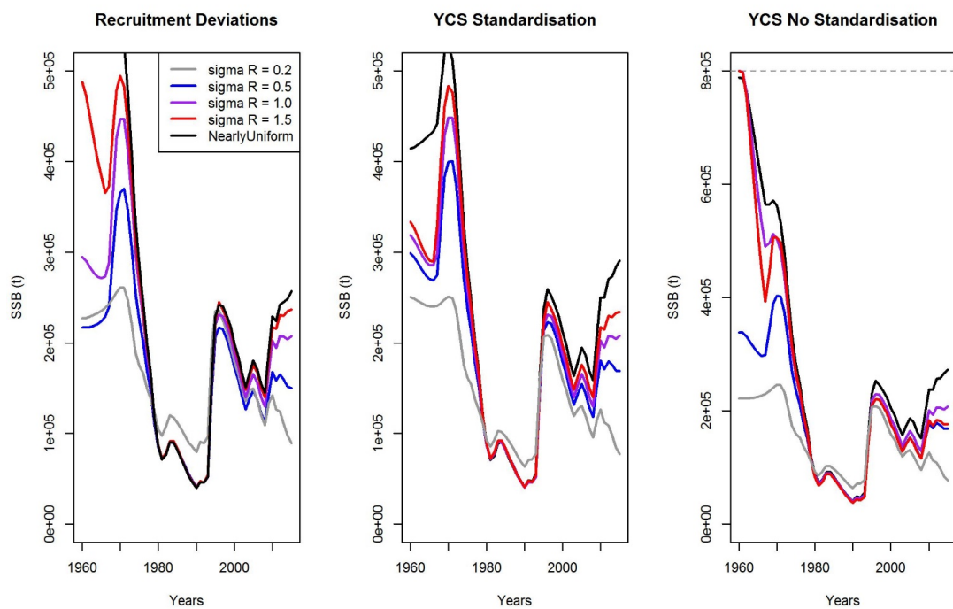
Figure 6: SSB trajectories for the SBW-like assessment after an MPD estimation for each scenario.
