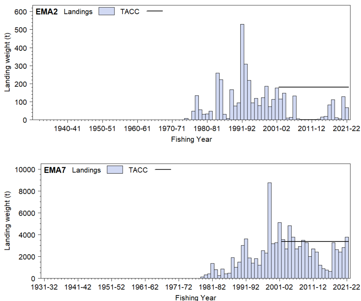
Figure 1 [Continued]: Reported commercial landings and TACC for the three main EMA stocks. From top: EMA 2 (Central East) and EMA 7 (Challenger to Auckland West).
