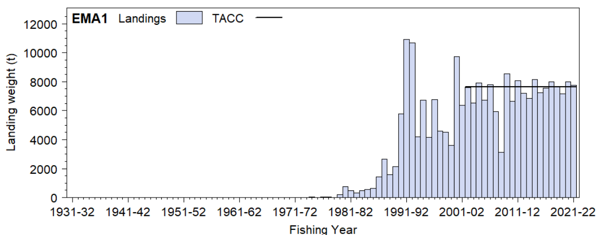
Figure 1: Reported commercial landings and TACC for the three main EMA stocks. EMA 1 (Auckland East). [Continued on next page]
