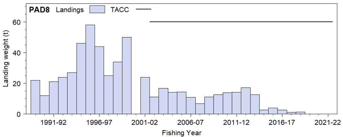
Figure 1 [Continued]: Reported commercial landings and TACCs for the six main PAD stocks: PAD 3 (south East Coast), PAD 5 (Southland), PAD 7 (Challenger) and PAD 8 (Central Egmont).
