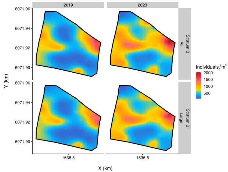
Figure C-5: Predicted cockle densities from the spatio-temporal model for Hokianga Harbour. Predictions are shown for all and for large cockles ( \geq 30 mm shell length) for each year the site was surveyed (since 2013–14, when high-resolution spatial data became available). Fishing years are indicated by the end year, e.g., 2023 refers to the 2022–23 fishing year.
