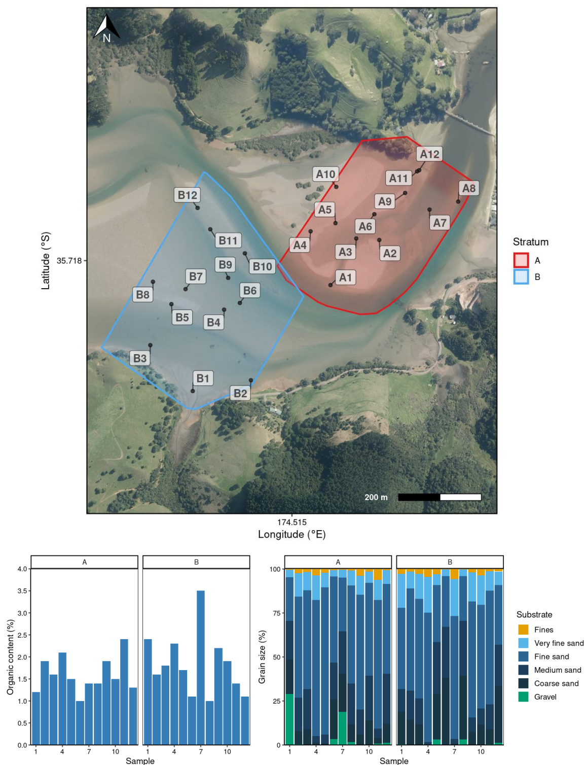
Figure 46: Sediment sample locations and characteristics at Pataua Estuary. Labels correspond to stratum and sample number. Graphs show organic content (% dry weight) and cumulative grain size (%). Sediment grain size fractions include fines (silt and clay, \leq 63 \mu\text{m} ), sands (very fine, >63 \mu\text{m} ; fine, >125 \mu\text{m} ; medium, >250 \mu\text{m} ; coarse, >500 \mu\text{m} ), and gravel ( >2000 \mu\text{m} ) (see details in Table B-1).
