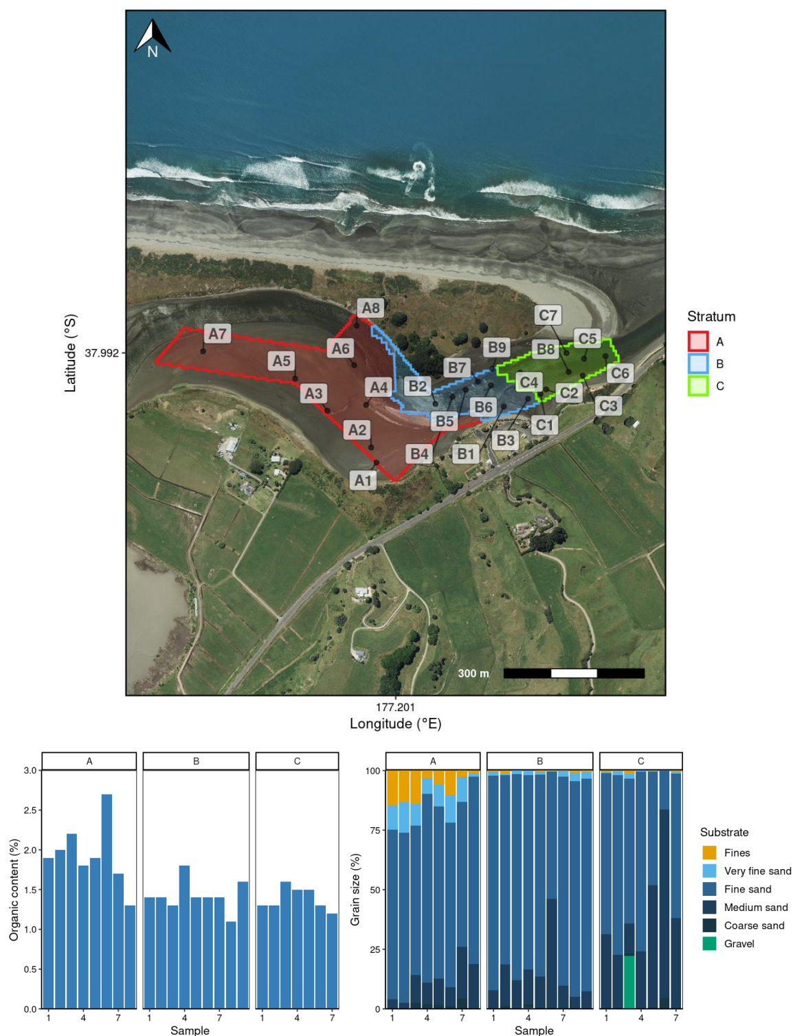
Figure 52: Sediment sample locations and characteristics at Waioata Estuary. Labels correspond to stratum and sample number. Graphs show organic content (% dry weight) and cumulative grain size (%). Sediment grain size fractions include fines (silt and clay, \leq 63 \mu\text{m} ), sands (very fine, >63 \mu\text{m} ; fine, >125 \mu\text{m} ; medium, >250 \mu\text{m} ; coarse, >500 \mu\text{m} ), and gravel ( >2000 \mu\text{m} ) (see details in Table B-1).
