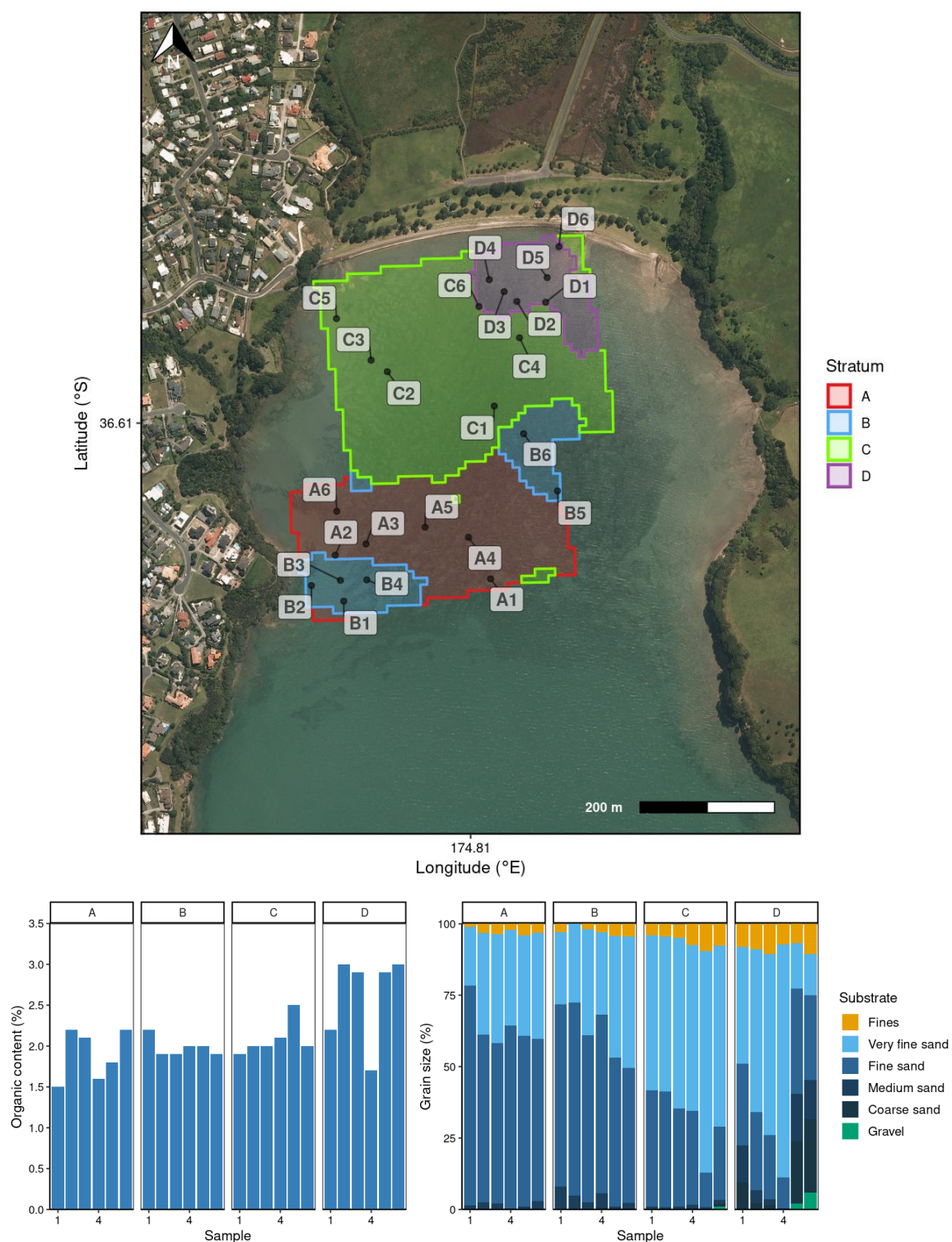
Figure 36: Sediment sample locations and characteristics at Okoromai Bay. Labels correspond to stratum and sample number. Graphs show organic content (% dry weight) and cumulative grain size (%). Sediment grain size fractions include fines (silt and clay, \leq 63 \mu\text{m} ), sands (very fine, >63 \mu\text{m} ; fine, >125 \mu\text{m} ; medium, >250 \mu\text{m} ; coarse, >500 \mu\text{m} ), and gravel ( >2000 \mu\text{m} ) (see details in Table B-1).
