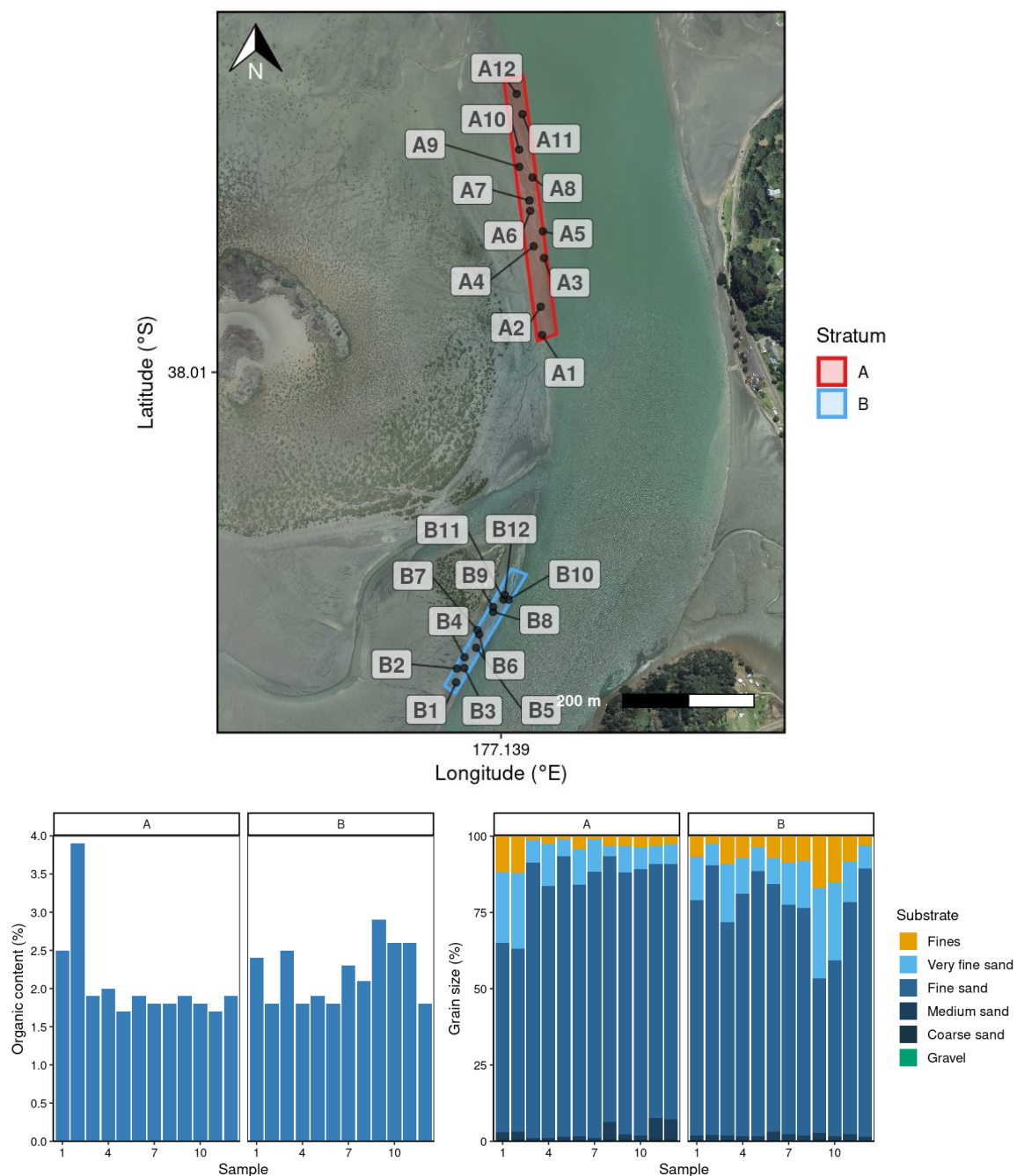
Figure 30: Sediment sample locations and characteristics at Ōhiwa Harbour. Labels correspond to stratum and sample number. Graphs show organic content (% dry weight) and cumulative grain size (%). Sediment grain size fractions include fines (silt and clay, \leq 63 \mu\text{m} ), sands (very fine, > 63 \mu\text{m} ; fine, > 125 \mu\text{m} ; medium, > 250 \mu\text{m} ; coarse, > 500 \mu\text{m} ), and gravel ( > 2000 \mu\text{m} ) (see details in Table B-1).
