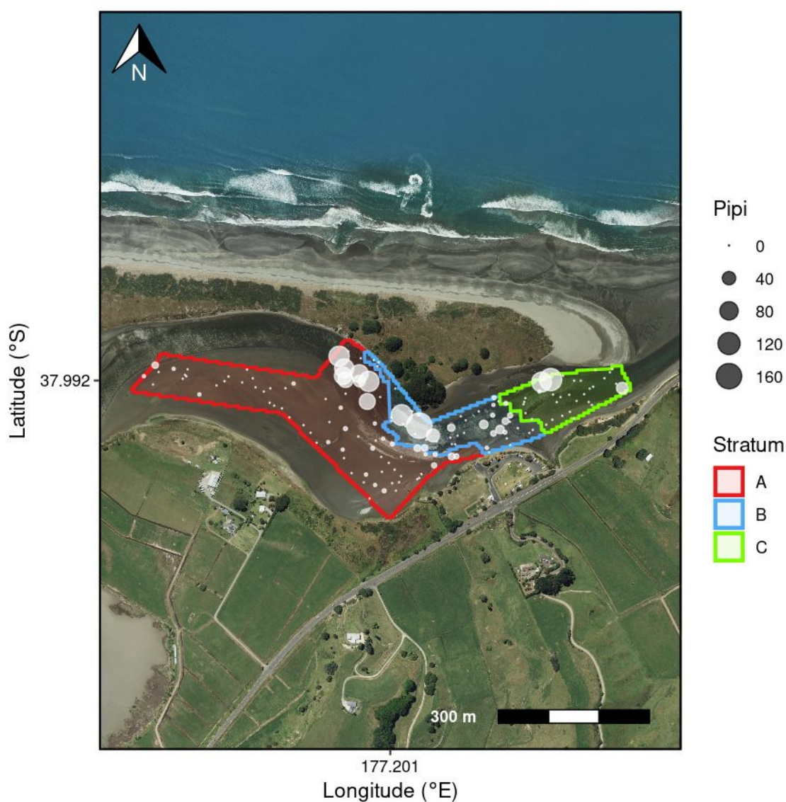
Figure 56: Map of sample strata and individual sample locations for pipi at Waioatahe Estuary, with the size of the circles proportional to the number of pipi (per 0.035 m 2 ) found at each location. Samples with zero counts are shown as small dots.
