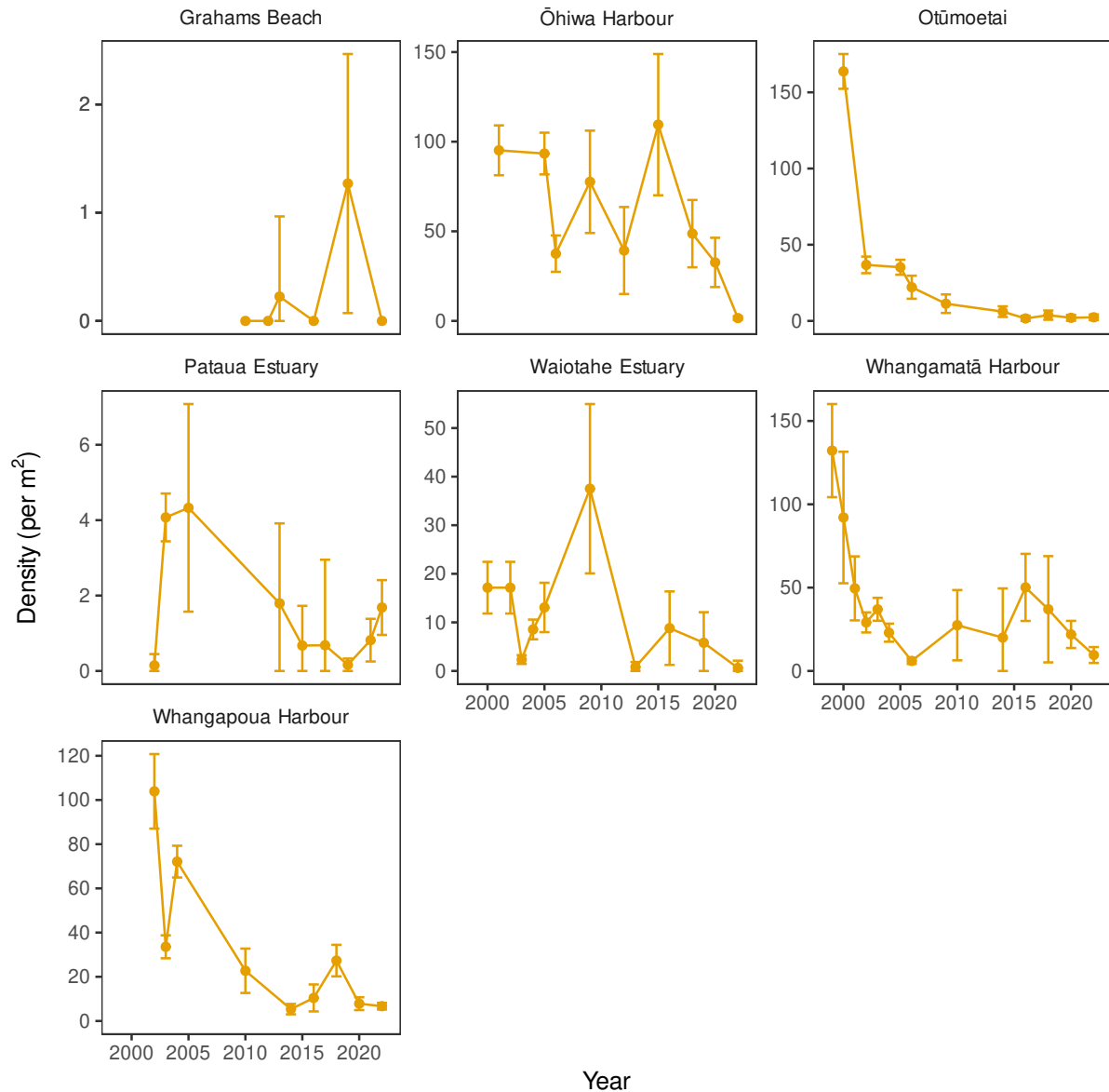
Figure 75: Estimated density of large pipi (≥50 mm shell length) for all sites where pipi in this size class were present in at least one survey. Shown are the mean estimated densities across years, with bars indicating the 95% confidence interval. (Note, different scales on the y-axes. Not all sites were surveyed each year, and the sampling extent may vary across years.)
