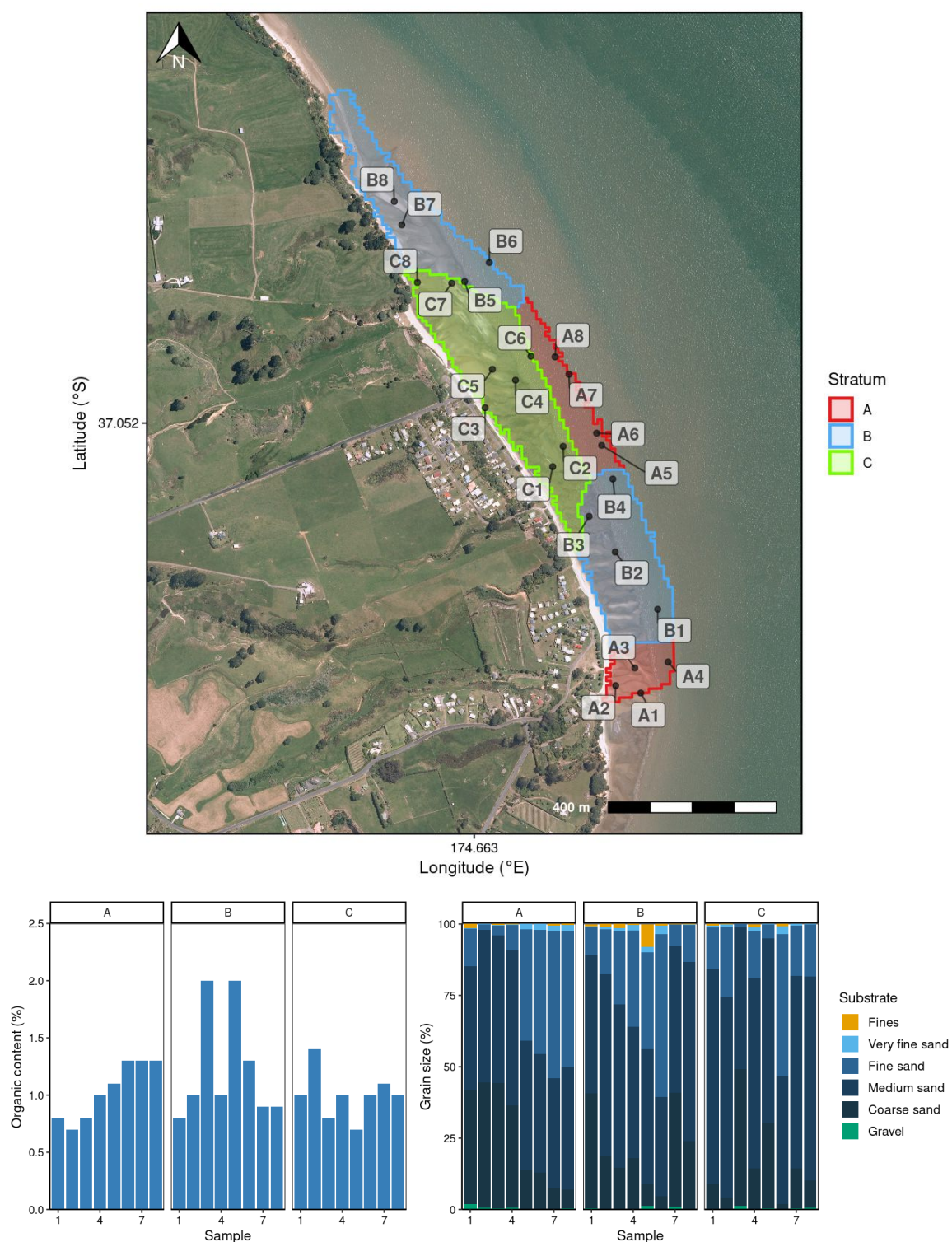
Figure 14: Sediment sample locations and characteristics at Grahams Beach. Labels correspond to stratum and sample number. Graphs show organic content (% dry weight) and cumulative grain size (%). Sediment grain size fractions include fines (silt and clay, \leq 63 \mu\text{m} ), sands (very fine, >63 \mu\text{m} ; fine, >125 \mu\text{m} ; medium, >250 \mu\text{m} ; coarse, >500 \mu\text{m} ), and gravel ( >2000 \mu\text{m} ) (see details in Table B-1).
