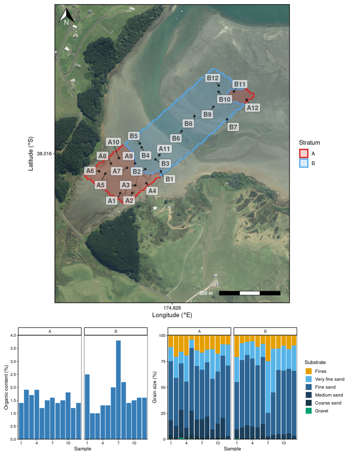
Figure 2: Sediment sample locations and characteristics at Aotea Harbour. Labels correspond to stratum and sample number. Graphs show organic content (% dry weight) and cumulative grain size (%). Sediment grain size fractions include fines (silt and clay, \leq 63 \mu\text{m} ), sands (very fine, >63 \mu\text{m} ; fine, >125 \mu\text{m} ; medium, >250 \mu\text{m} ; coarse, >500 \mu\text{m} ), and gravel ( >2000 \mu\text{m} ) (see details in Table B-1).
