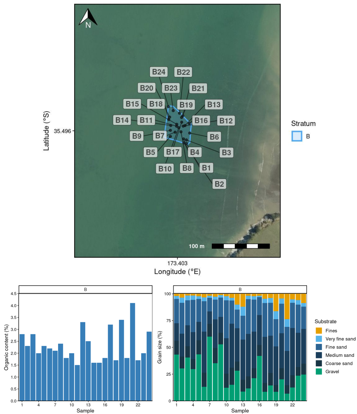
Figure 20: Sediment sample locations and characteristics at Hokianga Harbour. Labels correspond to stratum and sample number. Graphs show organic content (% dry weight) and cumulative grain size (%). Sediment grain size fractions include fines (silt and clay, \leq 63 \mu\text{m} ), sands (very fine, >63 \mu\text{m} ; fine, >125 \mu\text{m} ; medium, >250 \mu\text{m} ; coarse, >500 \mu\text{m} ), and gravel ( >2000 \mu\text{m} ) (see details in Table B-1).
