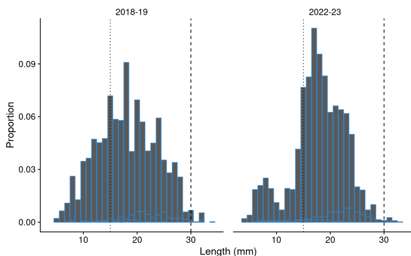
Figure 22: Weighted length-frequency (LF) distribution of cockles for the present survey at Hokianga Harbour. Vertical dotted and dashed lines indicate the cut-off sizes for recruits and large individuals, respectively.
