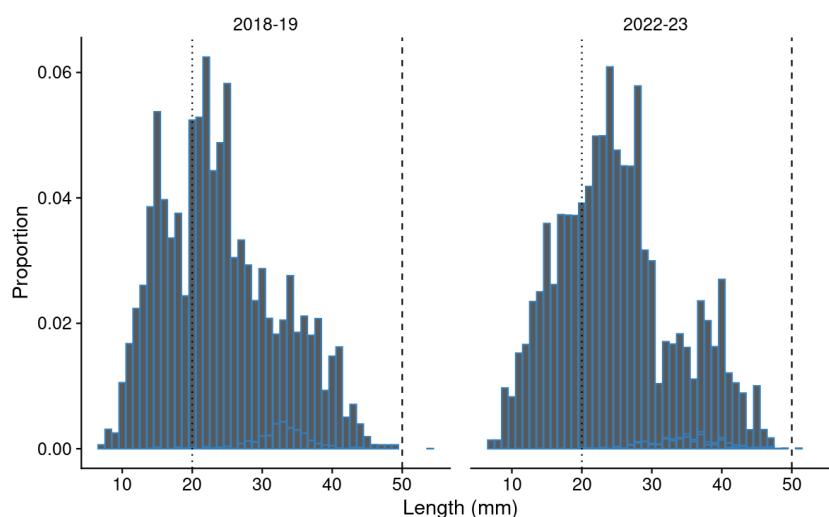
Figure 25: Weighted length-frequency (LF) distribution of pipi for the present survey at Hokianga Harbour. Vertical dotted and dashed lines indicate the cut-off sizes for recruits and large individuals, respectively.
