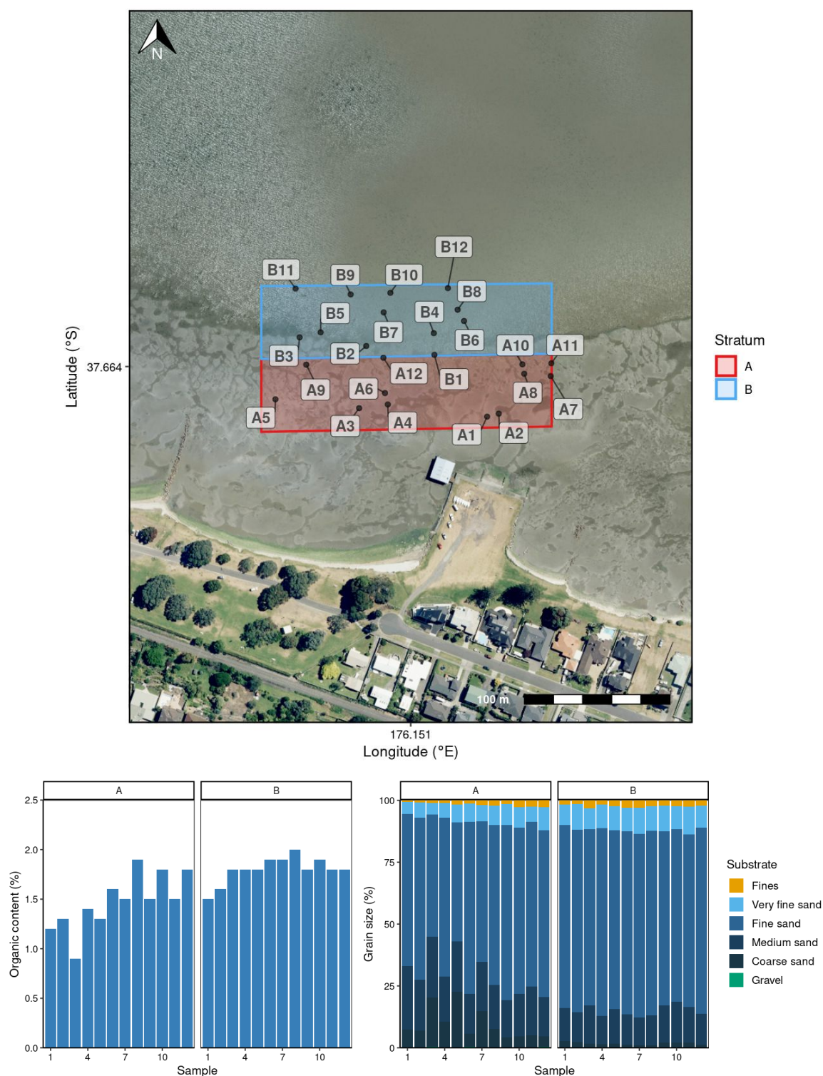
Figure 40: Sediment sample locations and characteristics at Otūmoetai (Tauranga Harbour). Labels correspond to stratum and sample number. Graphs show organic content (% dry weight) and cumulative grain size (%). Sediment grain size fractions include fines (silt and clay, \leq 63 \mu\text{m} ), sands (very fine, >63 \mu\text{m} ; fine, >125 \mu\text{m} ; medium, >250 \mu\text{m} ; coarse, >500 \mu\text{m} ), and gravel ( >2000 \mu\text{m} ) (see details in Table B-1).
