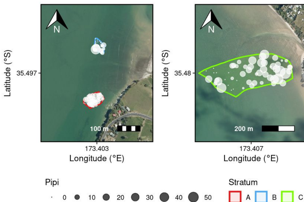
Figure 24: Map of sample strata and individual sample locations for pīpi at Hokianga Harbour, with the size of the circles proportional to the number of pīpi (per 0.035 m 2 ) found at each location. Samples with zero counts are shown as small dots.
