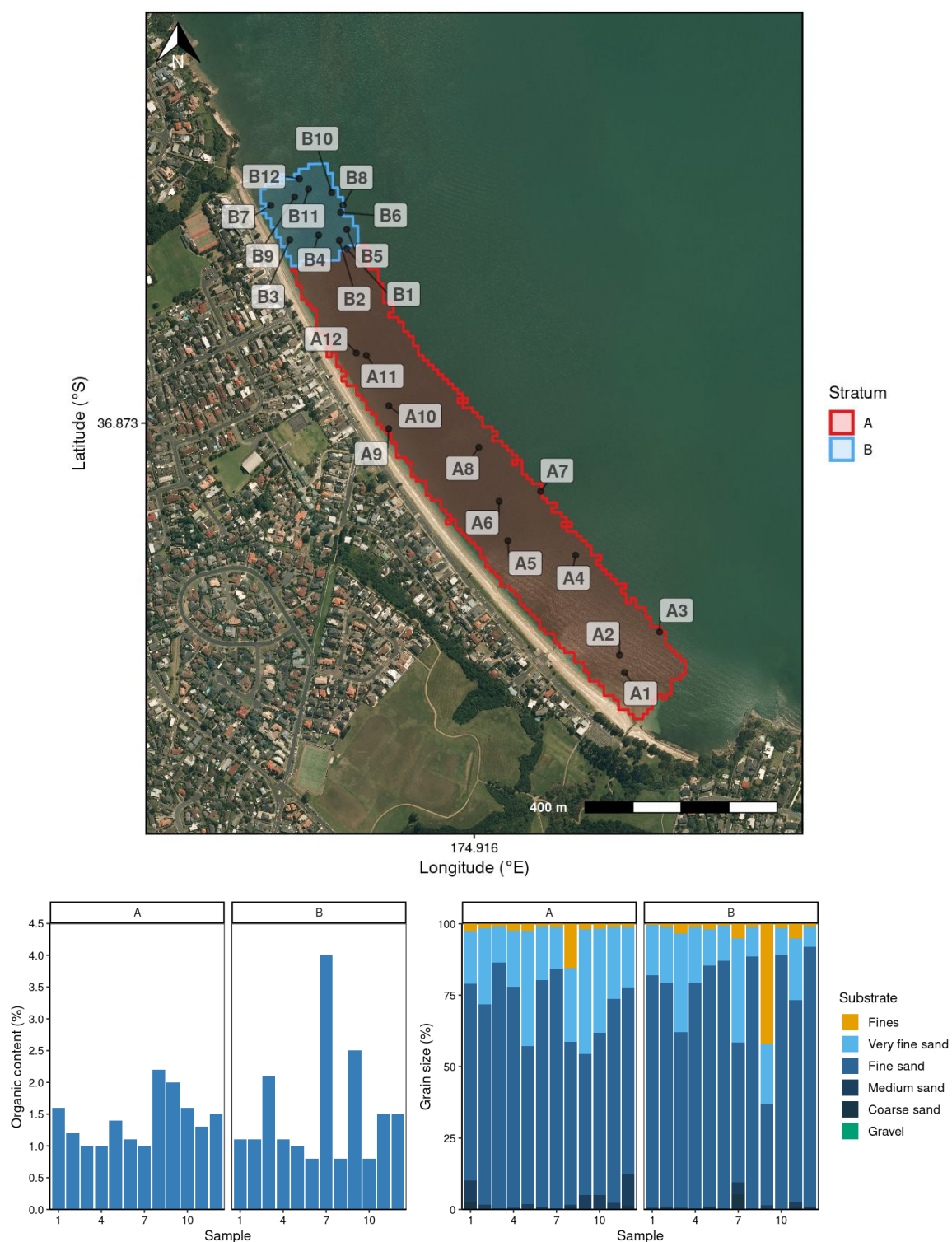
Figure 10: Sediment sample locations and characteristics at Eastern Beach. Labels correspond to stratum and sample number. Graphs show organic content (% dry weight) and cumulative grain size (%). Sediment grain size fractions include fines (silt and clay, \leq 63 \mu\text{m} ), sands (very fine, >63 \mu\text{m} ; fine, >125 \mu\text{m} ; medium, >250 \mu\text{m} ; coarse, >500 \mu\text{m} ), and gravel ( >2000 \mu\text{m} ) (see details in Table B-1).
