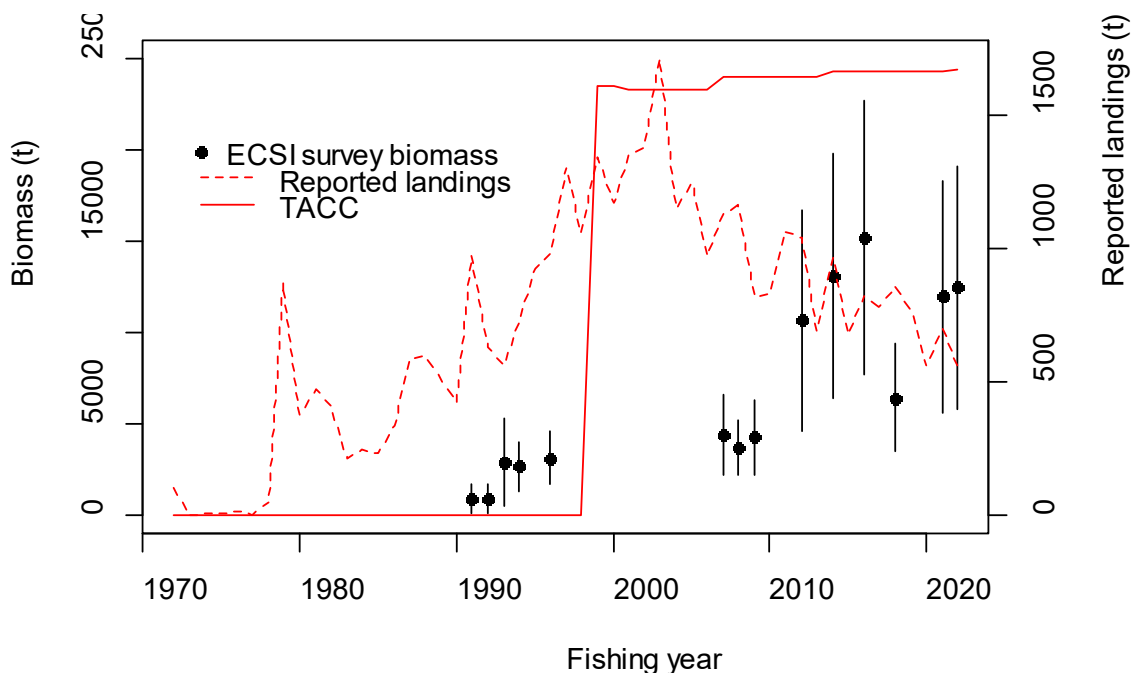
GSH 1–4: Relative biomass from east coast South Island (ECSI) Kaharoa survey. Black circles and vertical lines are \pm 2 s.e.; dashed red line, reported QMR/MHR landings (right axis); solid red line, TACC for GSH 1–4 (right axis).
