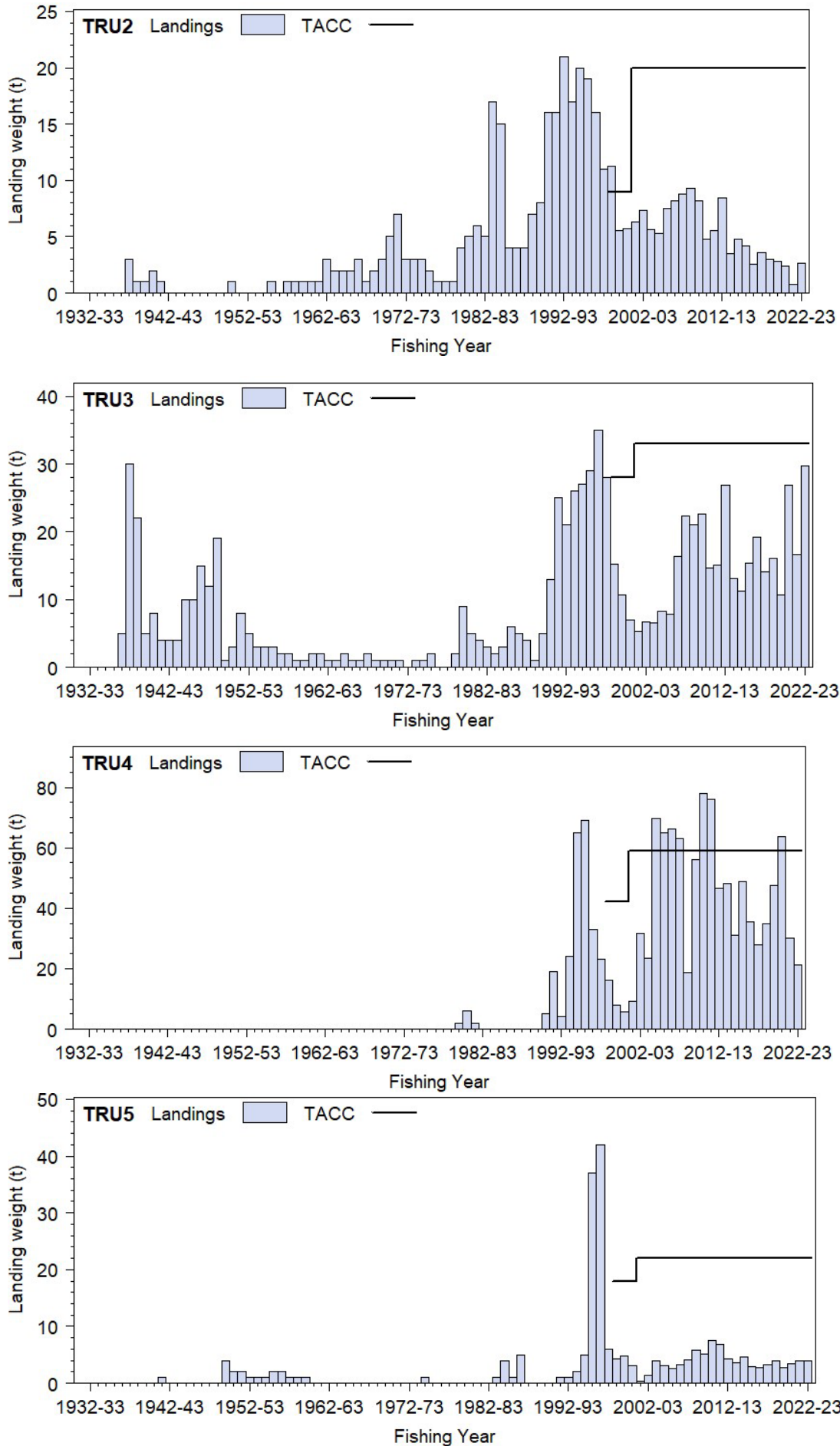
Figure 1: Reported commercial landings and TACCs for the four main TRU stocks. Top to bottom: TRU 2 (Central East), TRU 3 (South East Coast), TRU 4 (South East Chatham Rise), and TRU 5 (Southland).
