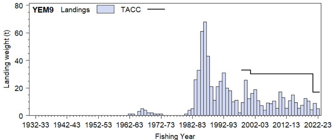
Figure 1: Reported commercial landings and TACCs for the two main YEM stocks. YEM 1 (Auckland East) and YEM 9 (Auckland West).
