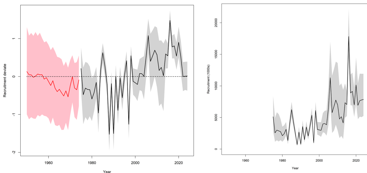
Figure 7: Estimates of annual recruitment deviates (left) and recruitment (numbers of fish, thousands) (right) from the Base Case model (MCMCs). The black line represents the median of the MCMC estimates and the shaded area represents the 95% credibility interval. Recruitment deviates for the initialisation period (1950–1974) are presented in red.
