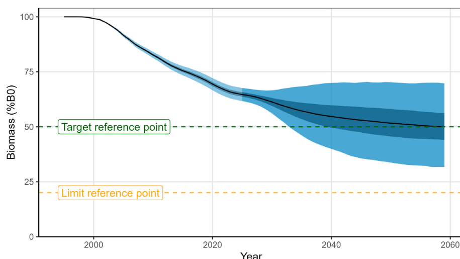
Figure 6: Markov chain Monte Carlo (MCMC) estimate of stock status projected out to 2059 for the base model (R2), with the median (black line), interquartile range (dark blue) and 95% credible intervals (light blue). The target reference point (50% B_0 ) is shown as a green dashed line, and the limit reference point (20% B_0 ) as an orange dashed line.
