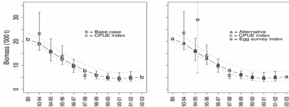
Figure 3: Estimated biomass trajectories for the base case and alternative model runs for the EC stock. Annual biomass estimates are mean posterior density (MPD) values and 95% confidence intervals (grey dashed lines) are calculated from the posterior profile distribution of B_0 estimates. The CPUE index CVs (sampling error plus process error) are shown, as is the CV calculated for the egg survey biomass estimate.
