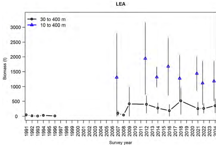
Figure 3: Leatherjacket total biomass for the ECSI winter surveys in core strata (30–400 m), and core plus shallow strata (10–400 m) in 2007, 2012, 2014, 2016, 2018, 2021, 2022, and 2024. Error bars are 2 standard deviations.
