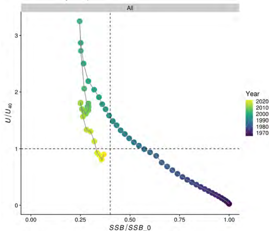
Plot of SSB relative to unfished spawning biomass ( SSB_0 ), and exploitation rate ( U ) relative to exploitation rate at 40% of SSB_0 .
