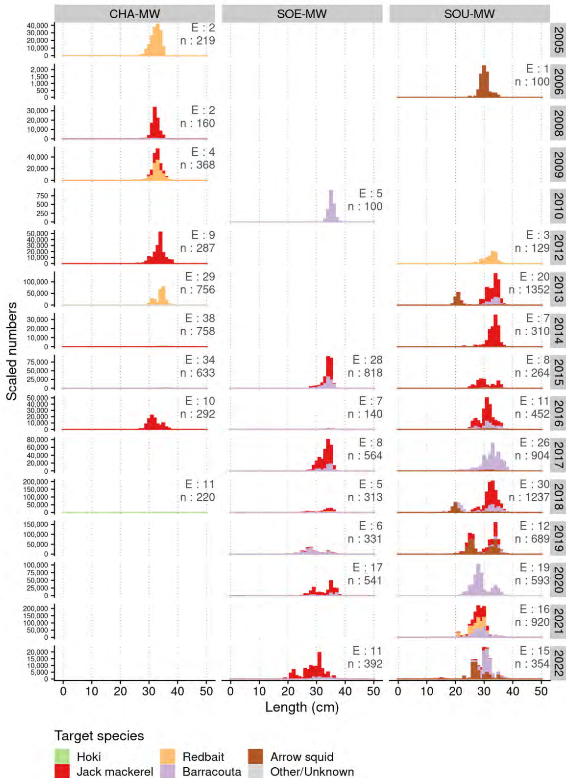
Figure 4: Scaled observer length-frequency distributions for red bait caught in the midwater trawl fishery, by observer region (CHA: Challenger; SOE: eastern Chatham Rise; SOU: Southland), year, and target species (E: Events sampled; n: number of measured fish).
