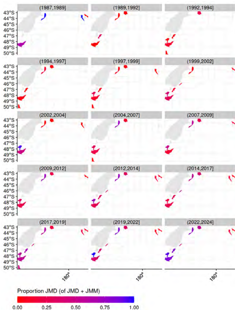
Figure 5: The relative proportions of T. declivis (JMD) and T. murphyi (JMM) from observer sampling in JMA 3. Data were aggregated in regions defined by DBSCAN clustering of the start locations of observed tows.
