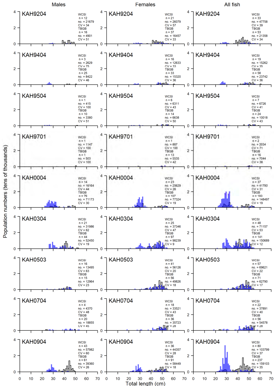
Figure 8: Scaled population length frequency distributions for John dory in 30–400 m for west coast (white bars) and Tasman Bay/Golden Bay (blue bars), from WCSI inshore trawl surveys. n = number of fish measured, no. = scaled population number, CV = coefficient of variation (%). [Continued on next page]
