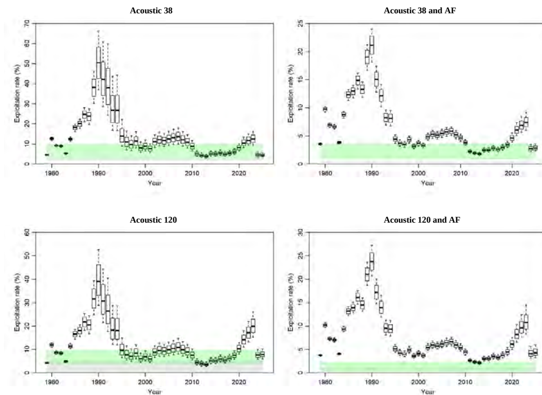
Figure 10: ESCR, MCMC estimated exploitation rate trajectory for the four assessment model runs (boxplot where solid line, median; outer box, interquartile range; whiskers 95% SI) Green (upper) shaded area indicates the exploitation rate corresponding to the target zone ( U_{30} to U_{50} ) after sampling from all year class strengths (1911–2025); Grey (lower) shaded area indicates the exploitation rate corresponding to the target zone ( U_{30} to U_{50} ) after sampling from recent year class strengths (1980–2025).
