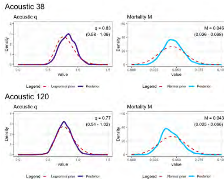
Figure 12: NWCR assessment model runs Acoustic 38 and Acoustic 120, (left) prior (broken line) and MCMC posterior (solid line) for the acoustic q , with text giving the median and 95% credible intervals; (right) prior (broken line) and MCMC posterior (solid line) for natural mortality rate ( M ) with text giving the median and 95% credible intervals.
