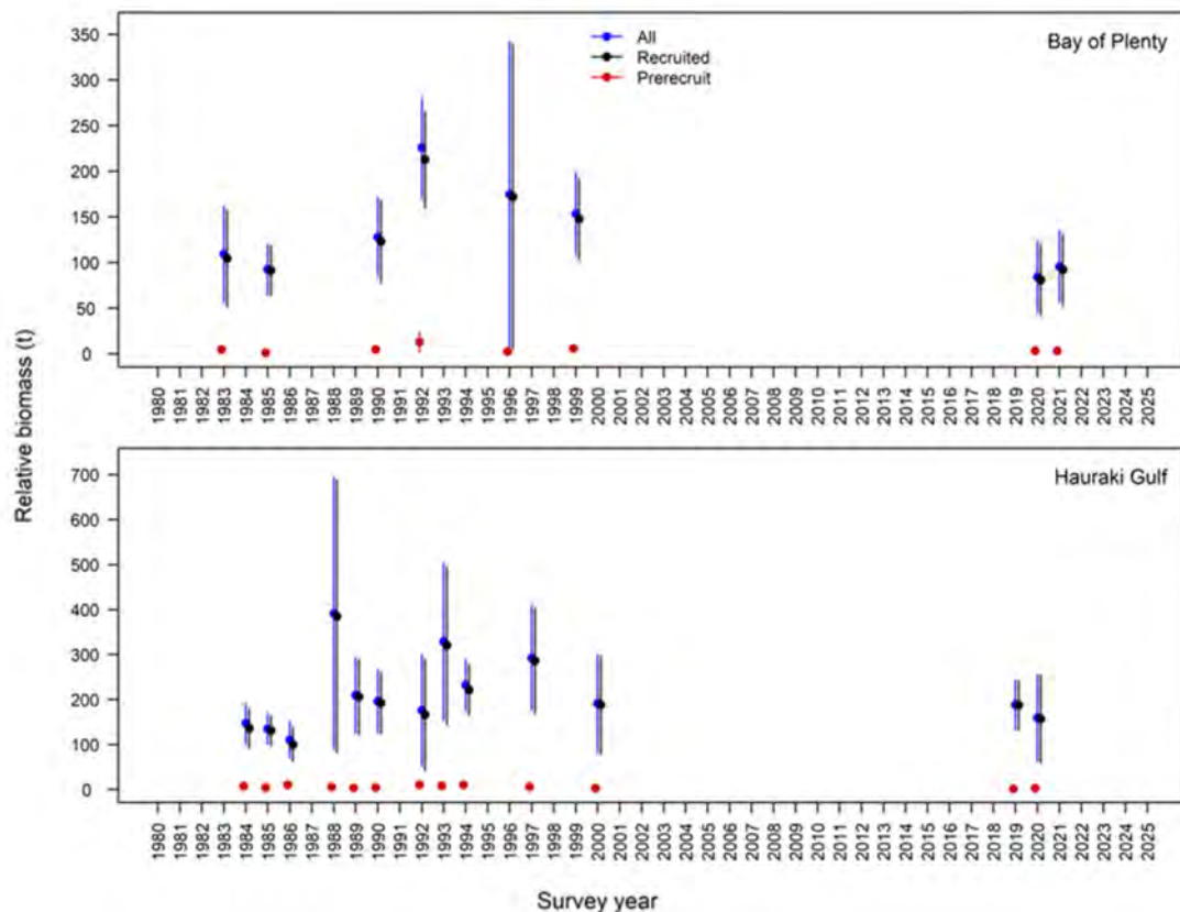
Figure 2: Estimates of recruited (length \geq 25 cm) John dory biomass (t) from Kaharoa trawl surveys with 95% confidence intervals. The 2025 estimate is not part of the time series, conducted from Kaharoa II with different trawl net at a different time of year. [Continued on the next page]
