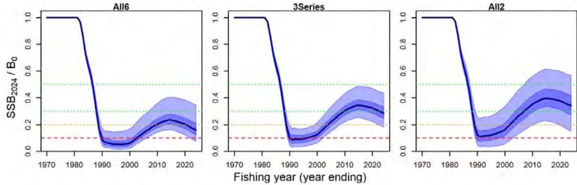
Figure 7: MCMC estimated spawning-stock status ( SSB_{2024}/B_0 ) trajectory. The solid line shows the median, the darker shaded areas covers 50% of the distribution, and the lighter shaded areas 95% of the distribution. The hard limit 10% B_0 (dashed red), soft limit 20% B_0 (dotted orange), and biomass target range 30–50% B_0 (green) are marked by horizontal lines.
