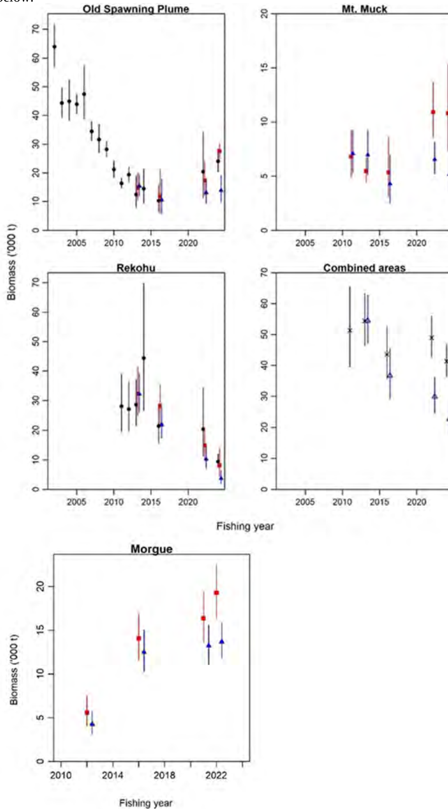
Figure 5: Acoustic biomass estimates for Chatham Rise orange roughy. Combined areas is the Old Spawning plume, Mt. Muck, and Rekohu (all East & South Chatham Rise). Black circles, vessel 38 kHz; red squares, AOS 38 kHz; blue triangles, AOS 120 kHz. In combined areas panel: black cross, vessel 38 kHz; blue triangle, AOS 120 kHz.
