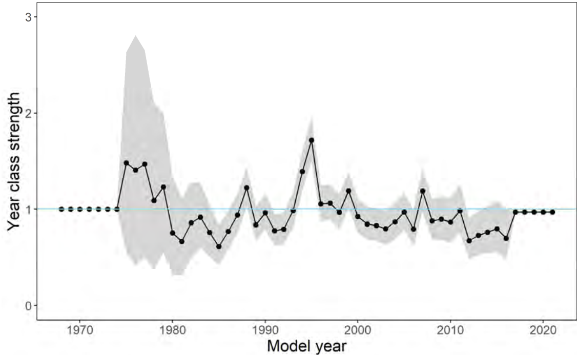
Figure 3: LIN 3&4. Estimated posterior distributions of year class strength from the base case run, with median (line and individual points) and 95% credible interval (grey band). The horizontal line indicates a year class strength of one.
