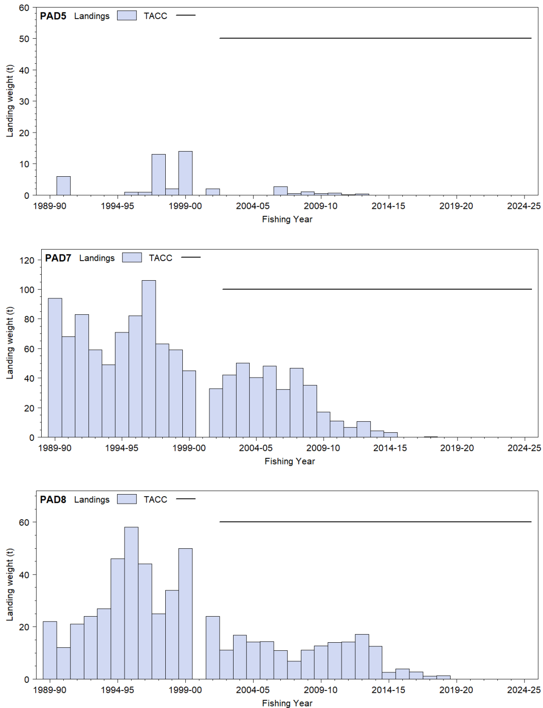
Figure 1 [Continued]: Reported commercial landings and TACCs for the six main PAD stocks: PAD 5 (Southland), PAD 7 (Challenger) and PAD 8 (Central Egmont).
