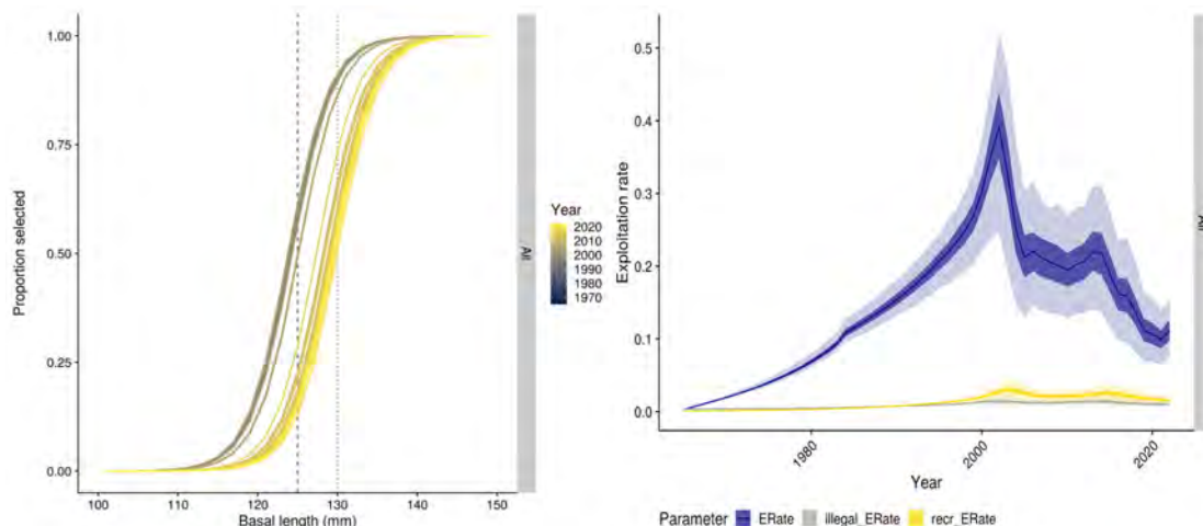
Figure 7: Estimated selectivity by year (left) and exploitation rate (right) for commercial (ERate), illegal (illegal_ERate), and recreational fishery components assumed in the model. Vertical dashed and dotted lines show the minimum legal size and 130 mm as a reference.
