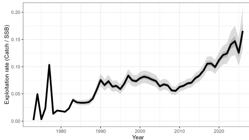
Figure 12: LIN 7WC base model: Exploitation rate (defined as total catch divided by spawning stock biomass) with the interquartile range (dark grey) and 95% credible interval (light grey).
