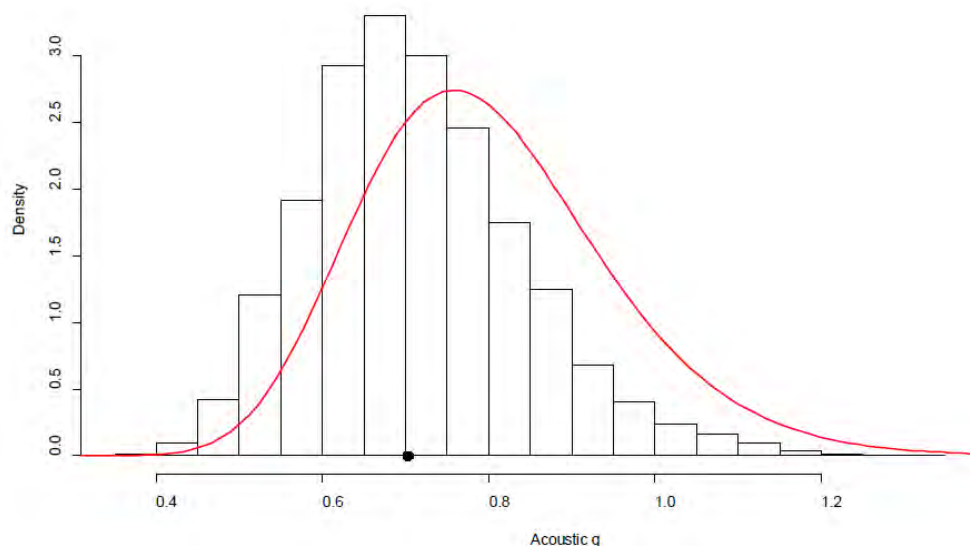
Figure 17: Puysegur base, the marginal posterior distribution of the acoustic q (histogram) compared with its prior (red line). The black dot marks the median of the marginal posterior.
