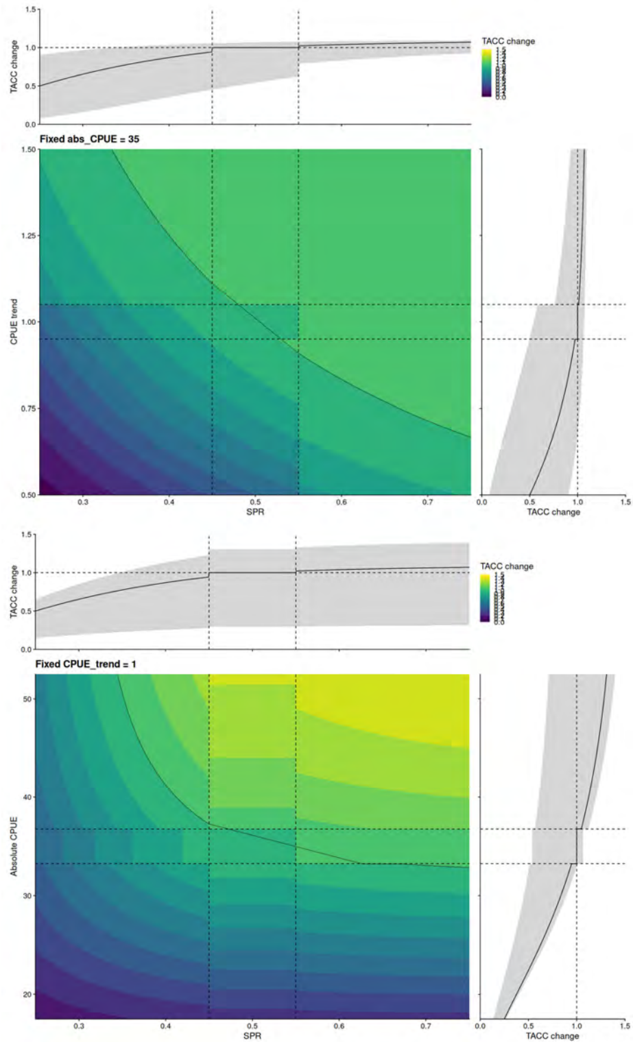
Figure 3: Schematic of the CPUE/LBSPR harvest control rule, illustrating two of the three component signals per panel, illustrating how they combine to determine the TACC multiplier (the multiplier that is applied to the current commercial catch to inform the new TACC).
