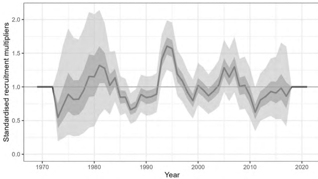
Figure 6: LIN 5&6 and LIN 6B. Estimated posterior distribution of year class strength from the base case run, with median (line and individual points), interquartile range (dark grey band) and 95% credible interval (light grey band). The horizontal line indicates a year class strength of one.
