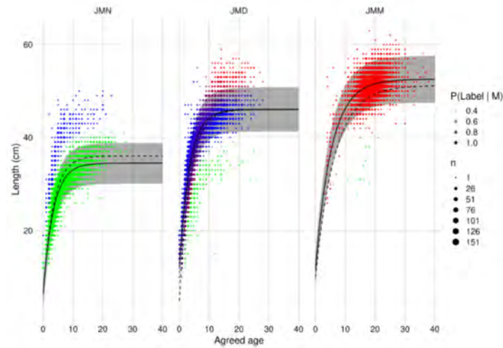
Figure 7: Estimated growth curves for jack mackerels in JMA 7 (JMN, T. novaezelandiae ; JMD, T. declivis ; JMM, T. murphyi ). Solid lines indicate the median and 95% interval for predicted size at age, in comparison to the growth curves based on parameters previously reported in the Plenary (dashed lines). The three panels group the data according to the observer assigned species, and points are coloured by the model predicted species (JMN = green, JMD = blue, JMM = red), and shaded by the estimated probability of that prediction.
