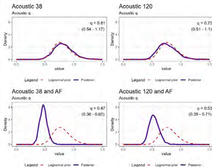
Figure 7: ESCR assessment model prior (broken line) and MCMC posterior (solid line) for the acoustic q (series from 2011) with text giving the median and 95% credible intervals.
