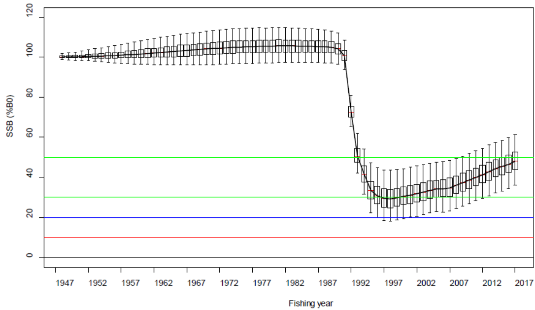
Figure 19: Puysegur base, MCMC estimated spawning stock biomass trajectory. The box in each year covers 50% of the distribution and the whiskers extend to 95% of the distribution. The hard limit (red), soft limit (blue), and biomass target range (green) are marked by horizontal lines.
