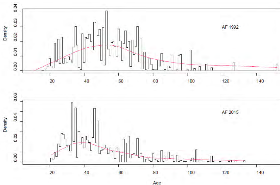
Figure 15: Puysegur age frequency density from 1992 and 2015 used in the base model. The red lines were produced using the lowest smoother in R.
