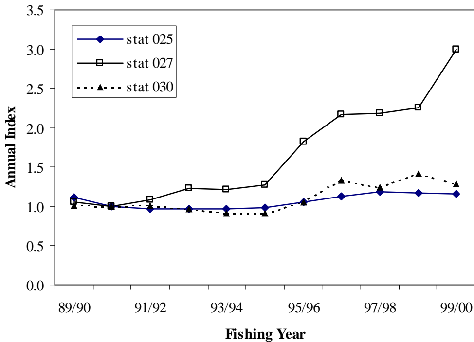
Figure 2: Annual indices for main statistical areas of BCO 5 from individual CPUE models (Langley, 2002).
