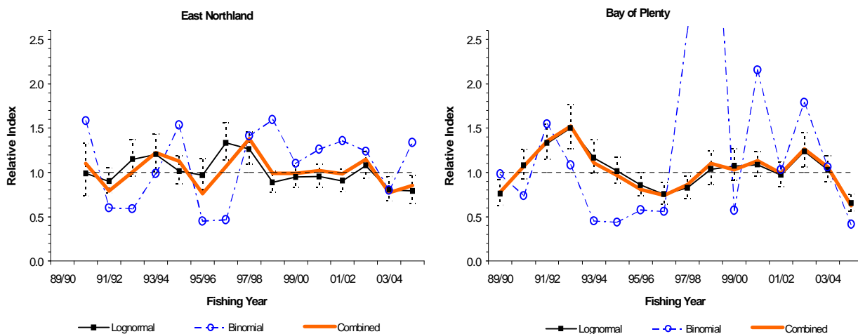
Figure 1. Three standardised CPUE models for the East Northland and Bay of Plenty bottom longline data [Starr et al. 2006a]: a) a lognormal model using non-zero landings as the dependent variable (with associated 95% lognormal error bars); b) a binomial (logistic) model using a binary variable indicating a successful or zero catch of bluenose and c) a combined model which summarises the two sets of indices into a single trajectory
