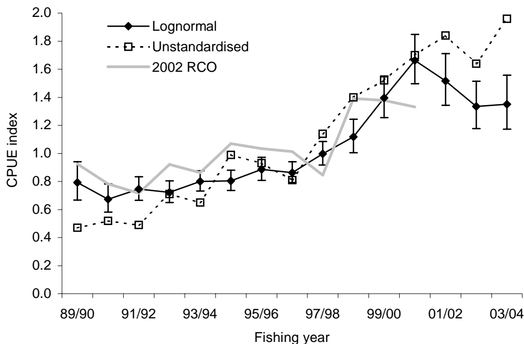
Figure 1: Relative CPUE indices for ELE 3 using the loglinear non-zero model based on the bycatch in the RCO 3 target trawl fishery. Error bars are \pm 2*SE . The equivalent series from the 2002 RCO 3 target fishery is also shown as a thick grey line.
